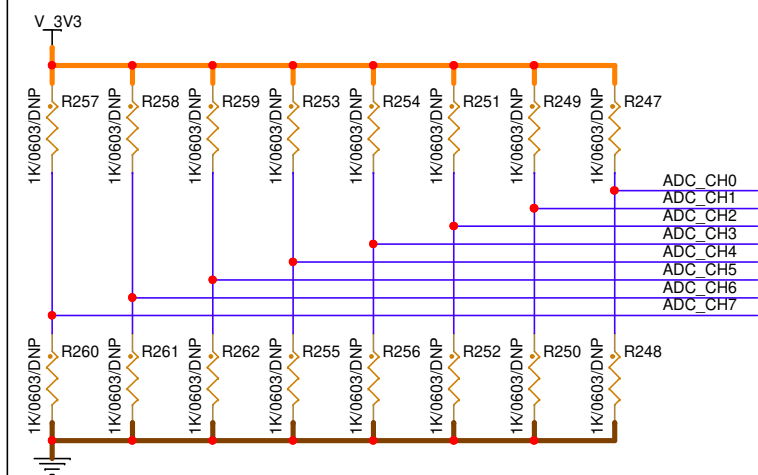
ADC pull-up/pull-down resistors
