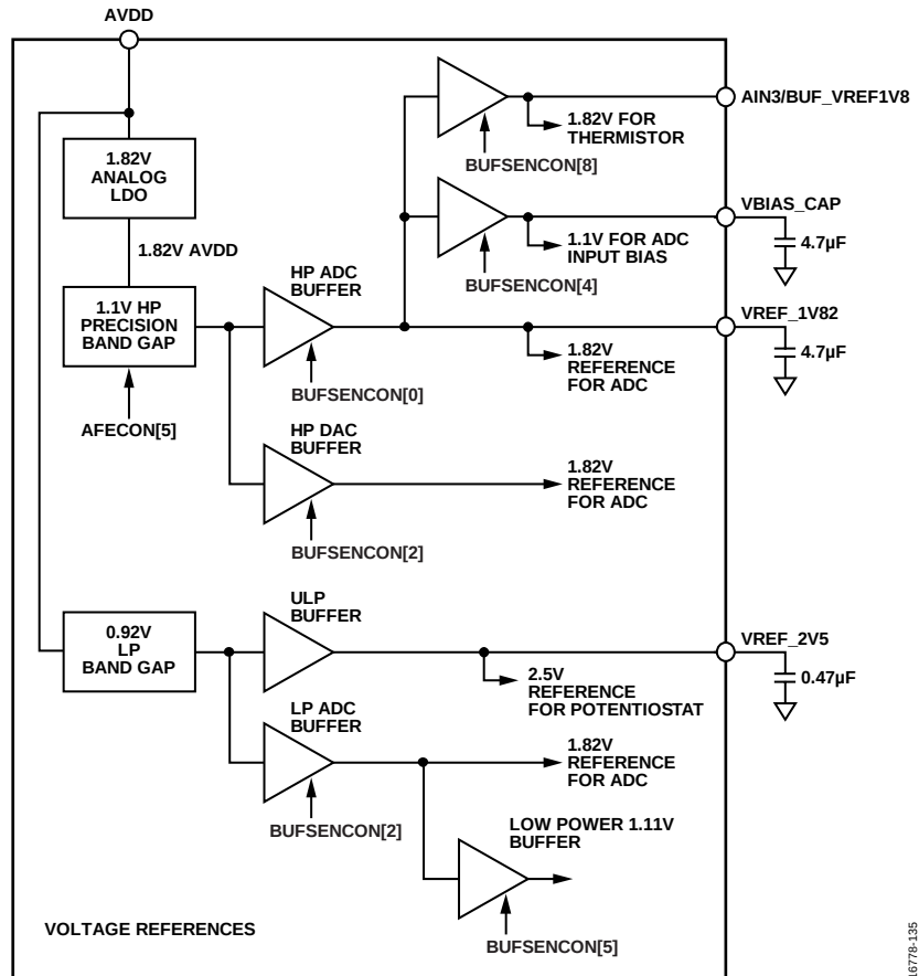
Figure 34. Precision Voltage References
