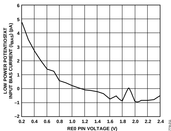
Figure 10. Low Power Potentiostat Input Bias Current ( I_{BIAS} ) vs. REO Pin Voltage
