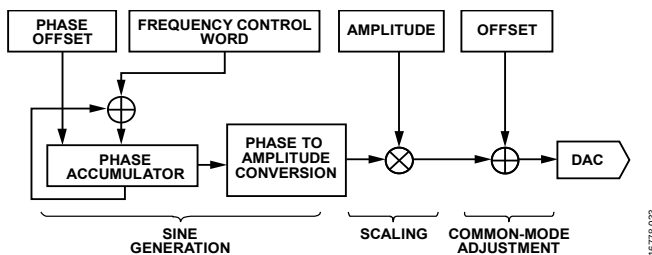
Figure 42. Sinusoid Generator
