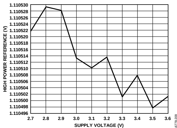
Figure 8. High Power Reference vs. Supply Voltage, 1.11 V Voltage Reference DC PSRR
