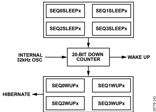
Figure 45. Sleep and Wake-Up Timer Block Diagram
