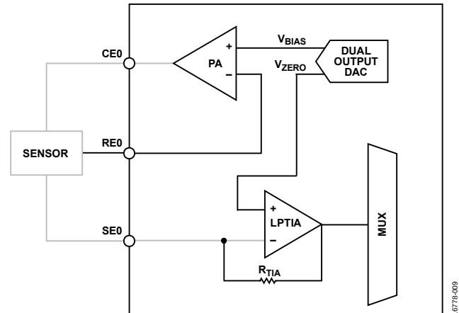
Figure 17. Electrochemical Standard Configuration
