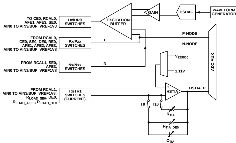
Figure 32. Switch Matrix High Level Diagram
