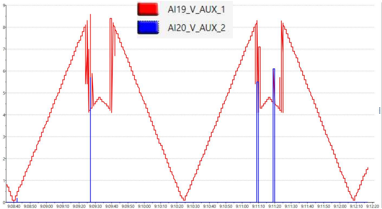
Sweep 0-10V on ADC1, ADC2 floating (depending on LSB value, fail migrate to ADC2?)
