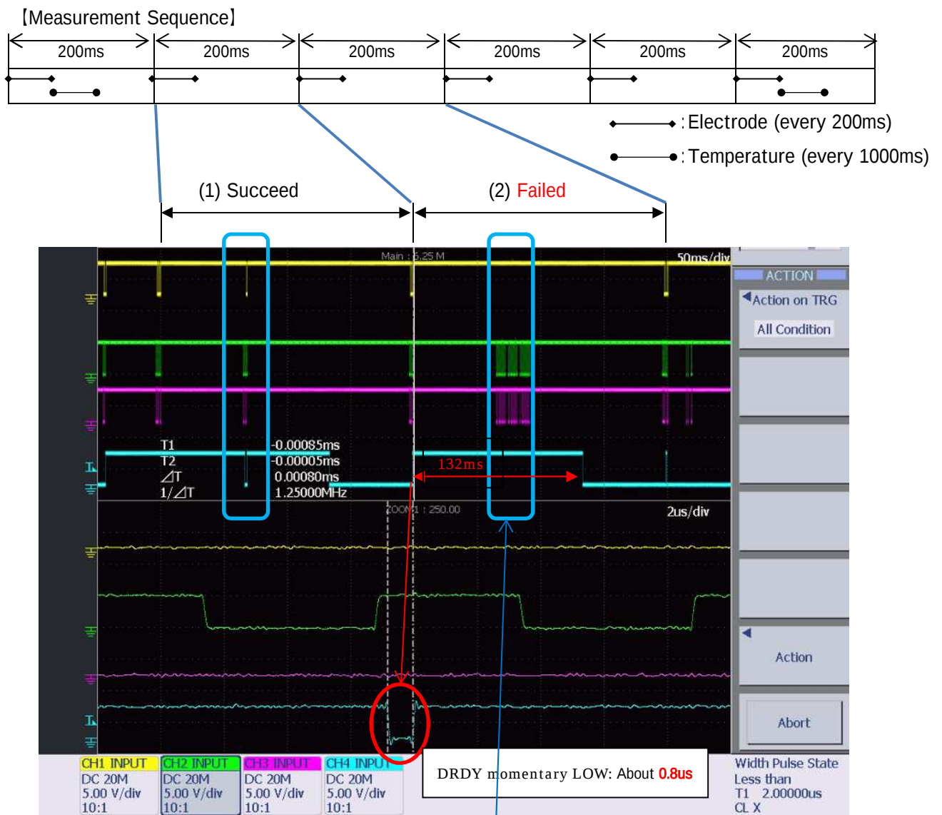
Figure.8 Whole waveform when error occurred (Yellow:CS Green:CLK Pink:DIN Blue:DRDY)
