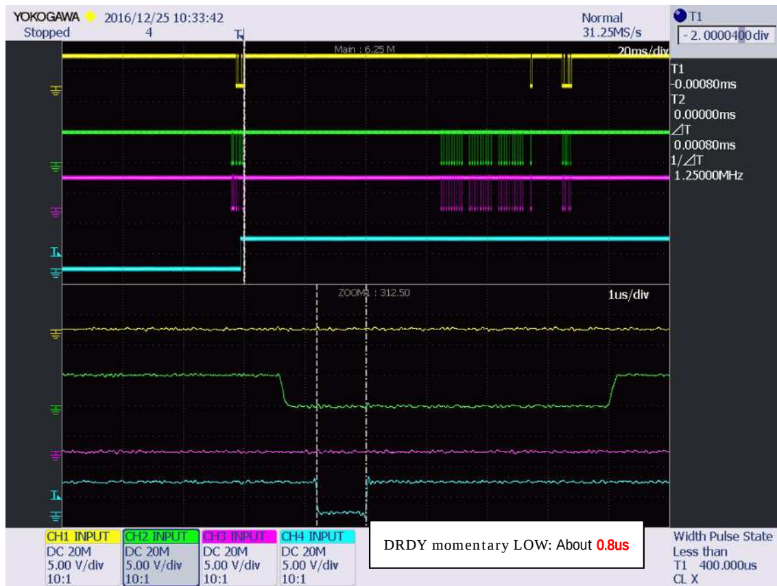
Figure.7 Zoomed momentary DRDY Low (Yellow:CS Green:CLK Pink:DIN Blue:DRDY)
