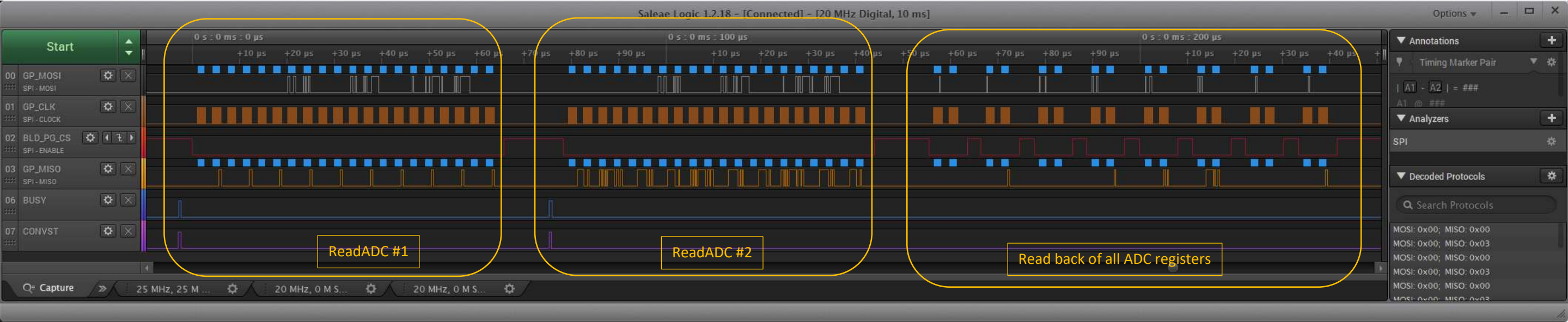
A sequence of CONVST and reading the ADC results twice followed by reading the ADC registers
