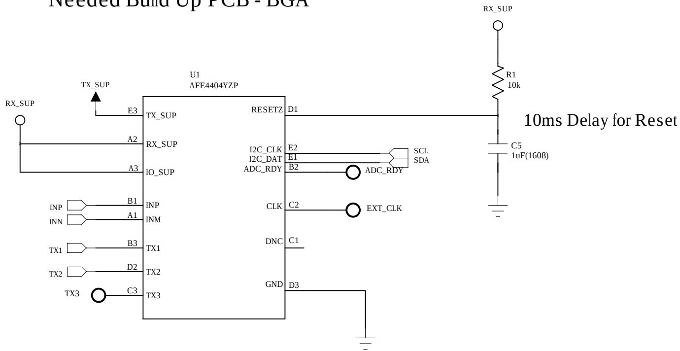
Needed Build Up PCB - BGA
