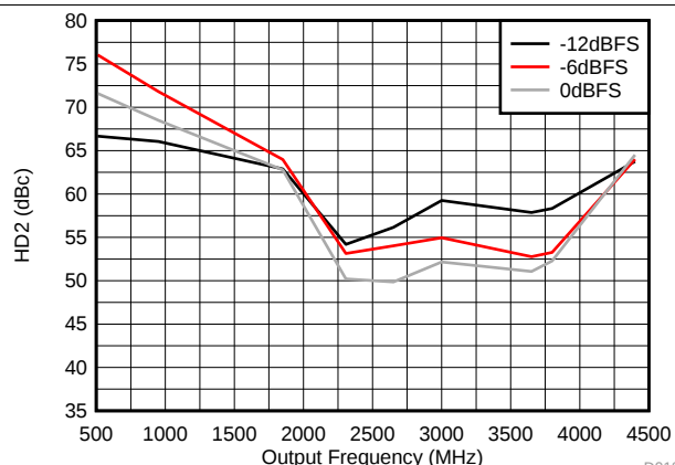
D018 DAC38RF80/90/84
