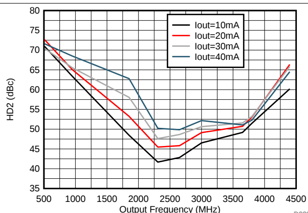
D028 DAC38RF80/90/84
