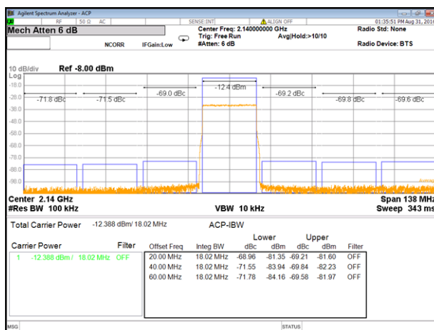
Figure 171. Dual band ACPR Performance in Downlink Band 1 with On-chip PLL
