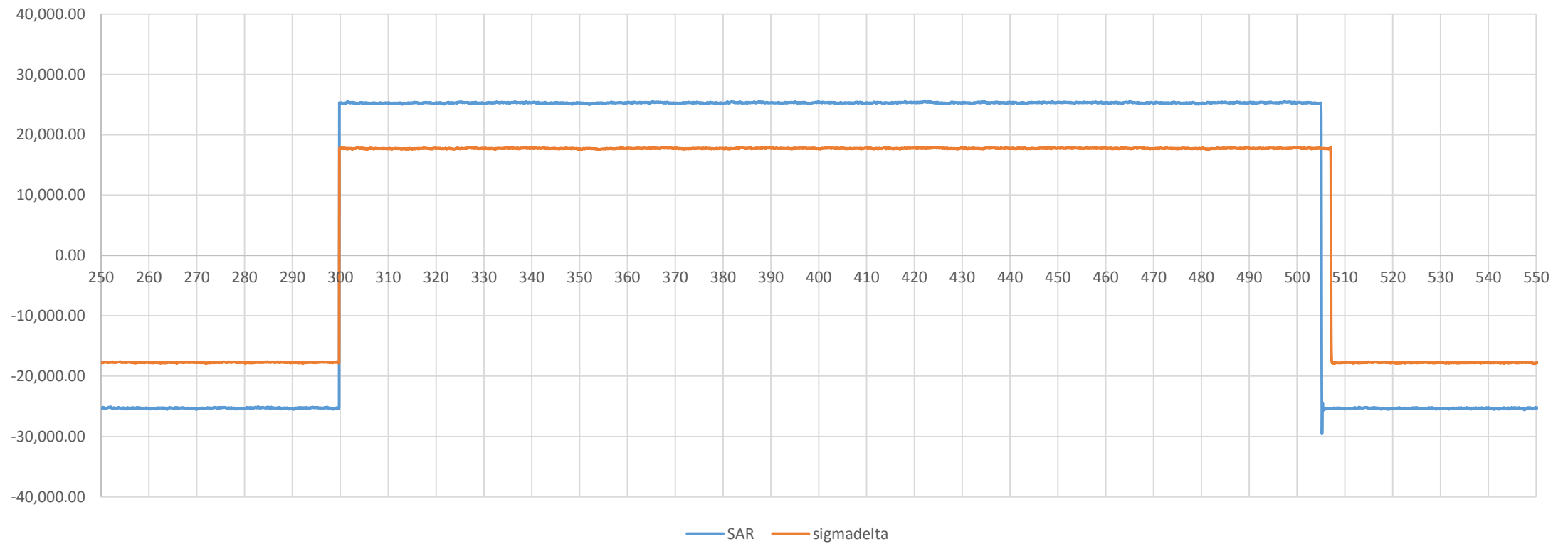
Pulse_testing_250mSpulse width
