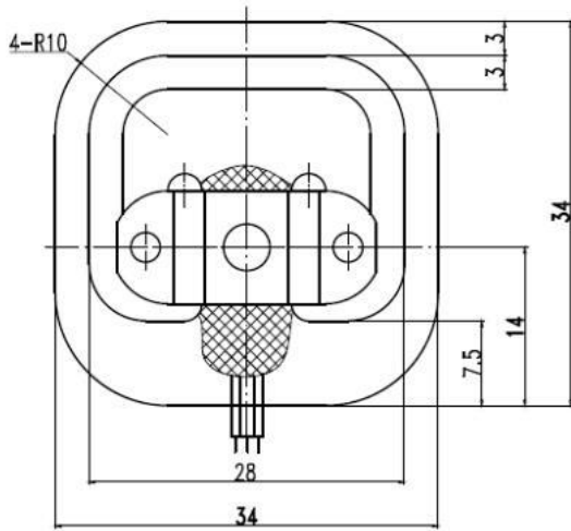
Electrical connection and Dimensions:(dimension unit: mm)
