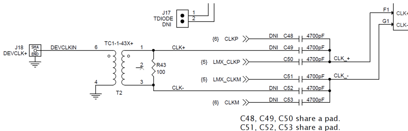
Figure B-3. External DevCLK EVM Configuration
