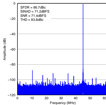
Figure 29. FFT for 170-MHz Input Signal
