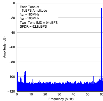
Figure 31. FFT for Two-Tone Input Signal
