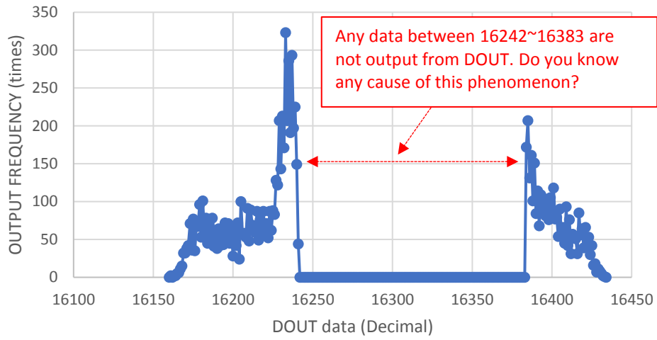
OUTPUT FREQUENCY vs ADS8326 DOUT data
