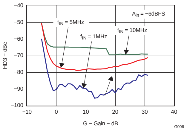
Figure 13. HD3 Across Coarse Gain and Three f_{IN} (–6dBFS) (2)
