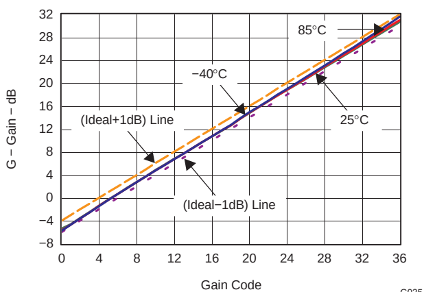
Figure 5. Gain vs Gain Code and Temperature
