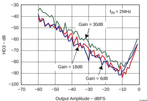
Figure 15. HD3 vs Output Amplitude
