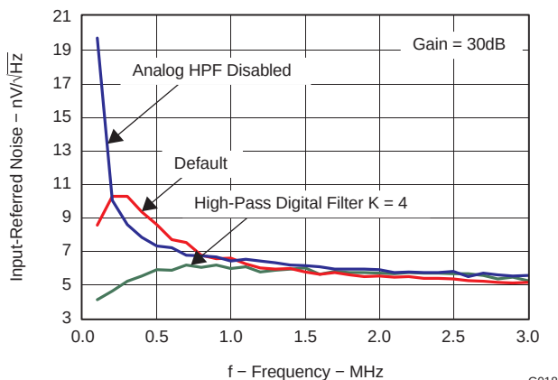
Figure 28. Input-Referred Noise vs Frequency
