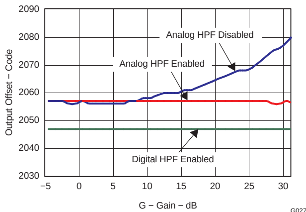
Figure 17. Output Offset vs Gain
