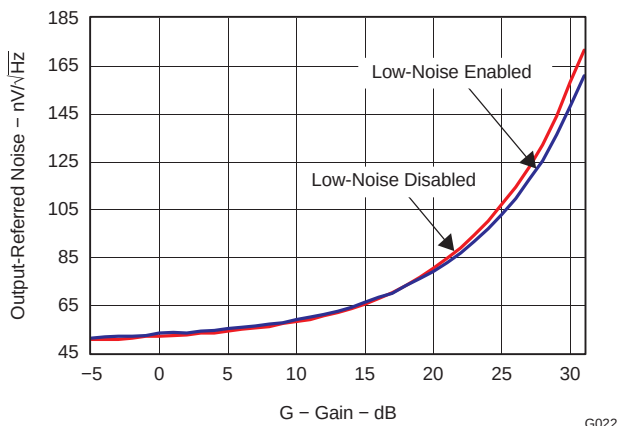
Figure 7. Output-Referred Noise vs Gain
