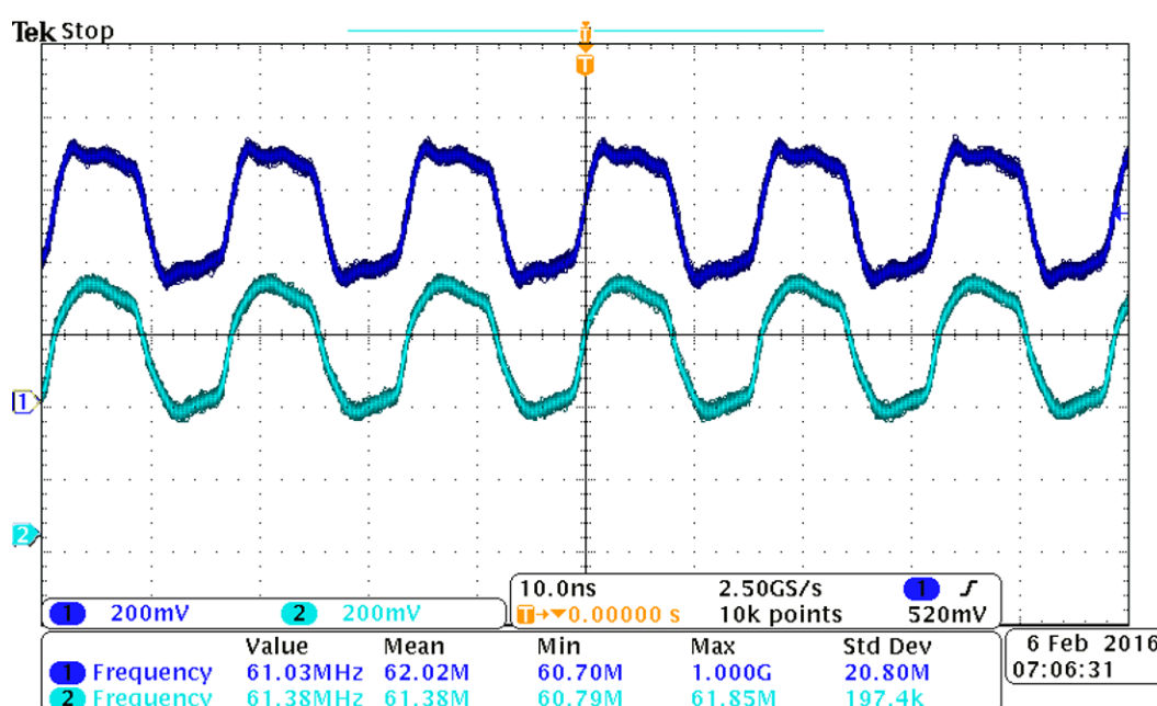
Figure 26. SYSREF Signal Probed at Two Different DAC3xJ8x EVM With LMK04828 in Nested 0-Delay Dual Loop Mode
