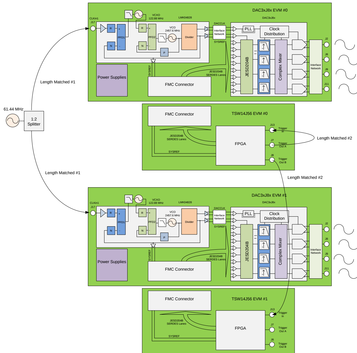
Figure 7. Overall Measurement Setup
