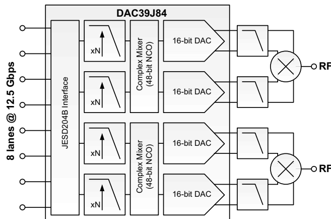
Figure 1. Typical Application Environment of DAC3xJ8x
