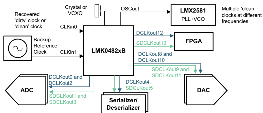
Figure 2. LMK0482xB Simplified Schematic
