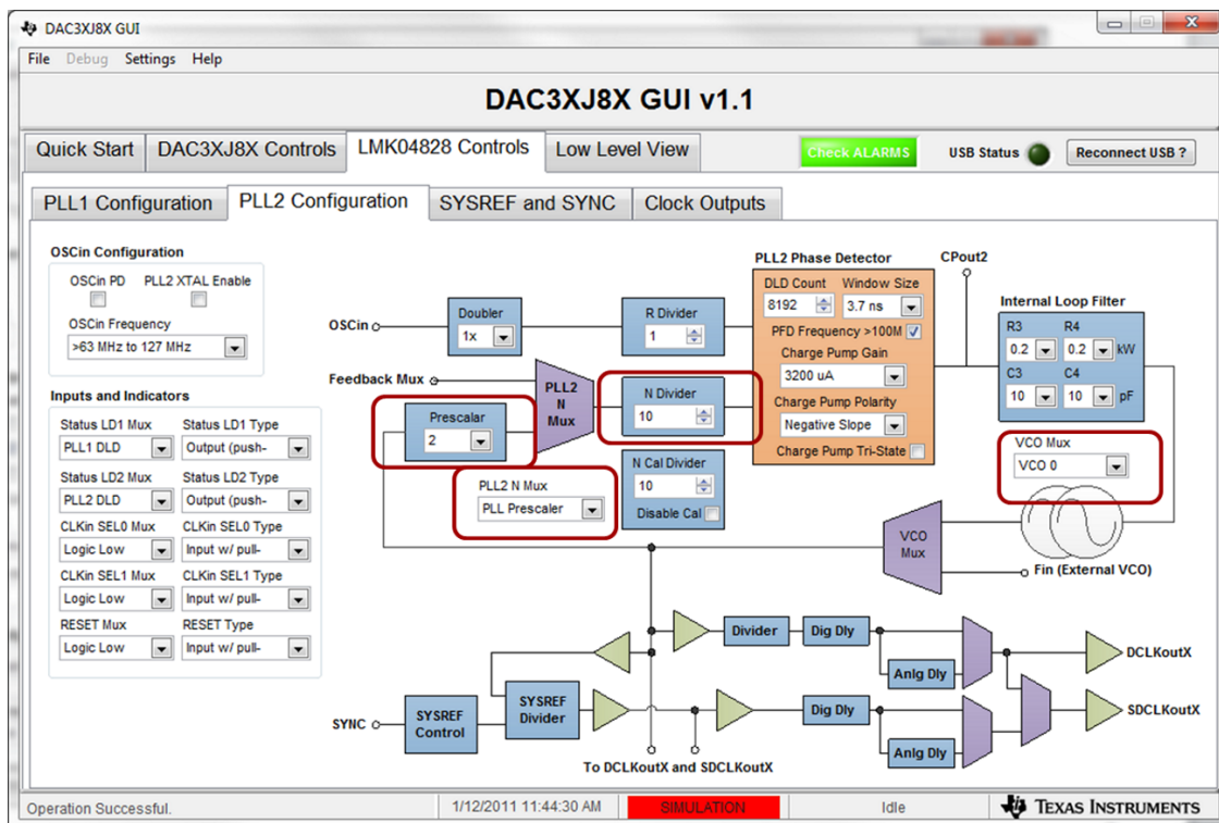
Figure 17. PLL2 Settings
