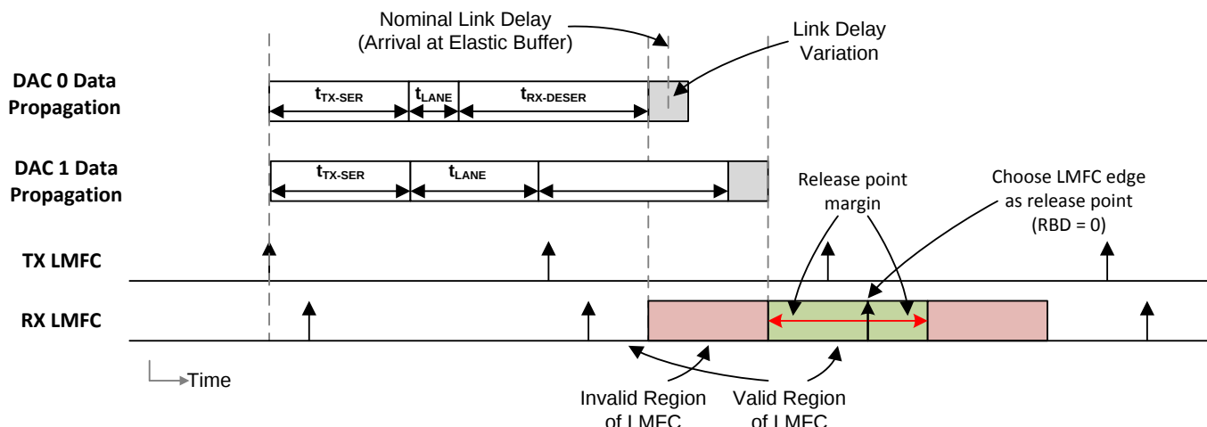
Figure 6. RBD Selection for the DAC3xJ8x JESD204B RX Link
