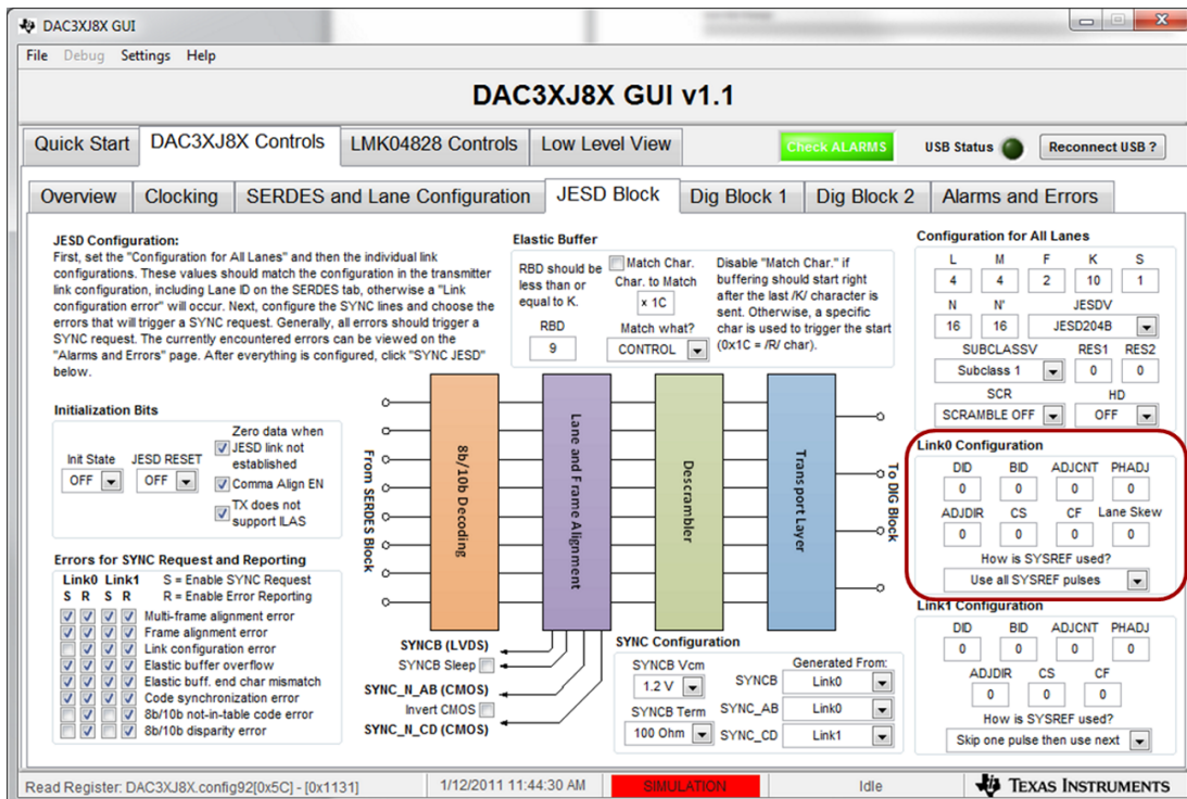
Figure 15. DAC3xJ8x GUI—Setting Link0 SYSREF Option
