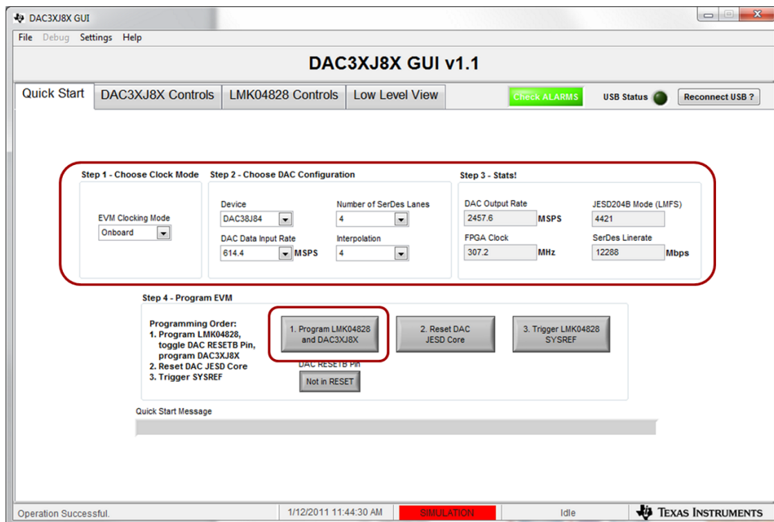
Figure 13. DAC3xJ8x GUI—Quick Start Menu
