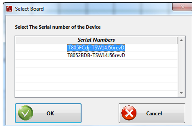
Figure 24. Select TSW14J56 EVM0 Master Board
