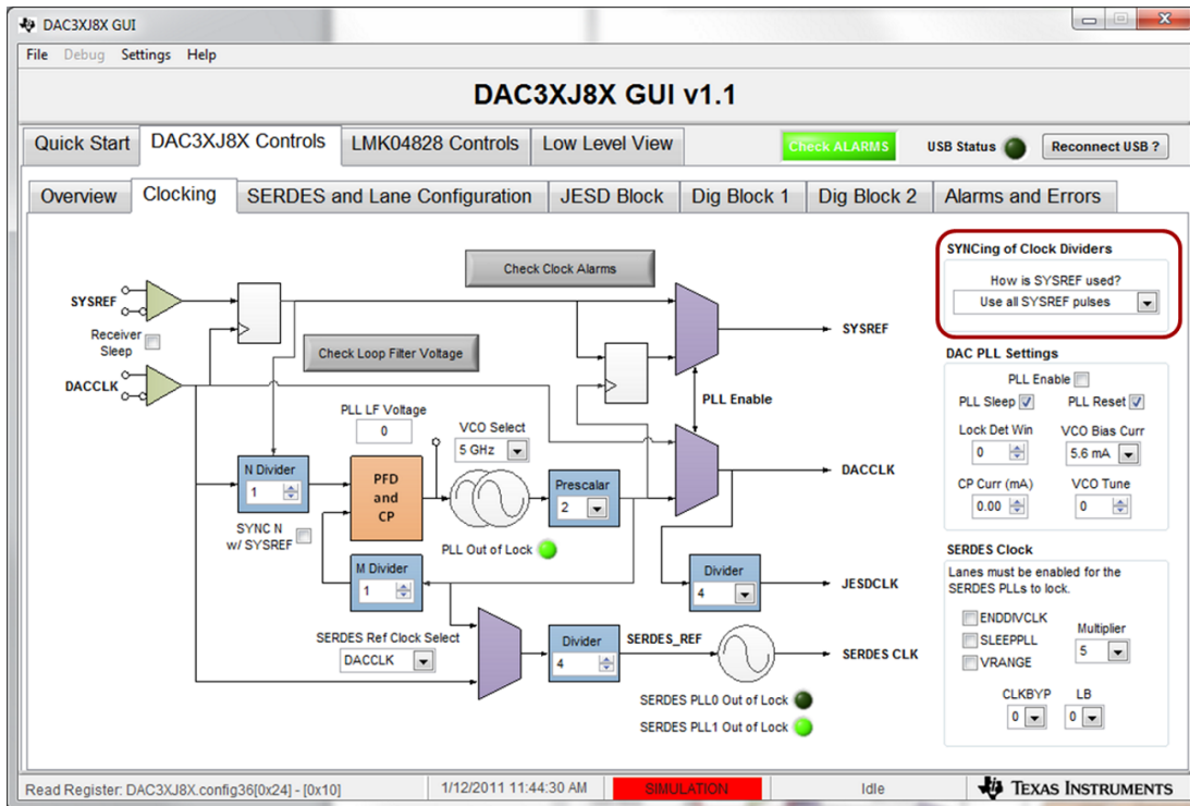
Figure 14. DAC3xJ8x GUI—Setting Clock Divider
