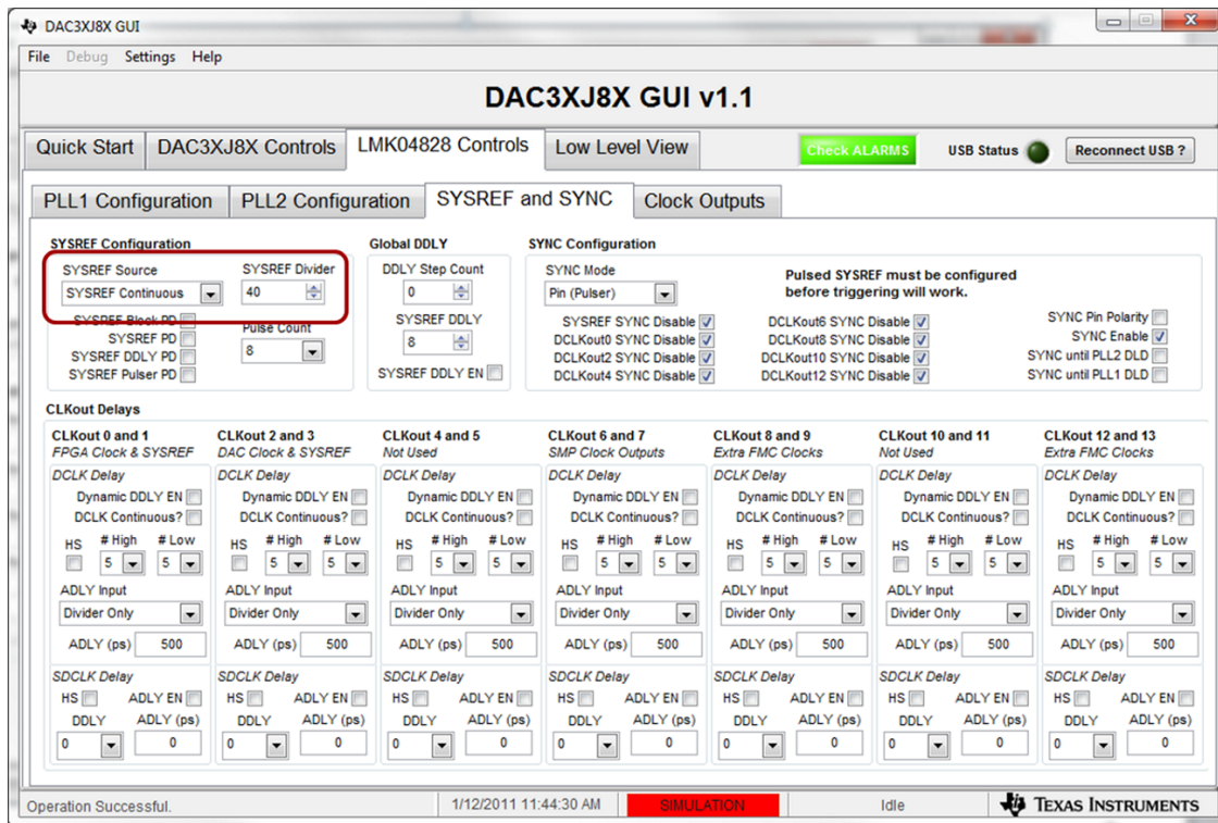
Figure 18. SYSREF Setting
