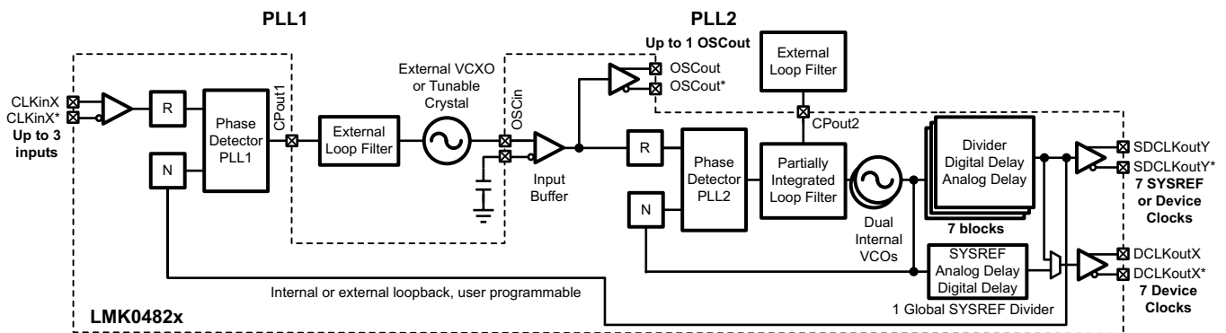
Figure 8. Simplified Functional Block Diagram for Nested 0-delay Dual Loop Mode (From LMK04828 Datasheet)
