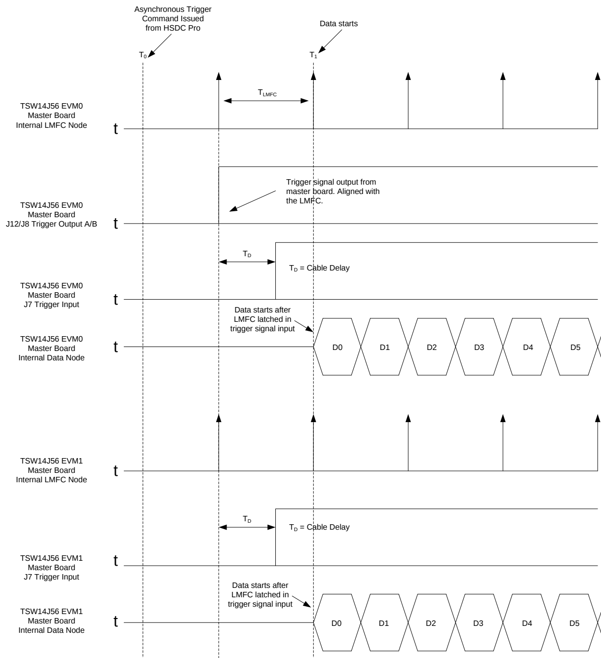
Figure 12. TSW14J56 EVM Sample Alignment in Trigger Mode
