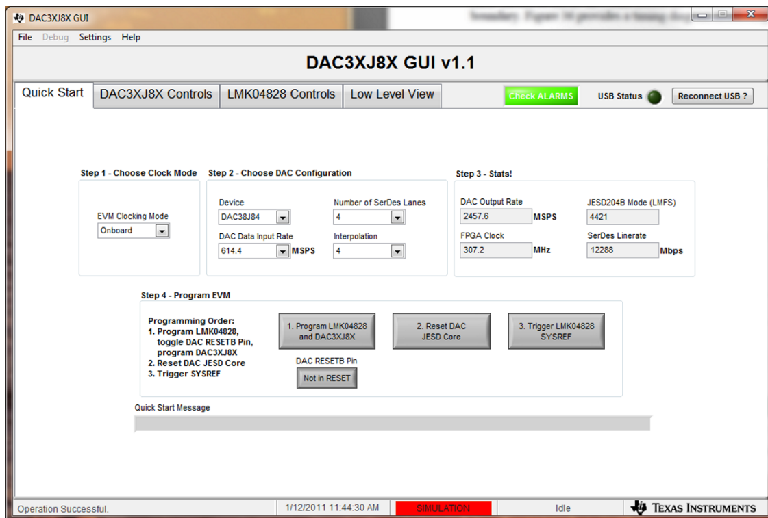
Figure 9. DAC38J84 Setting
