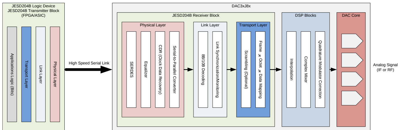
Figure 4. DAC3xJ8x JESD204B Receiver Block and Overall JESD204B Environment
