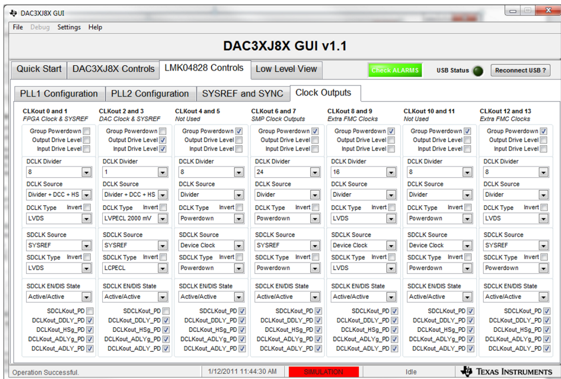
Figure 19. DCLK and SDCLK Setting
