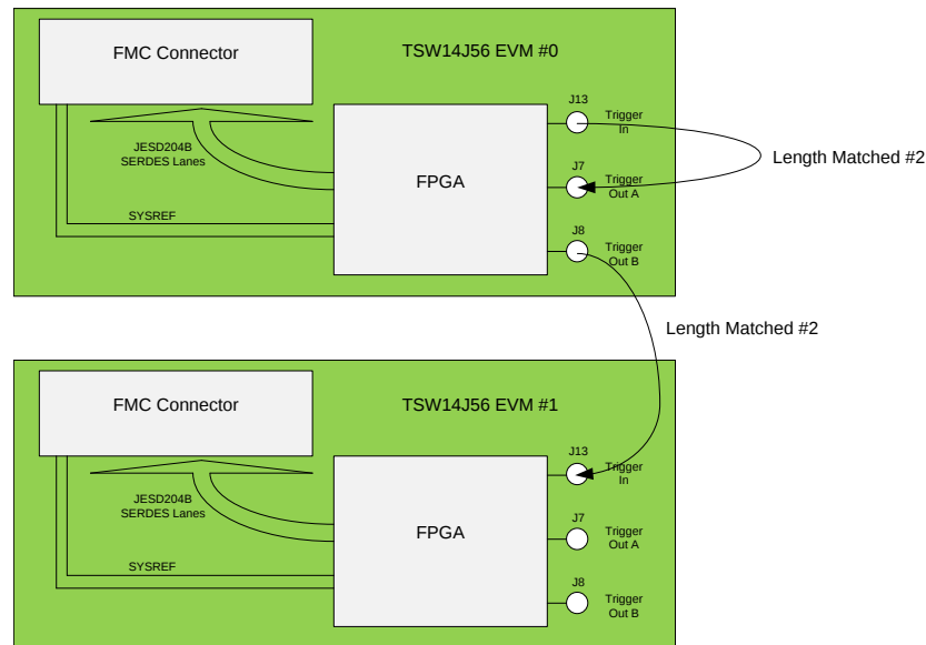
Figure 11. TSW14J56 EVM Master and Slave Trigger Setup
