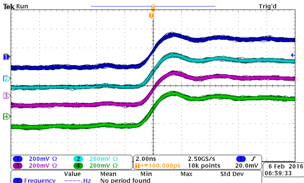
Figure 27. DAC3xJ8x Channel A and Channel B Outputs at Two Different DAC3xJ8x EVMs
