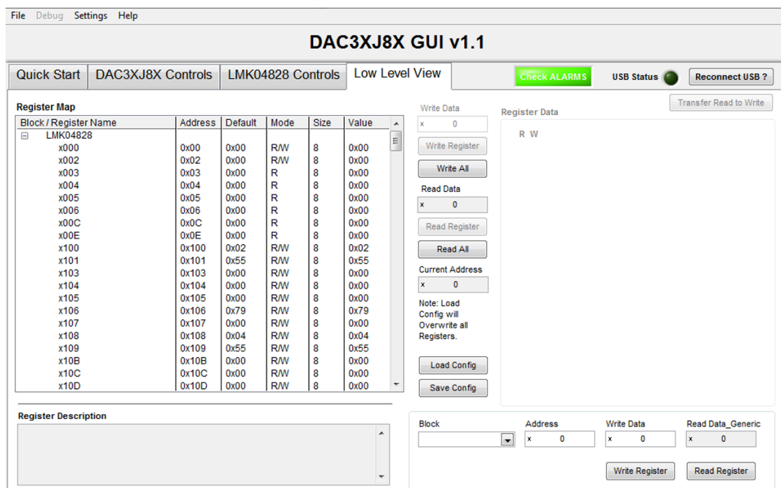
Figure 20. DAC3xJ8x EVM GUI—Low Level View
