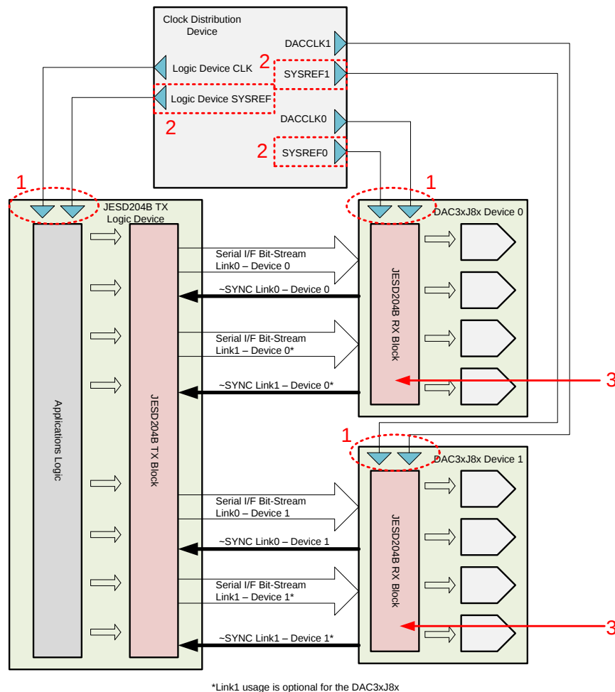
Figure 5. Typical Setup for Multiple JESD204B Links for DAC3xJ8x Devices
