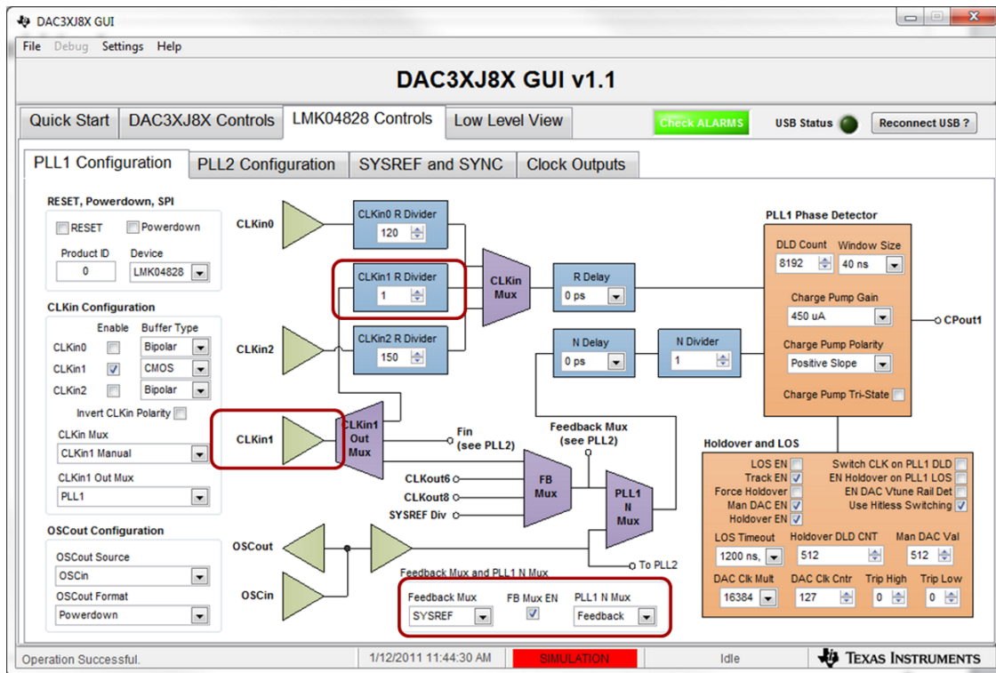
Figure 16. PLL1 Settings
