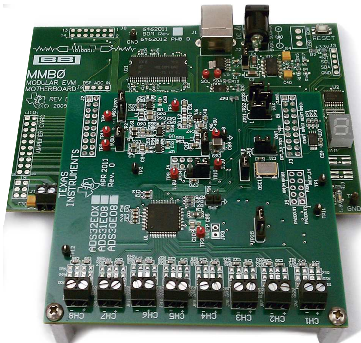
Figure 2. ADS131E08EVM-PDK Kit
