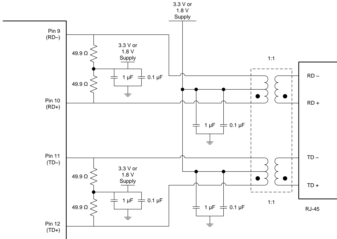
Figure 33. TPI Network Circuit
