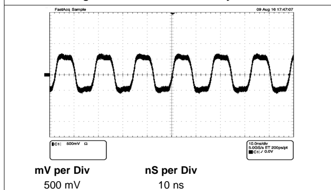
Figure 19. 100BASE-FX Waveform
