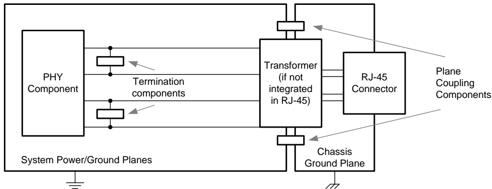
Figure 40. Layout Example
