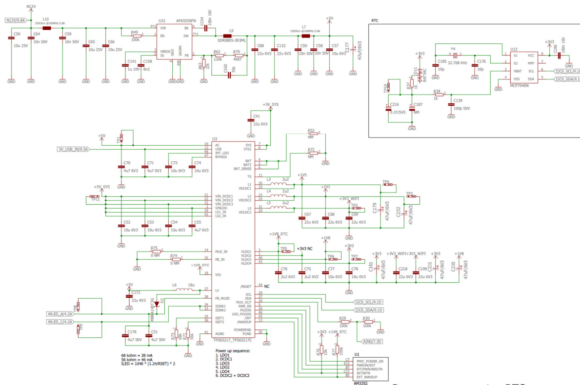
Power management + RTC
