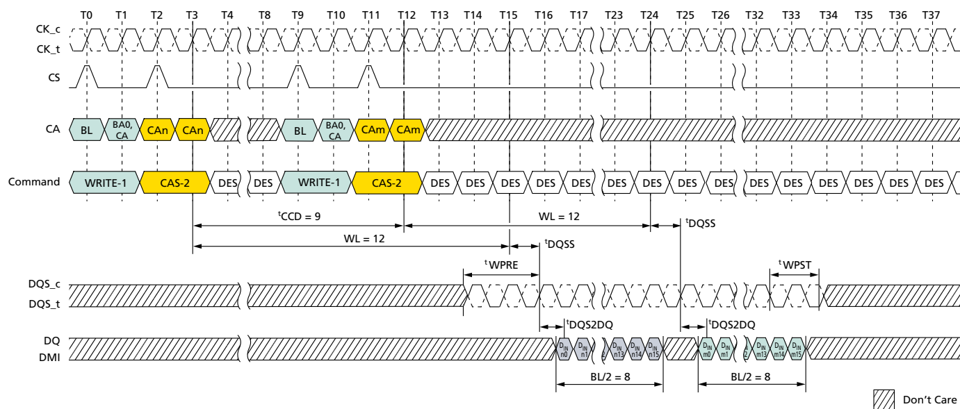
Figure 58: Consecutive WRITE: t_{CCD} = \text{MIN} + 1, 1.5n\text{CK} Postamble
