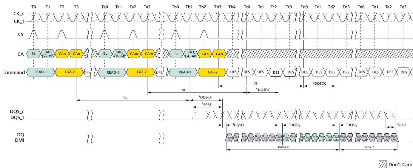
Figure 22: Seamless Burst Read
