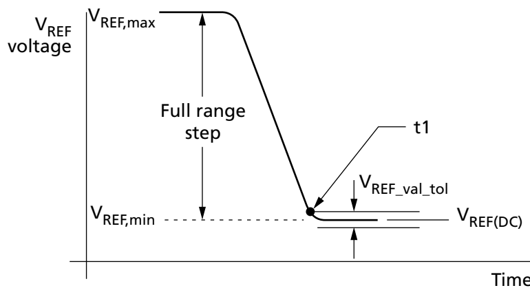
Figure 106: V_{REF(CA)} Full Step from V_{REF,max} to V_{REF,min}
