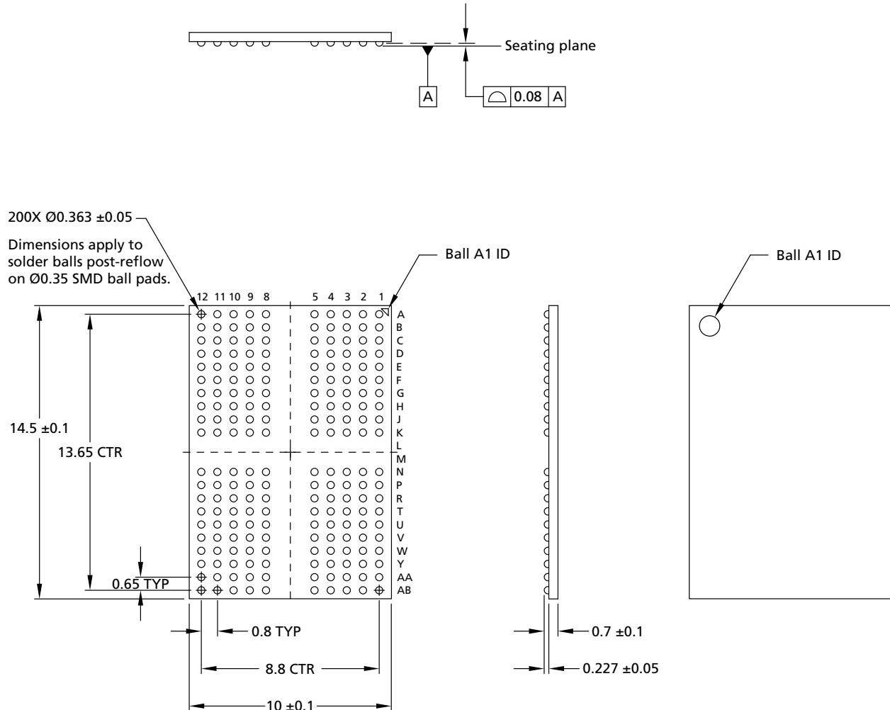
Figure 6: 200-Ball WFBGA – 10mm x 14.5mm (Package Code: DS)
