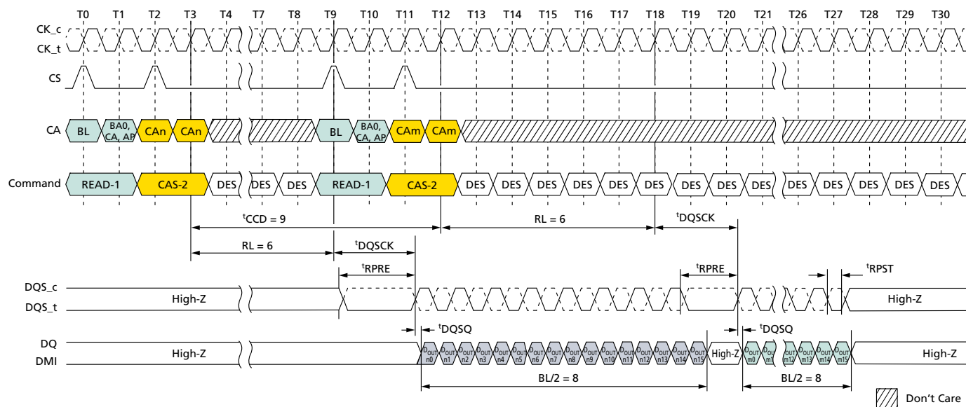
Figure 45: Consecutive READ: t_{CCD} = \text{MIN} + 1 , Preamble = Static, 0.5n\text{CK} Postamble
