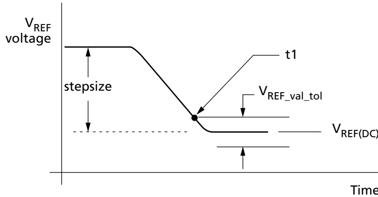
Figure 105: V_{REF(CA)} Full Step from V_{REF,min} to V_{REF,max}
