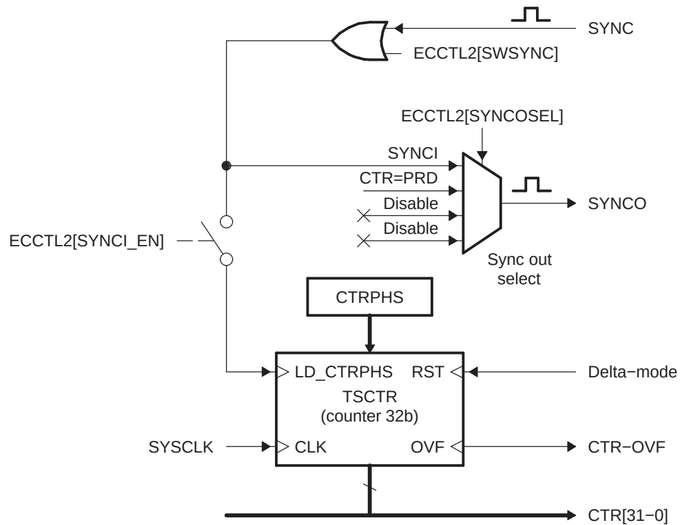
Figure 14-7. Counter and Synchronization Block Diagram
