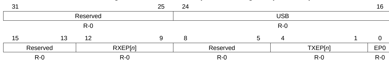
Figure 33-35. USB Interrupt Source Register (INTSRCR)
