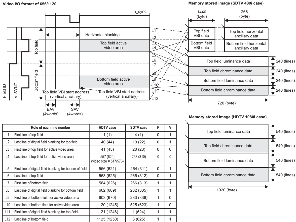
Figure 34-4. Interlaced Video
