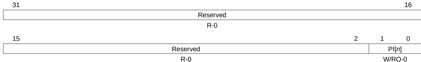
Figure 27-6. Ports Implemented Register (PI)
