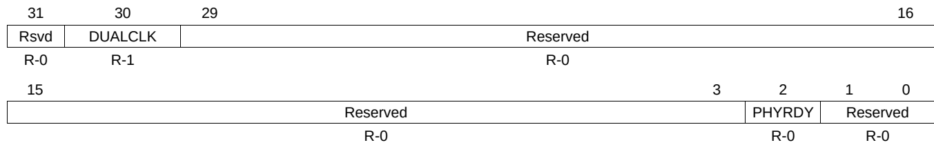
Figure 13-21. SDRAM Status Register (SDRSTAT)
