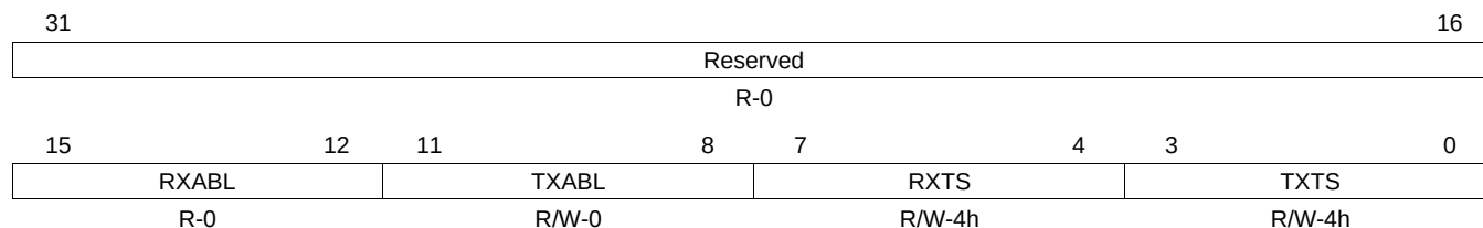
Figure 27-35. Port DMA Control Register (P0DMACR)
