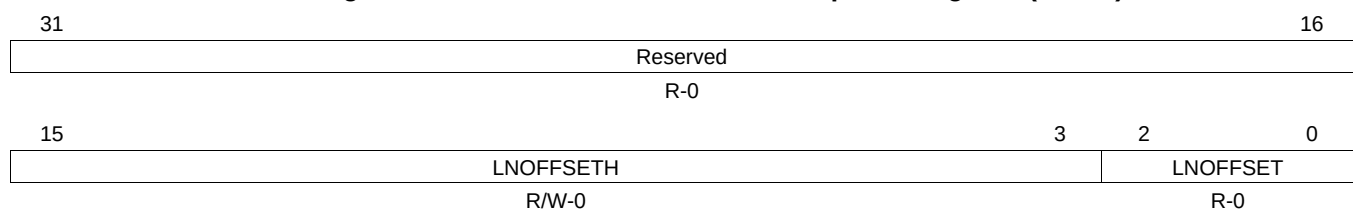
Figure 31-30. uPP DMA Channel I Descriptor 2 Register (UPID2)
