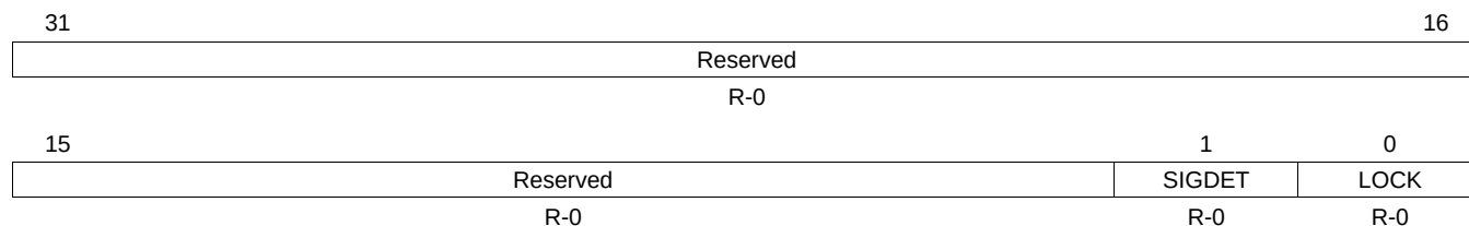
Figure 27-37. Port PHY Status Register (P0PHYSR)
