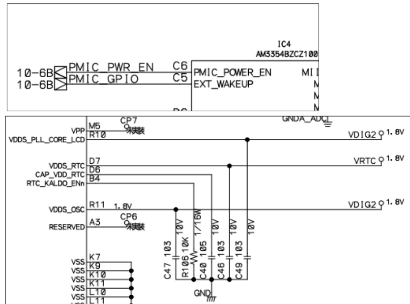
AM3354 RTC block schematic
