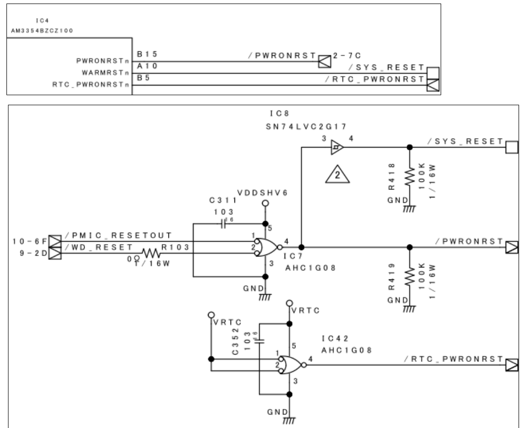
AM3354 RESET block schematic
