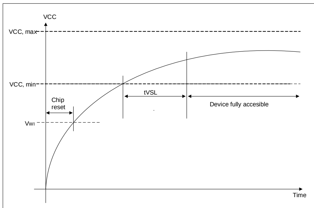
Figure 8.26 Power-Up Timing
