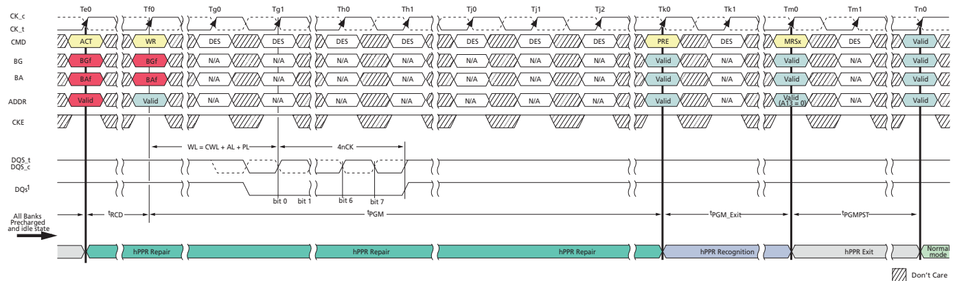
Figure 79: hPPR WR – Repair and Exit
