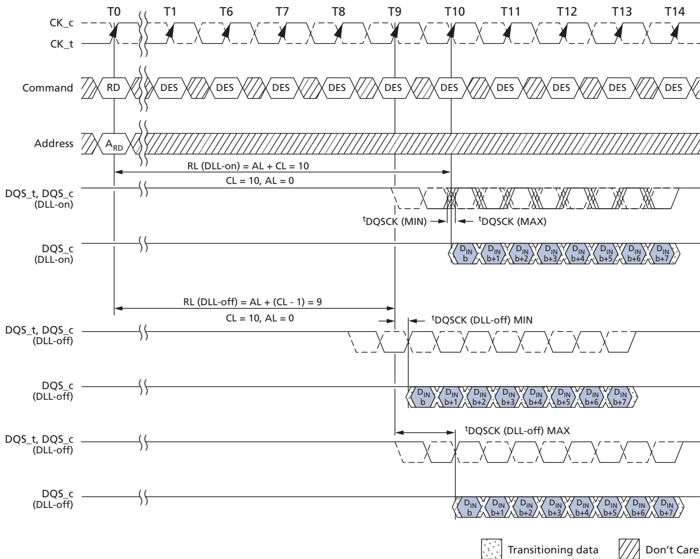
Figure 20: DLL-Off Mode Read Timing Operation
