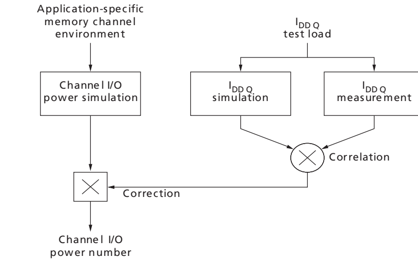
Figure 247: Correlation: Simulated Channel I/O Power to Actual Channel I/O Power
