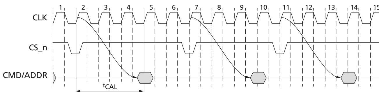
Figure 27: CAL Timing Definition
