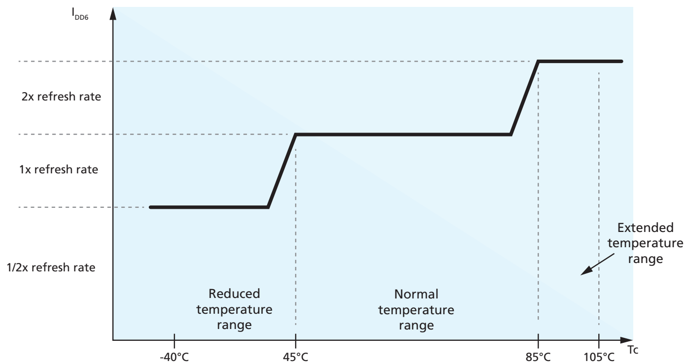
Figure 35: Auto Self Refresh Ranges
