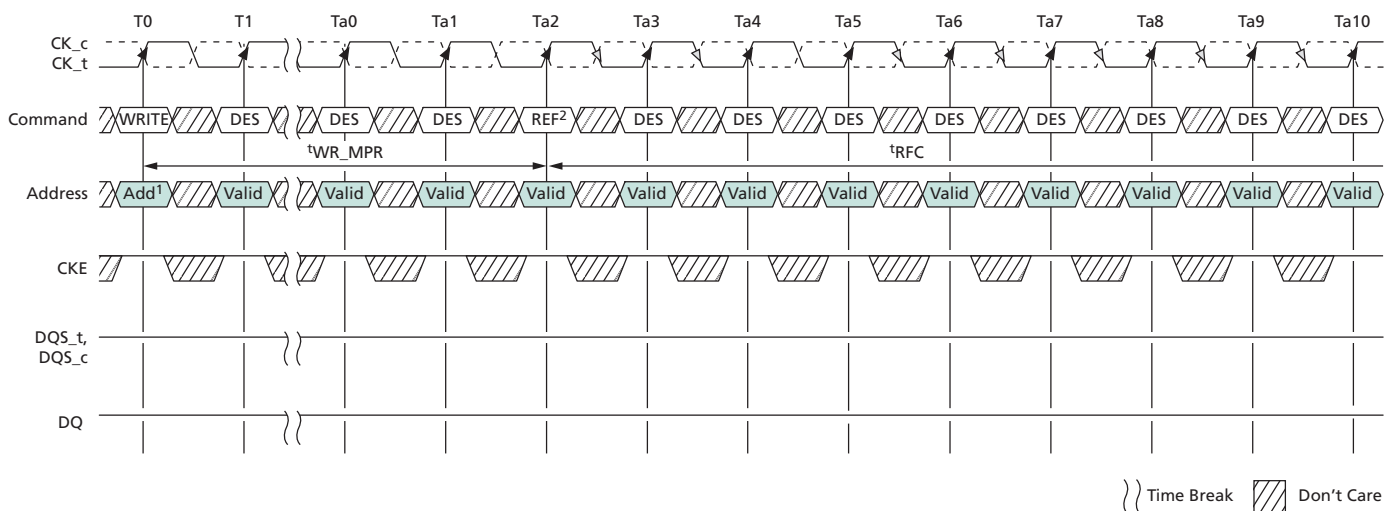
Figure 44: WRITE-to-REFRESH Timing
