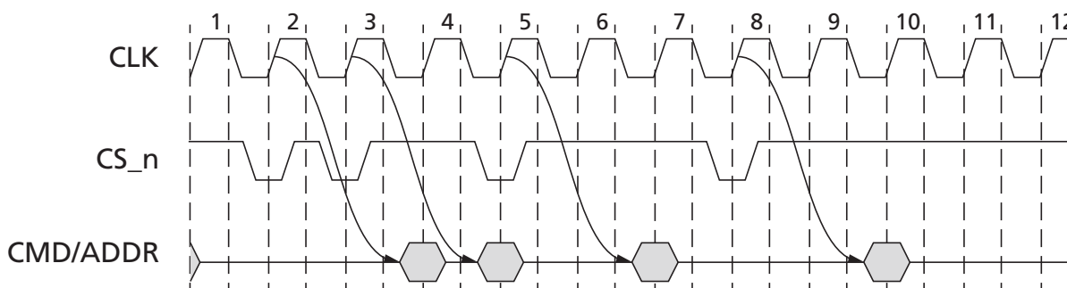
Figure 28: CAL Timing Example (Consecutive \text{CS}_n = LOW)
