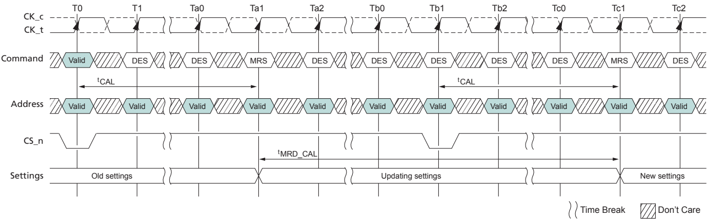
Figure 32: t_{MRD\_CAL} , Mode Register Cycle Time With CAL Enabled
