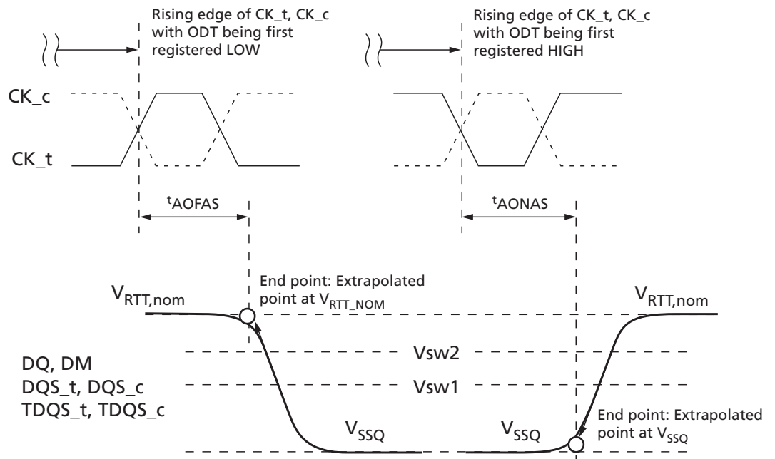
Figure 244: t_{\text{AOFAS}} and t_{\text{AONAS}} Definitions
