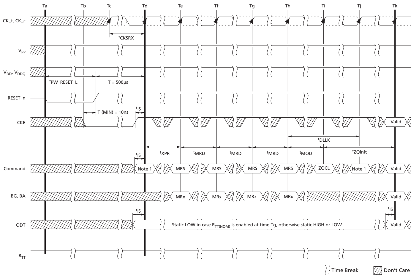
Figure 16: RESET and Initialization Sequence at Power-On Ramping
