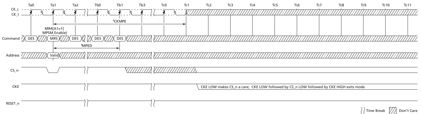
Figure 48: Maximum Power-Saving Mode Entry
