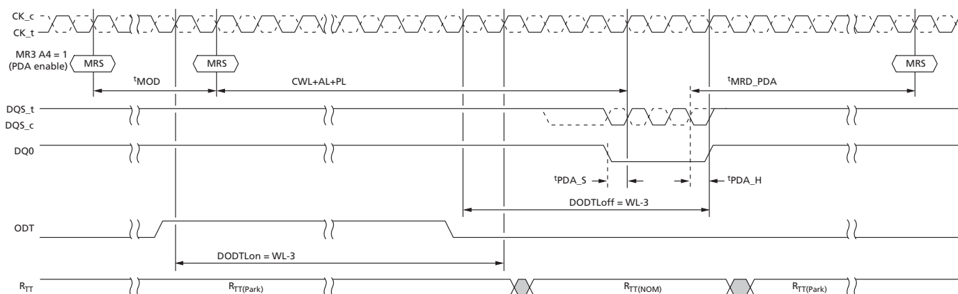
Figure 64: PDA Operation Enabled, BC4
