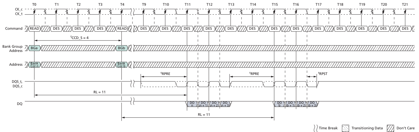
Figure 138: READ (BC4) to READ (BC4) with 2 nd CK Preamble in Different Bank Group
