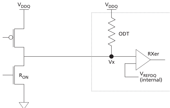
Figure 74: V_{\text{REFDQ}} Equivalent Circuit
