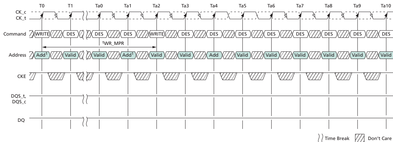
Figure 41: MPR Back-to-Back WRITE Timing
