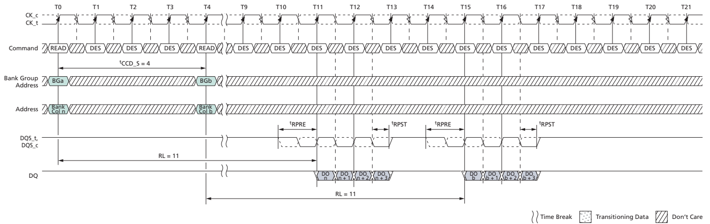
Figure 137: READ (BC4) to READ (BC4) with 1 st CK Preamble in Different Bank Group
