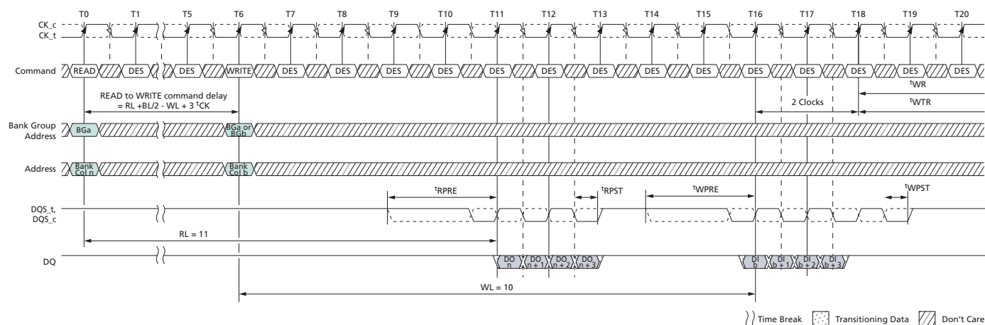
Figure 148: READ (BC4) Fixed to WRITE (BC4) Fixed with 2^t\text{CK} Preamble in Same or Different Bank Group
