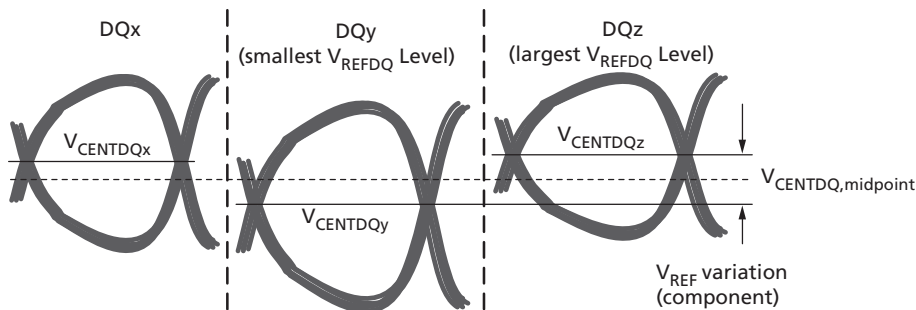
Figure 169: V_{\text{CENT\_DQ}} V_{\text{REFDQ}} Voltage Variation
