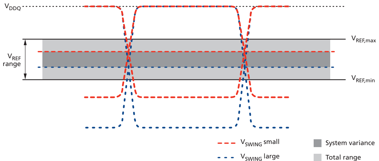
Figure 66: V_{\text{REFDQ}} Voltage Range
