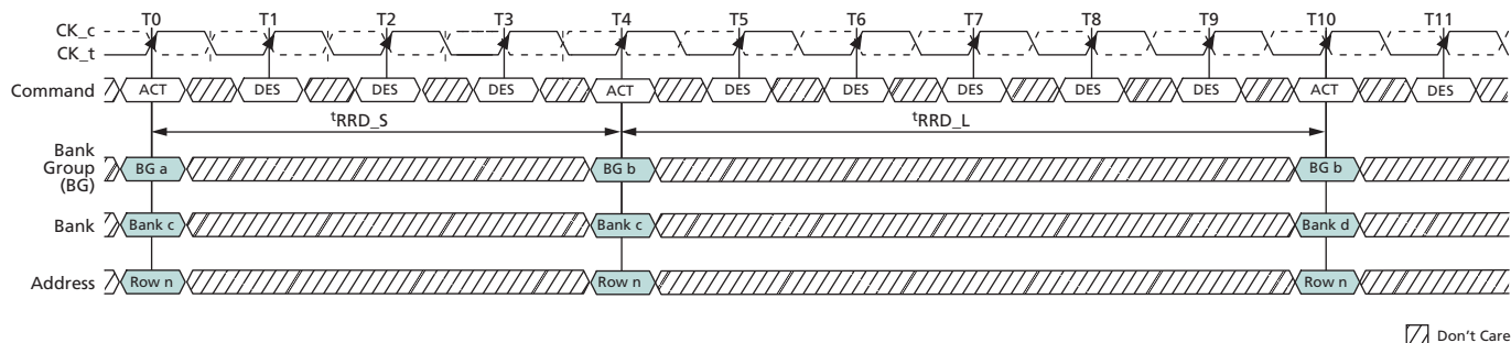
Figure 82: t_{RRD} Timing
