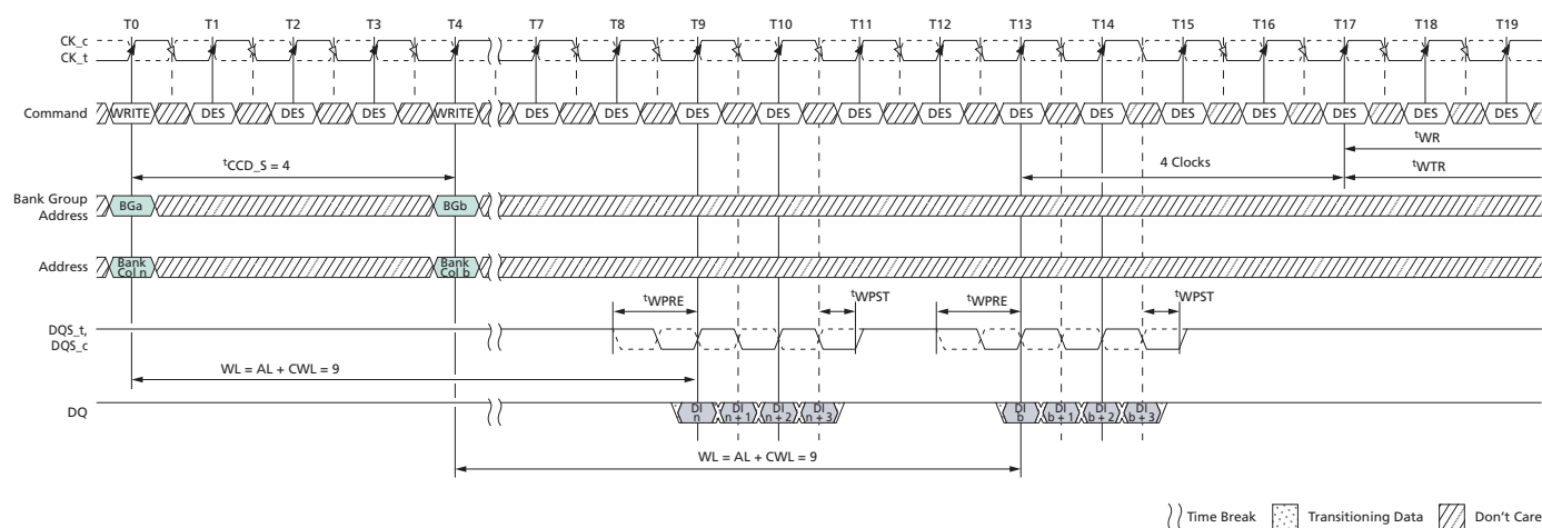
Figure 179: WRITE (BC4) OTF to WRITE (BC4) OTF with 1^tCK Preamble in Different Bank Group
