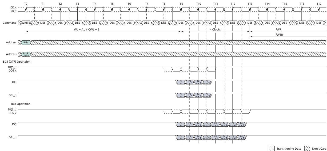
Figure 194: WRITE (BL8/BC4-OTF) with 1 t CK Preamble and DBI
