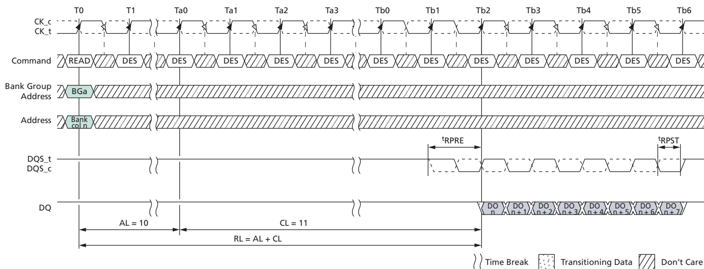
Figure 132: READ Burst Operation, RL = 21 (AL = 10, CL = 11, BL8)
