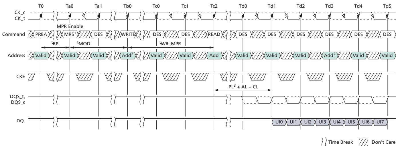
Figure 40: MPR WRITE and WRITE-to-READ Timing
