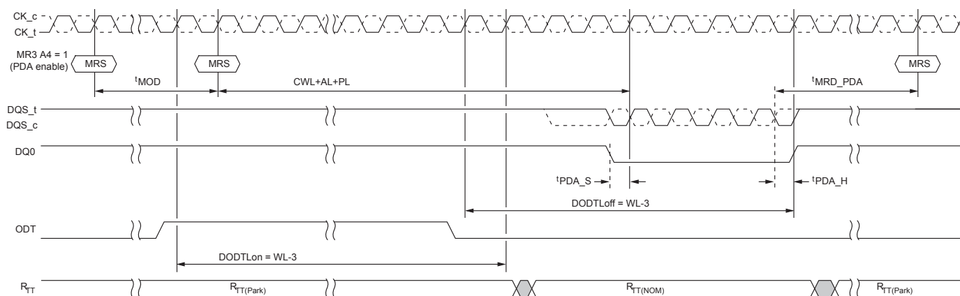
Figure 63: PDA Operation Enabled, BL8
