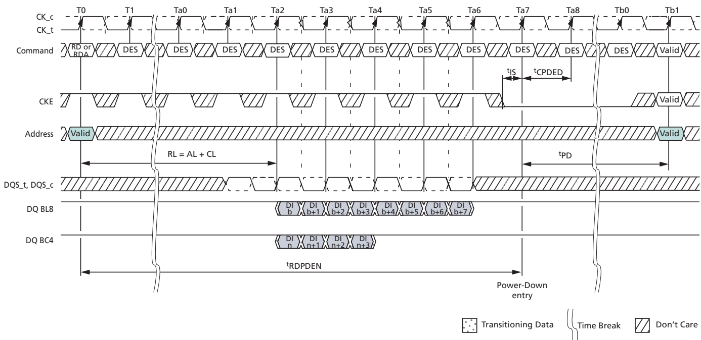
Figure 95: Power-Down Entry After Read and Read with Auto Precharge
