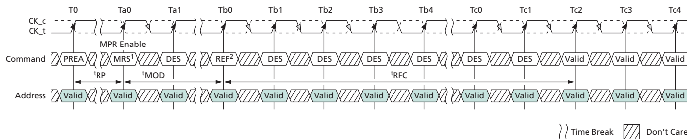
Figure 42: REFRESH Timing
