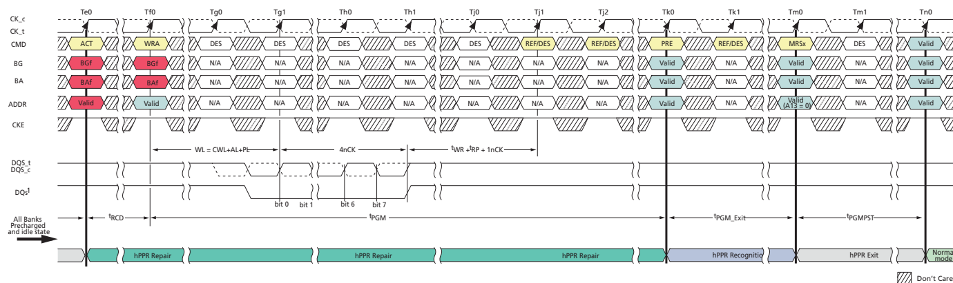
Figure 77: hPPR WRA – Repair and Exit
