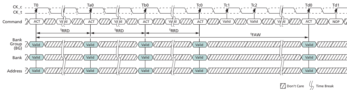
Figure 83: t_{FAW} Timing
