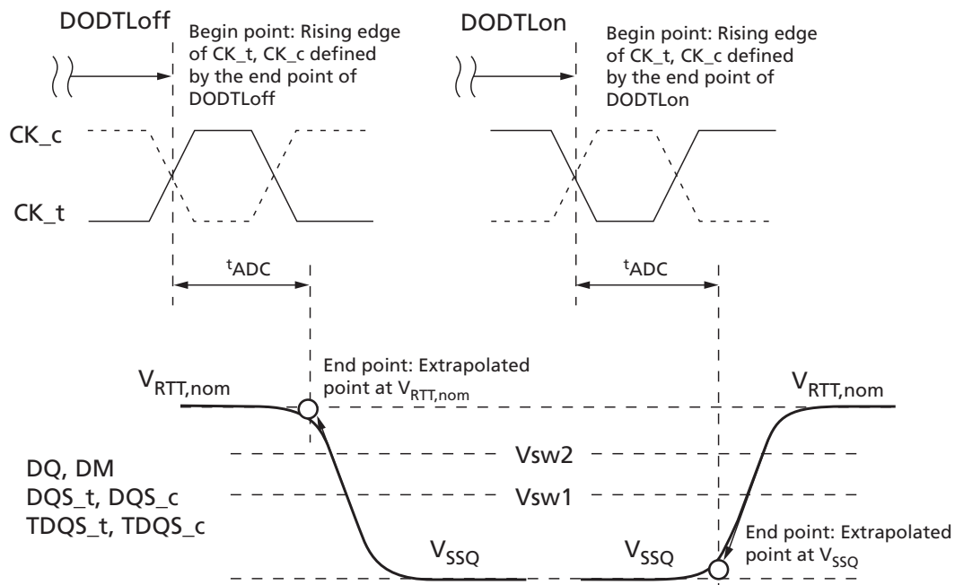
Figure 243: t_{ADC} Definition with Dynamic ODT Control
