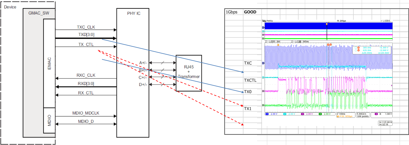
Figure 24-211. RGMII Interface Typical Application
