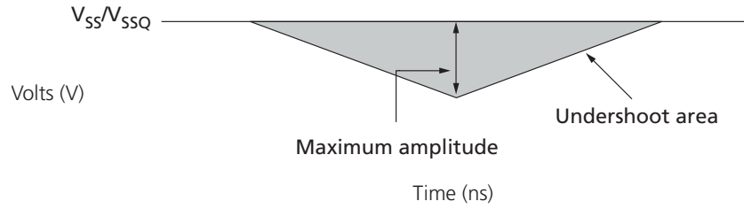
Figure 16: V_{IX} for Differential Signals
