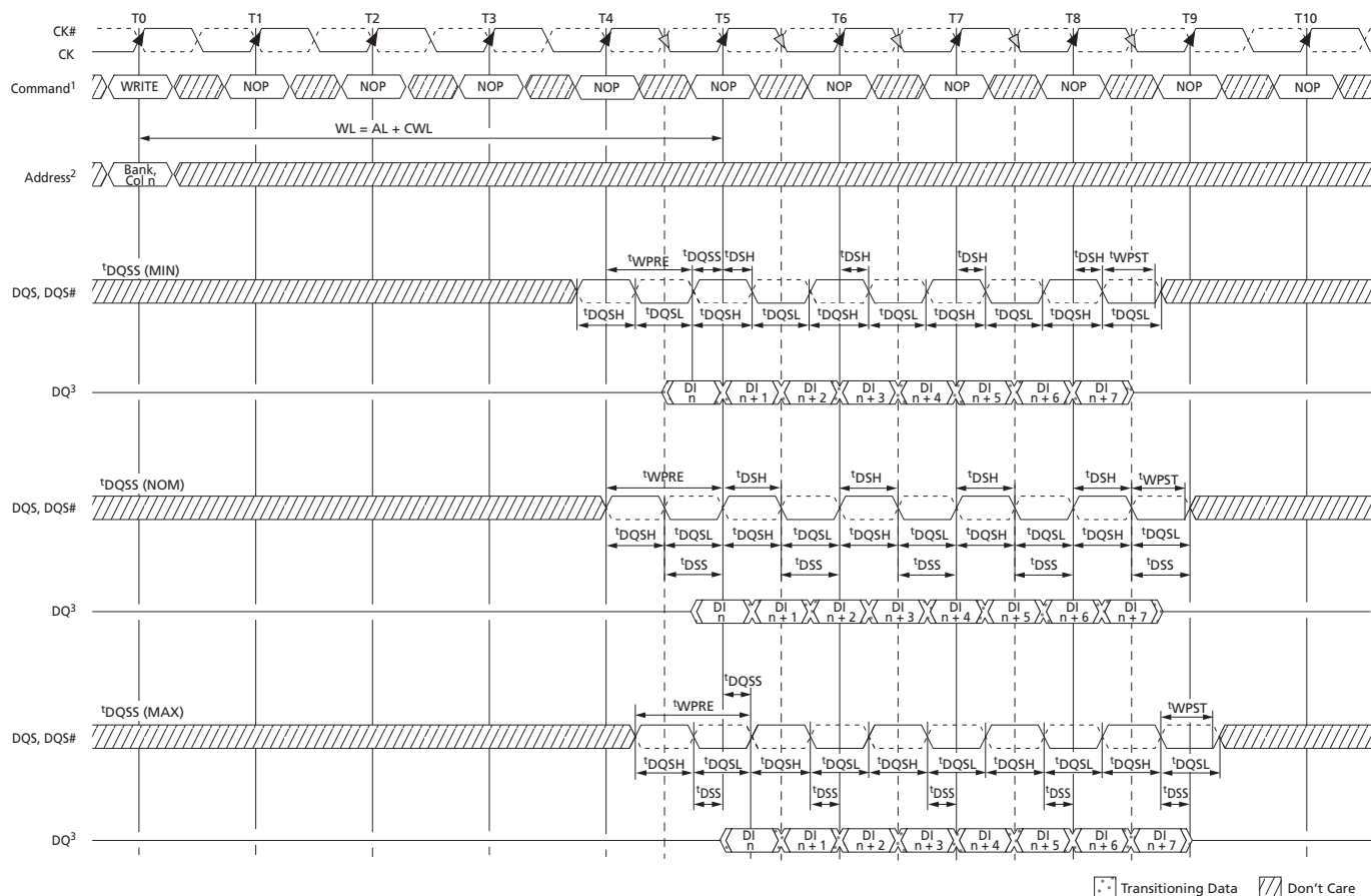
Figure 84: WRITE Burst
