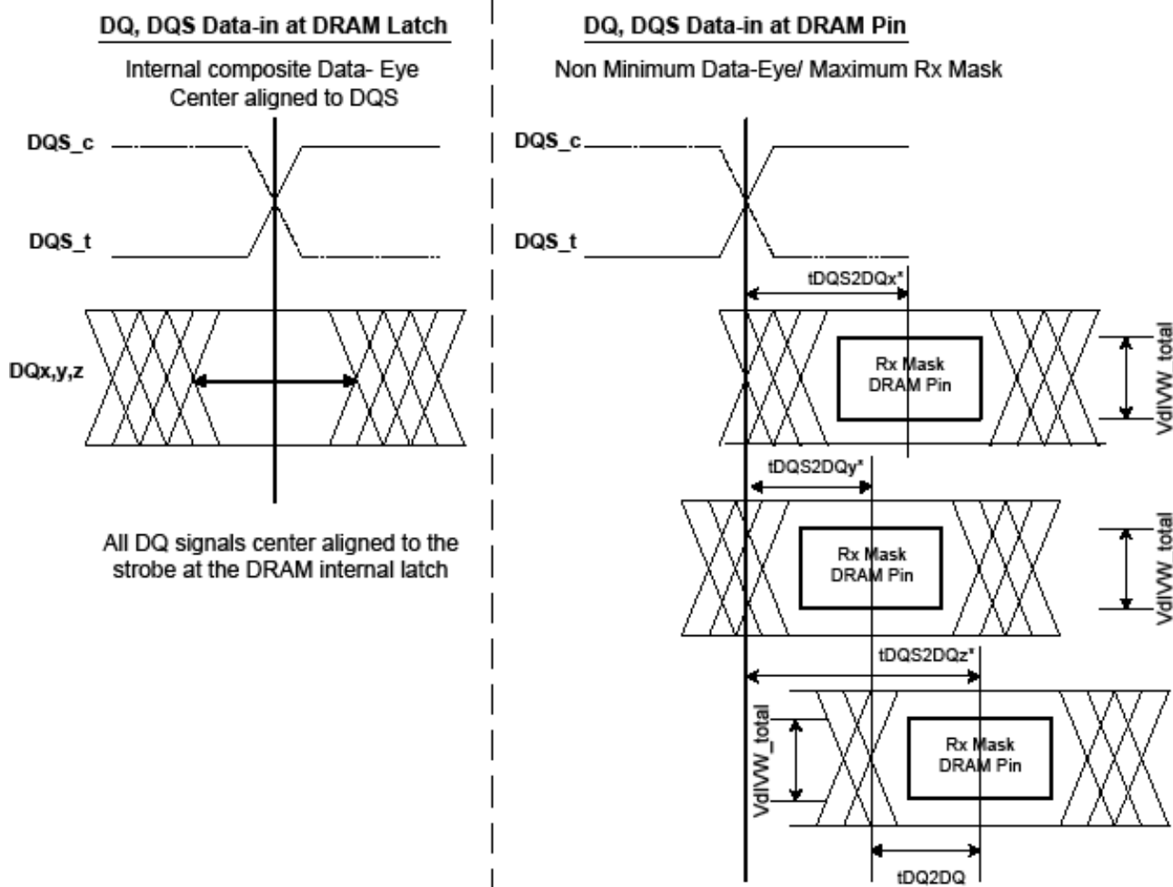
DQ to DQS t_{DQS2DQ} & t_{DQDQ} Timings at the DRAM pins referenced from the internal latch
