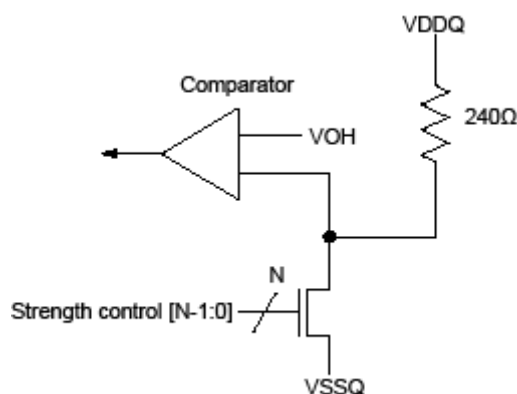
pull-down calibration
