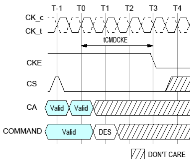
tCMDCKE Timing
