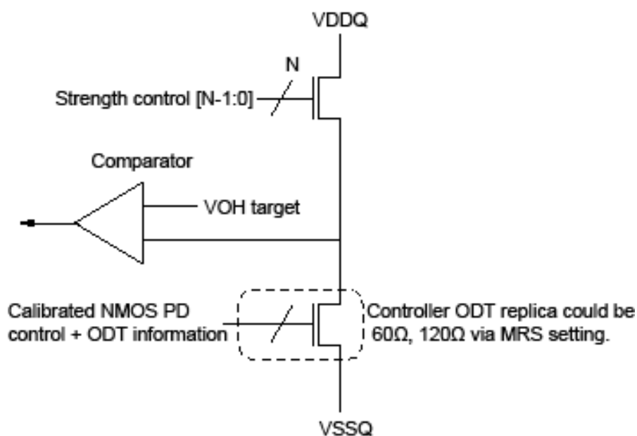
pull-up calibration
