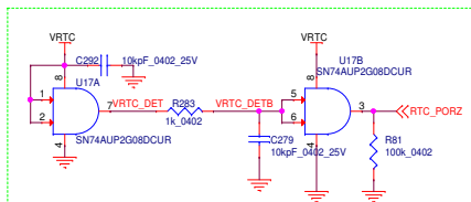
RTC POWER ON RESET
