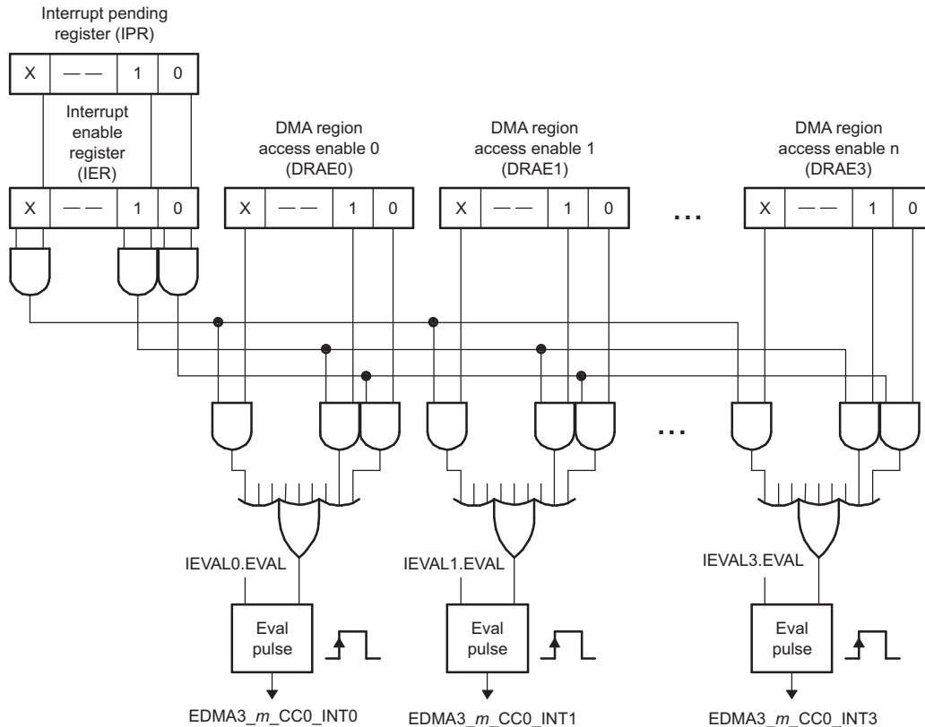
Figure 16-12. Interrupt Diagram
