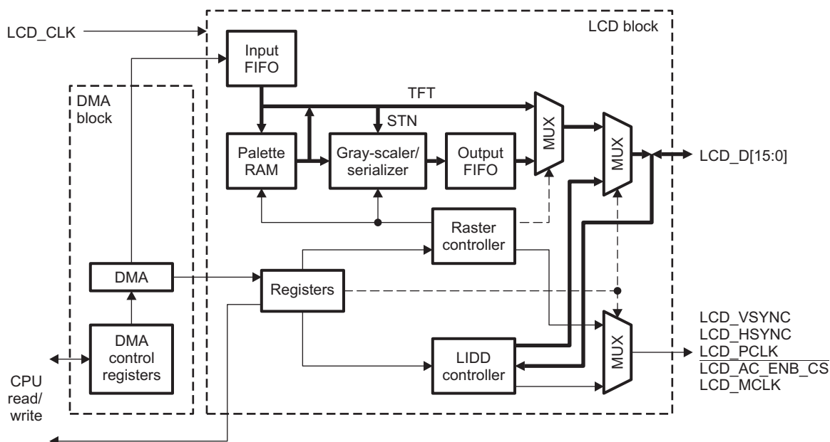
Figure 22-1. LCD Controller
