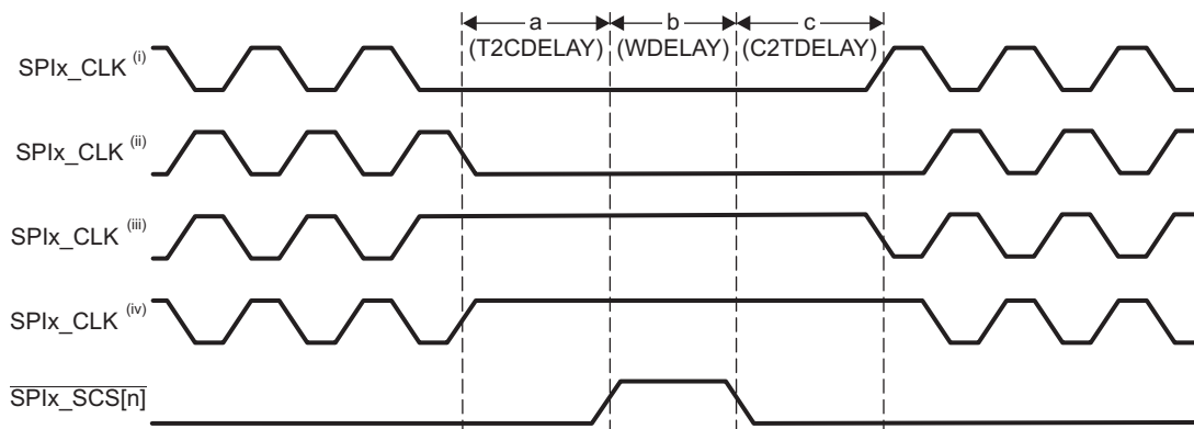
Figure 28-14. SPI 4-Pin with \overline{\text{SPIx\_SCS}}[n] Mode with T2CDELAY, WDELAY, and C2TDELAY
