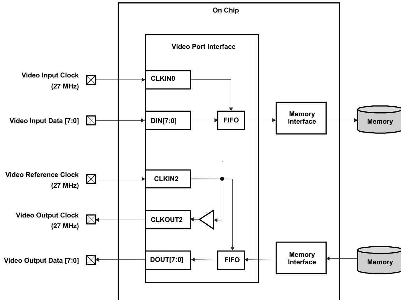
Figure 34-20. Clock Control on Video Input and Output with SDTV Encoding
