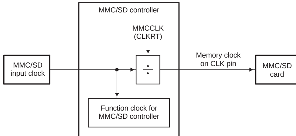
Figure 25-4. MMC/SD Controller Clocking Diagram
