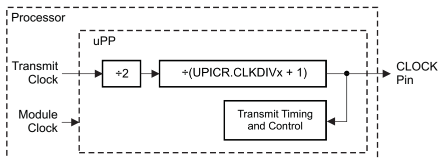
Figure 31-6. Clock Generation for a Channel Configured in Transmit Mode
