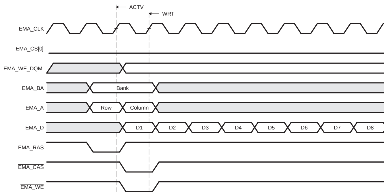
Figure 18-6. Timing Waveform for Basic SDRAM Write Operation
