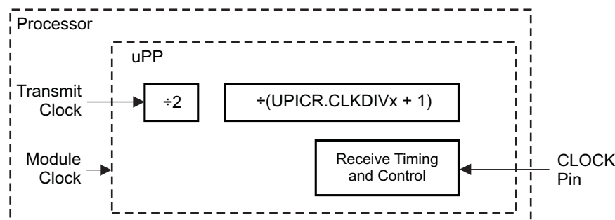
Figure 31-7. Clock Generation for a Channel Configured in Receive Mode
