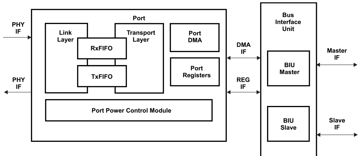
Figure 27-2. SATA Core Block Diagram
