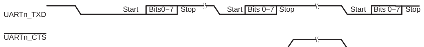
Figure 30-7. Autoflow Functional Timing Waveforms for UARTn_CTS
