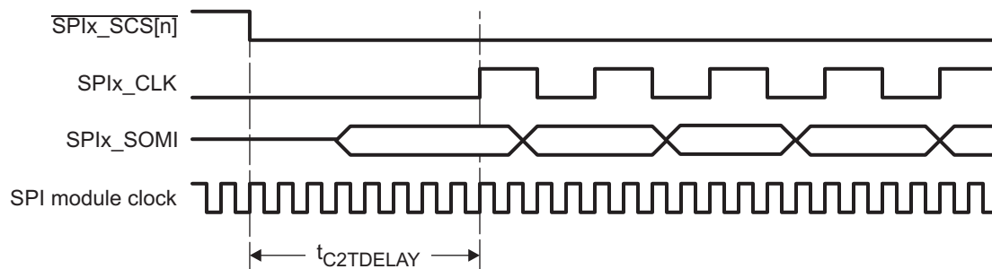
Figure 28-34. Example: t_{\text{C2DELAY}} = 8 SPI Module Clock Cycles
