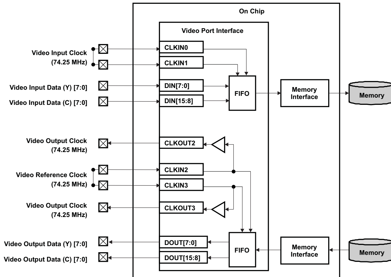
Figure 34-21. Clock Control on Video Input and Output with HDTV Encoding
