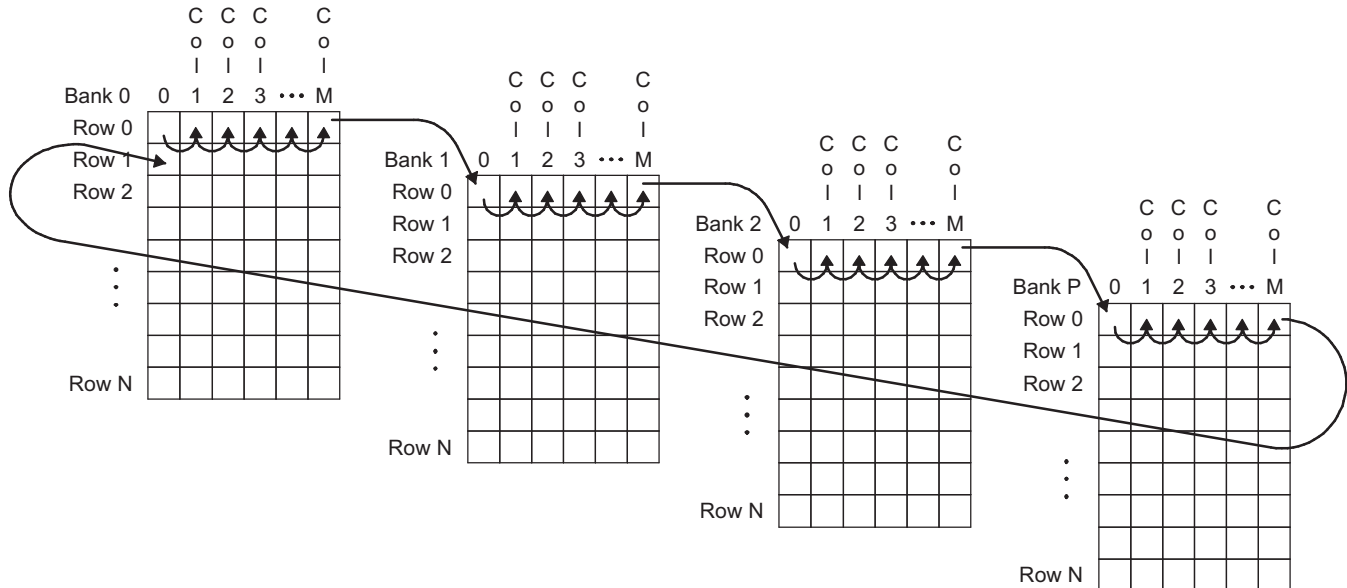
Figure 13-13. DDR2/mDDR SDRAM Column, Row, and Bank Access
