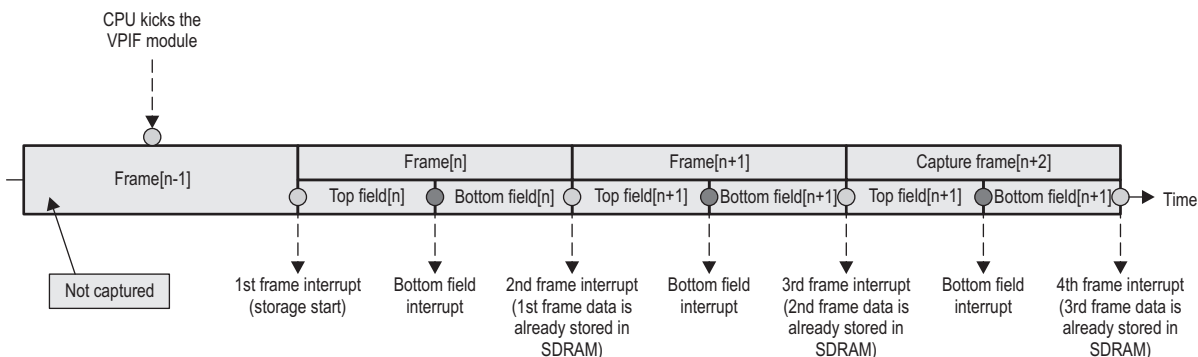
Figure 34-15. Relationship Between the First Interrupt and Incoming Data
