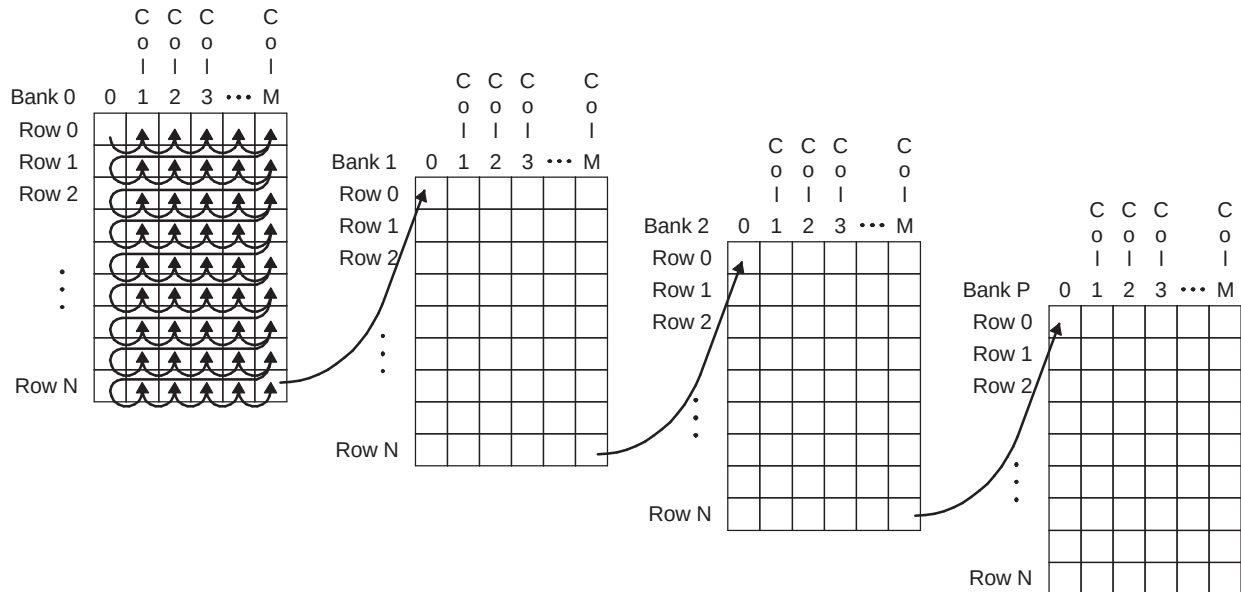
Figure 13-15. SDRAM Column, Row, Bank Access (IBANKPOS = 1)
