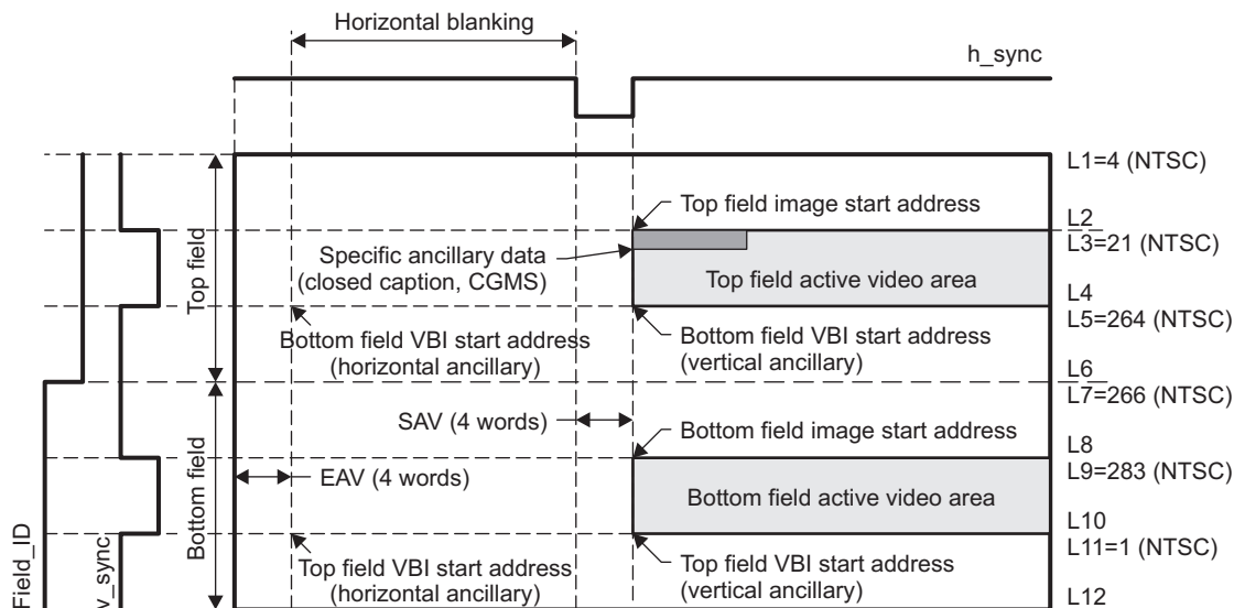
Figure 34-12. Image of Specific Ancillary Data on NTSC
