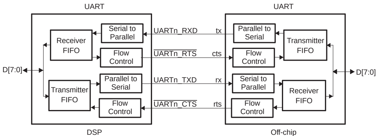
Figure 30-5. UART Interface Using Autoflow Diagram
