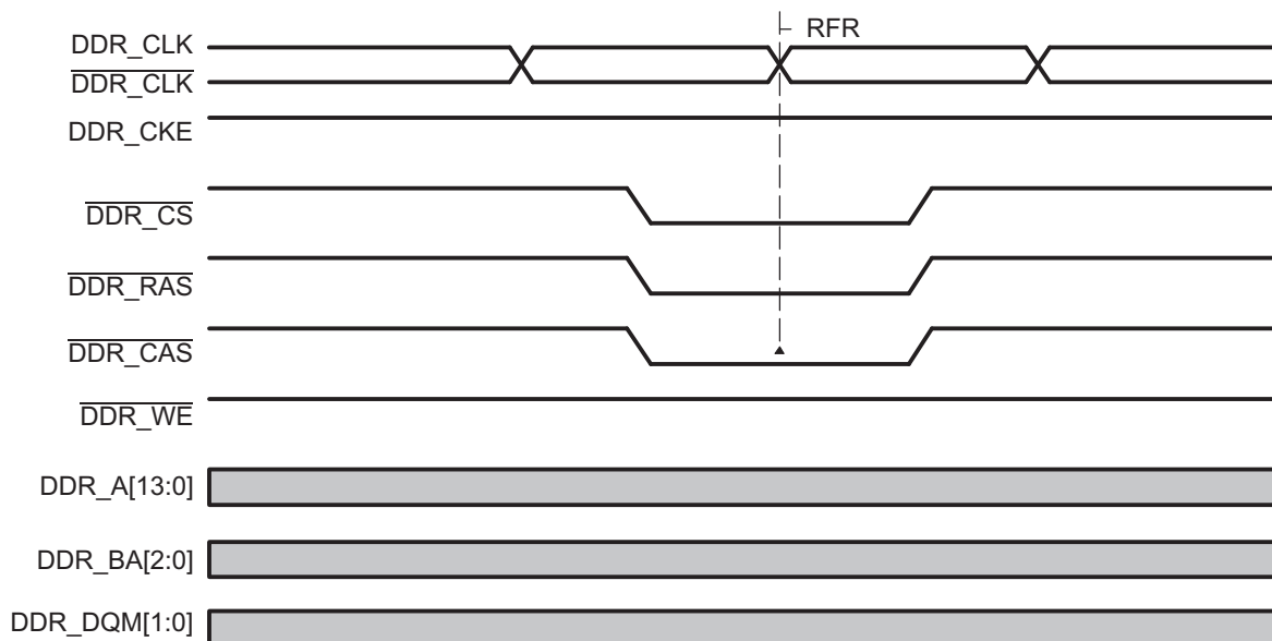
Figure 13-4. Refresh Command
