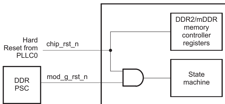
Figure 13-17. DDR2/mDDR Memory Controller Reset Block Diagram
