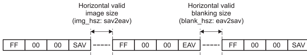
Figure 34-46. Horizontal Distance in Y/C Mode
