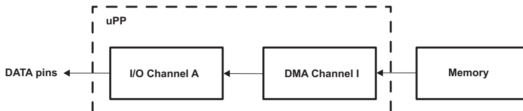
Figure 31-3. Data Flow for Single-Channel Transmit Mode
