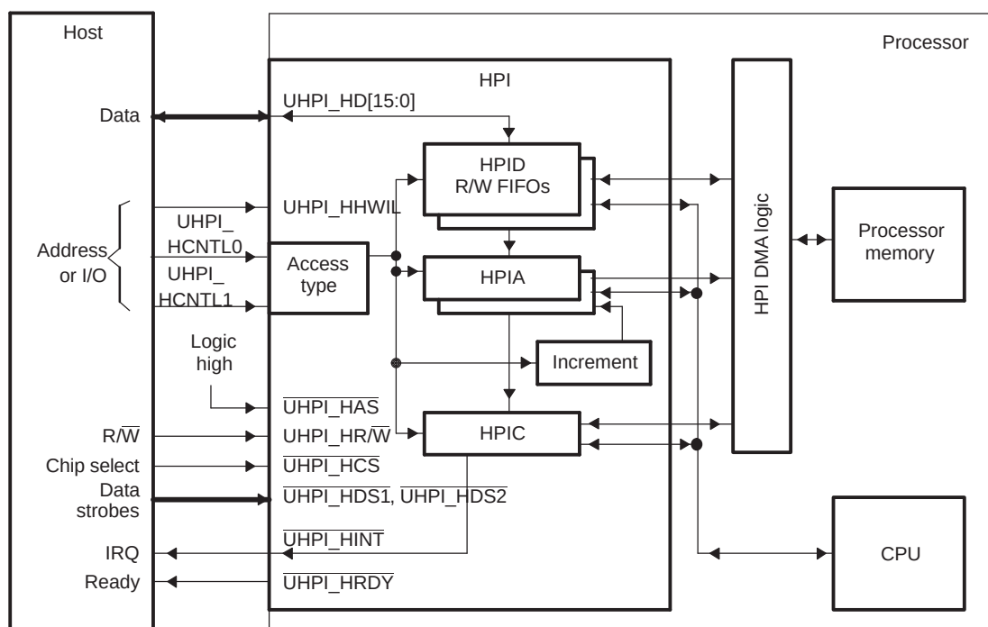
Figure 20-1. HPI Block Diagram
