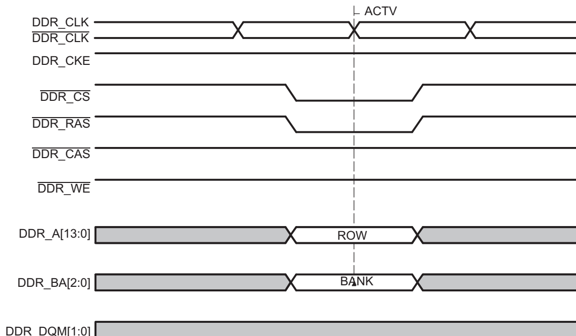
Figure 13-7. ACTV Command
