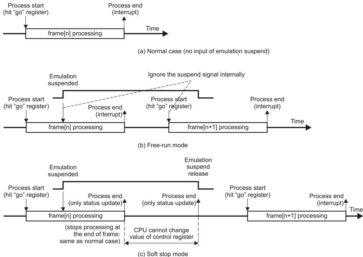
Figure 34-17. Module Performance with Emulation Suspend Signal
