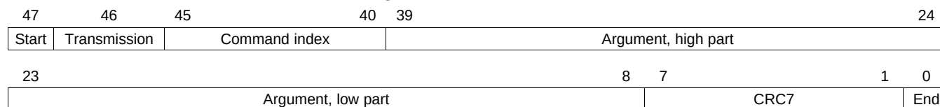
Figure 25-30. Command Format
