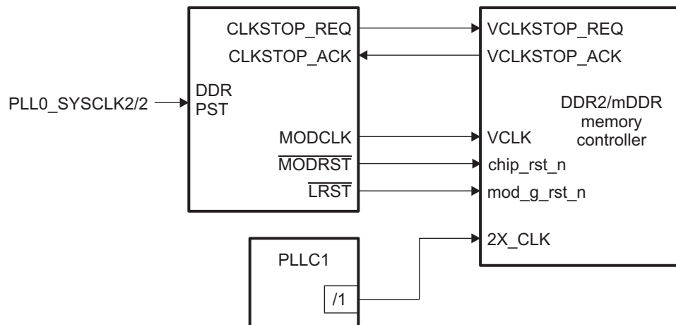
Figure 13-18. DDR2/mDDR Memory Controller Power Sleep Controller Diagram
