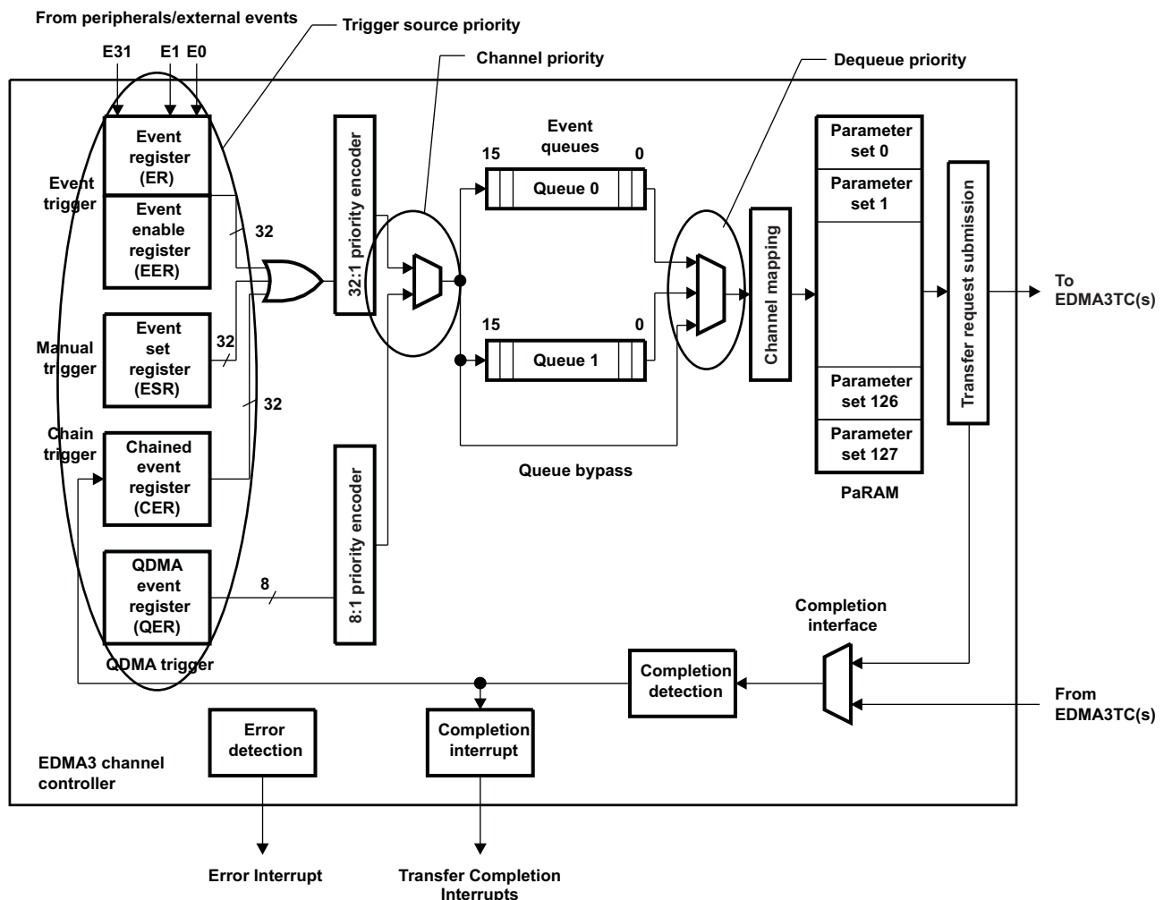
Figure 16-14. EDMA3 Prioritization
