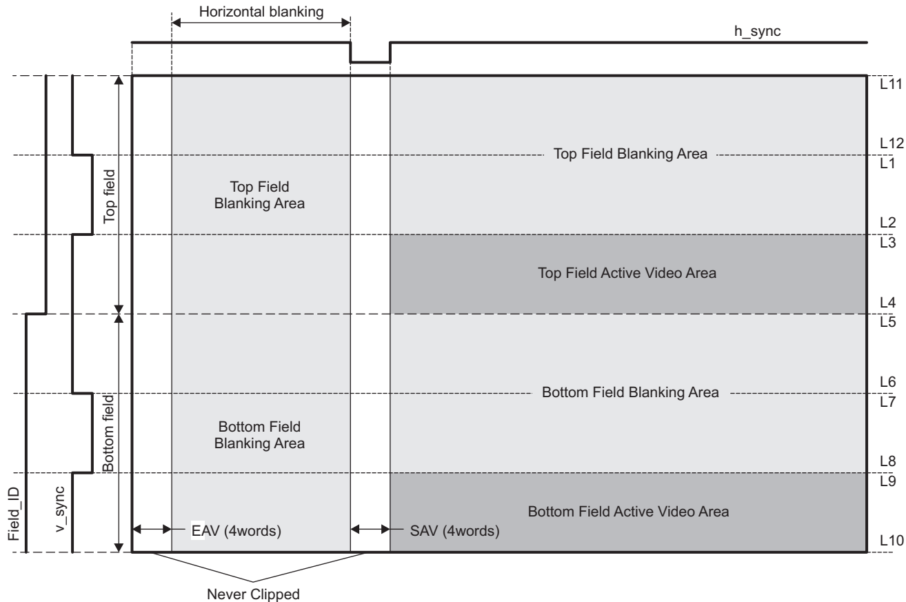
Figure 34-13. Data Areas and Clipping Function
