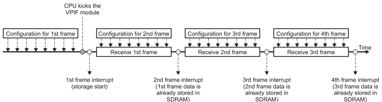
Figure 34-23. Relationship Between Register and Data Access
