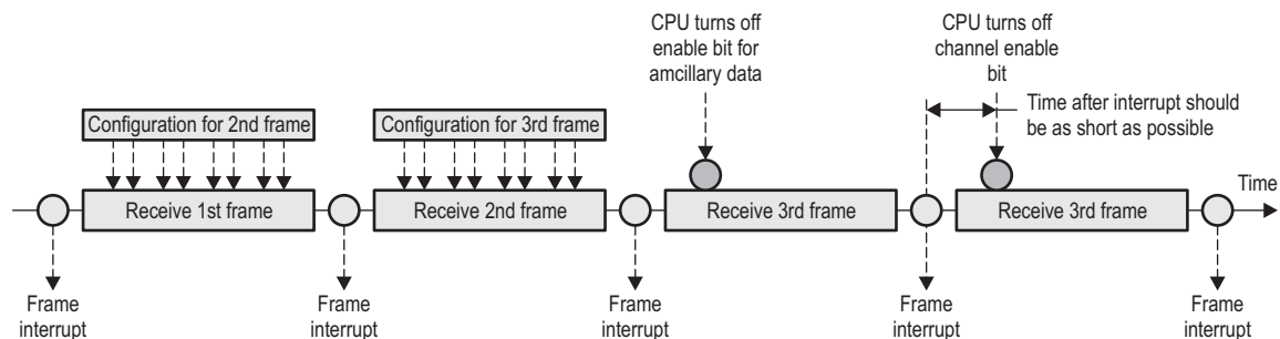
Figure 34-19. Method for Turning off Module Channel
