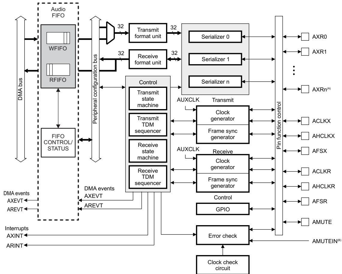
Figure 23-1. McASP Block Diagram
