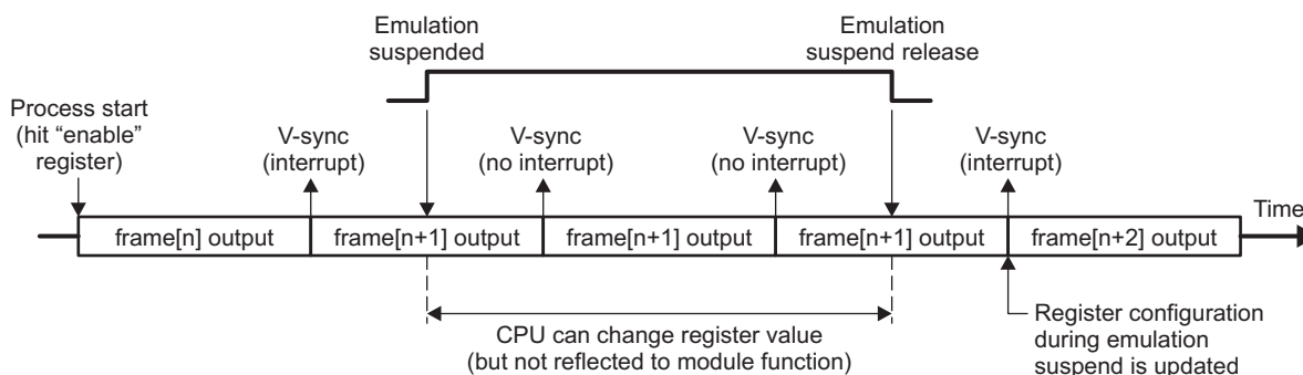
Figure 34-18. Emulation Suspend Function on Channels 2 and 3 (Transmit)
