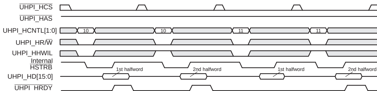
Figure 20-11. \overline{\text{UHPI\_HRDY}} Behavior During a Data Write Operation in the Multiplexed Mode (Case 1: No Autoincrementing)
