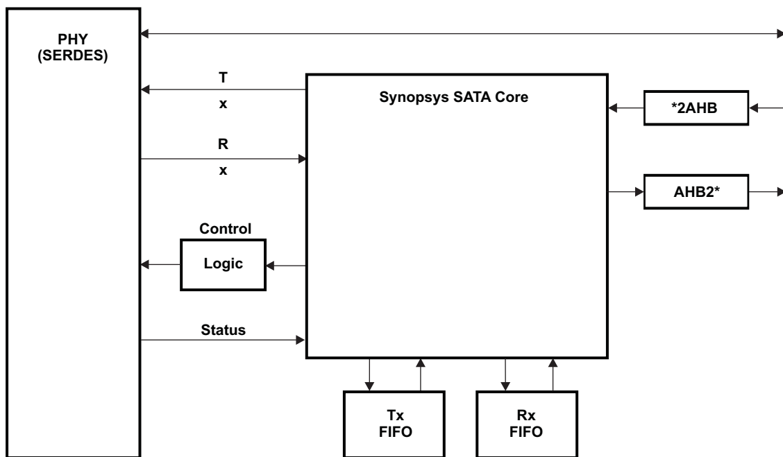
Figure 27-1. SATA Subsystem Functional Block Diagram
