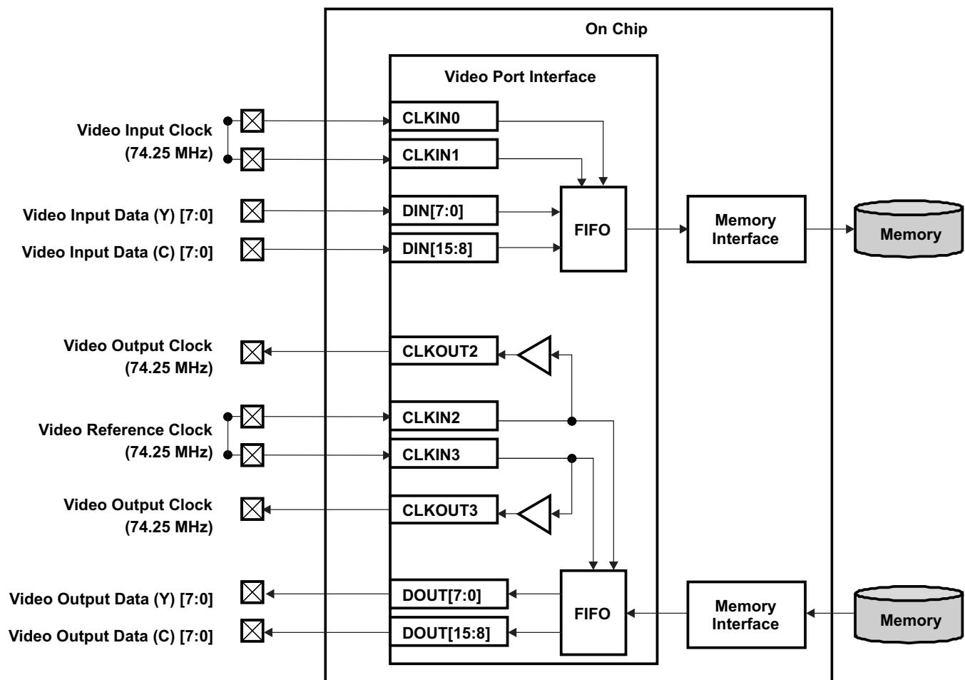
Figure 34-22. Clock Control on Video Input and Output with HDTV Encoding
