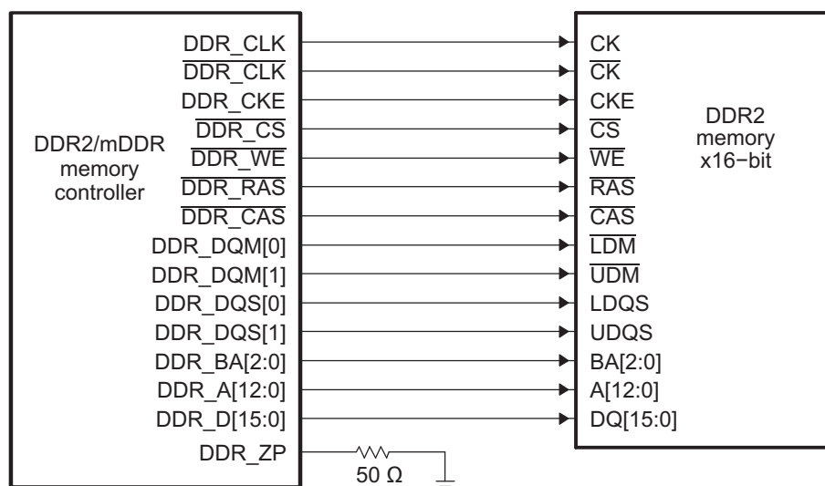
Figure 13-19. Connecting DDR2/mDDR Memory Controller to a 16-Bit DDR2 Memory
