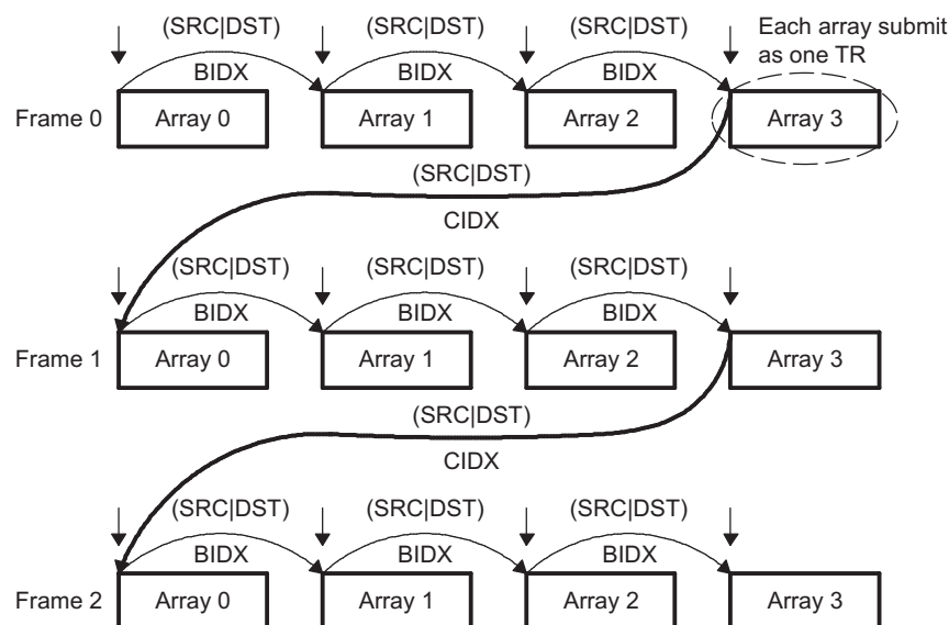
Figure 16-5. A-Synchronized Transfers (ACNT = n, BCNT = 4, CCNT = 3)
