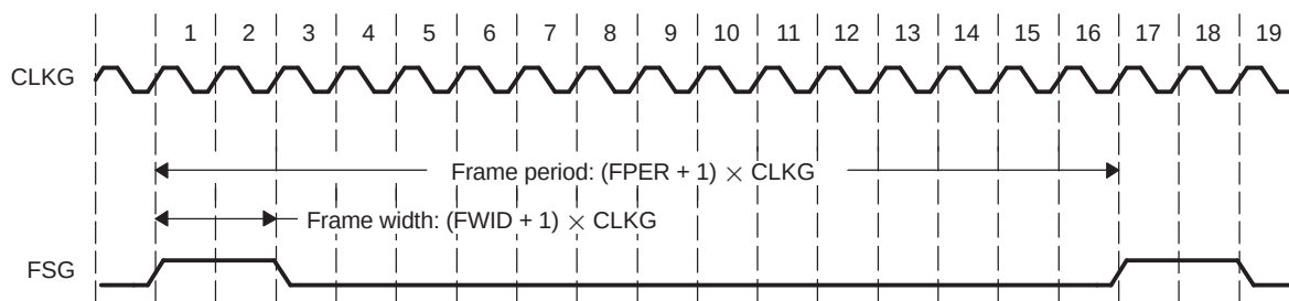
Figure 24-9. Programmable Frame Period and Width
