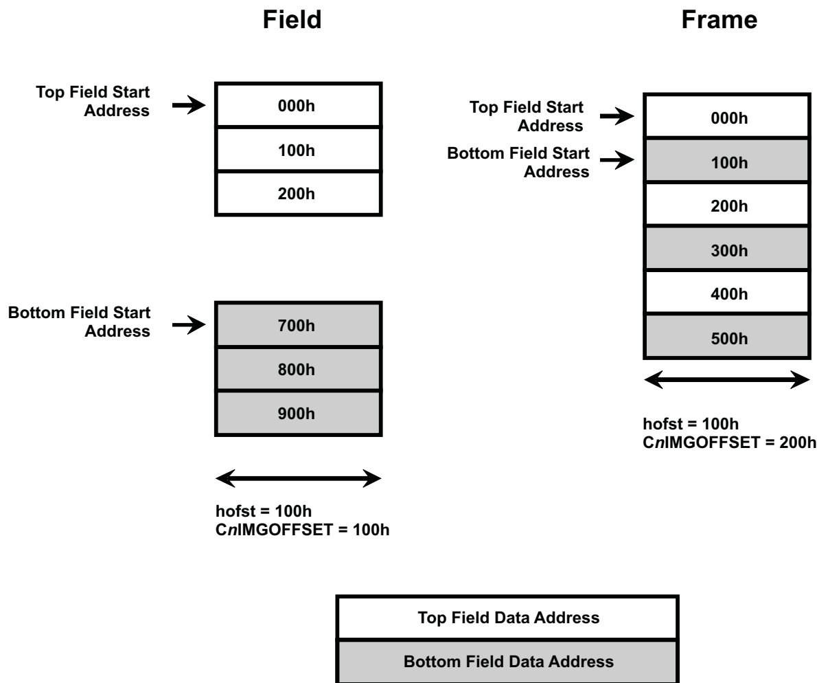
Figure 34-6. Memory Storage Modes for Interlaced Video
