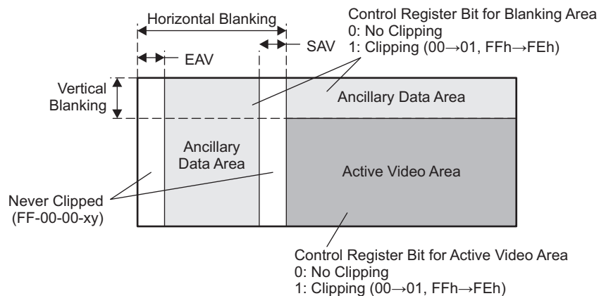
Figure 34-14. Register Bit Assignment on Clipping Function
