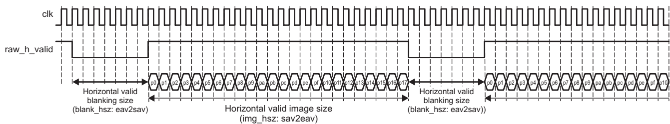
Figure 34-47. Horizontal Distance in CCD/CMOS Mode
