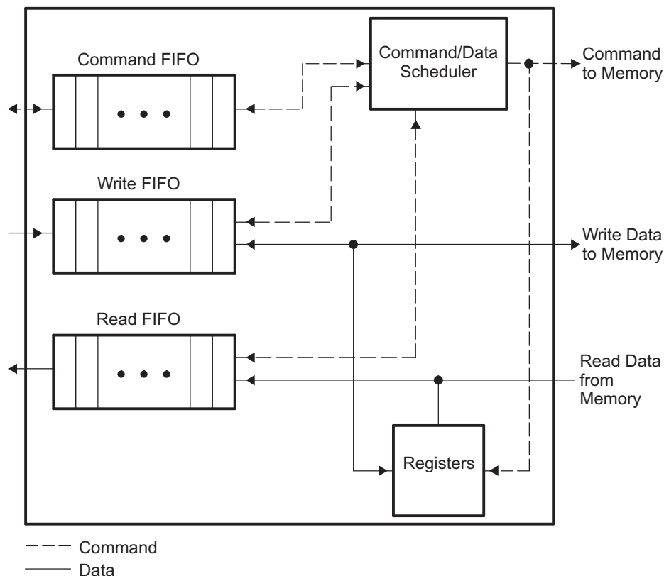
Figure 13-16. DDR2/mDDR Memory Controller FIFO Block Diagram
