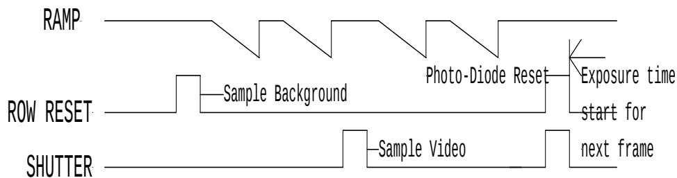
Figure #11: Correlated Multi-Sampling (CMS) Timing Example
