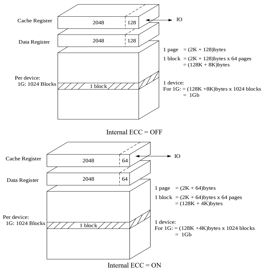
Figure 3. Array Organization
