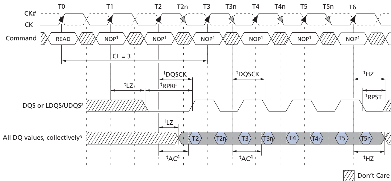
Figure 37: Data Output Timing – t_{AC} and t_{DQSCK}
