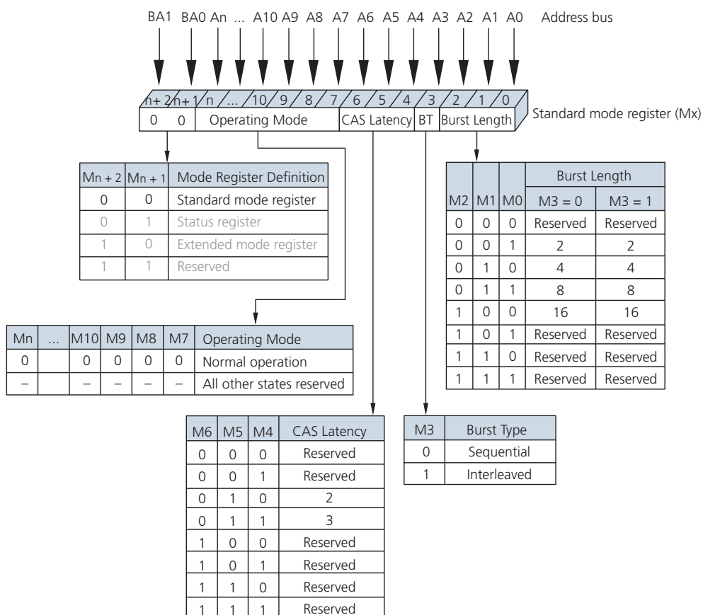
Figure 23: Standard Mode Register Definition
