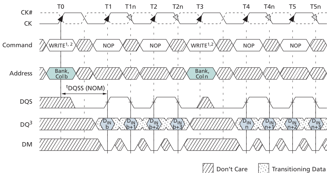
Figure 42: Nonconsecutive WRITE-to-WRITE
