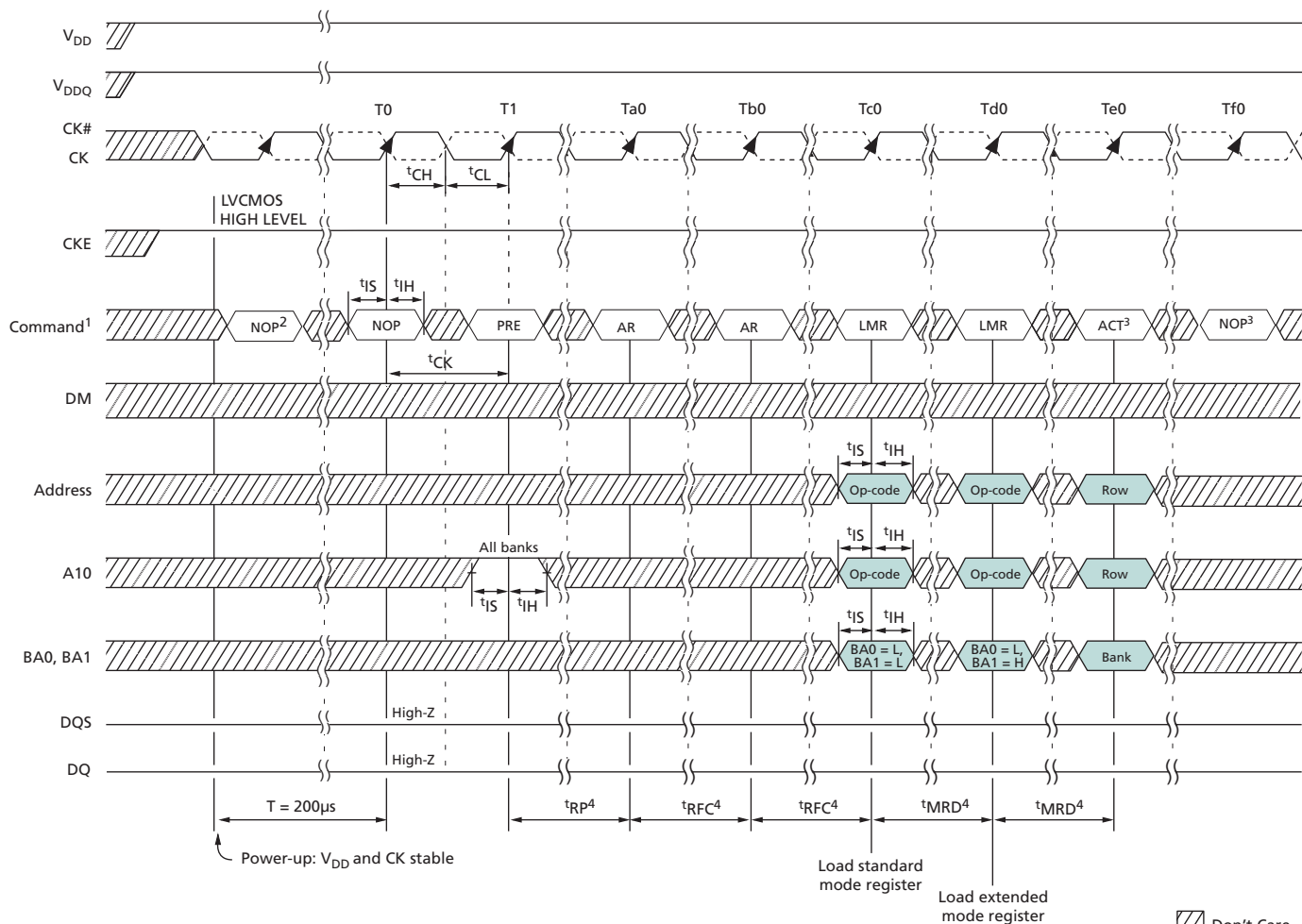
Figure 21: Initialize and Load Mode Registers
