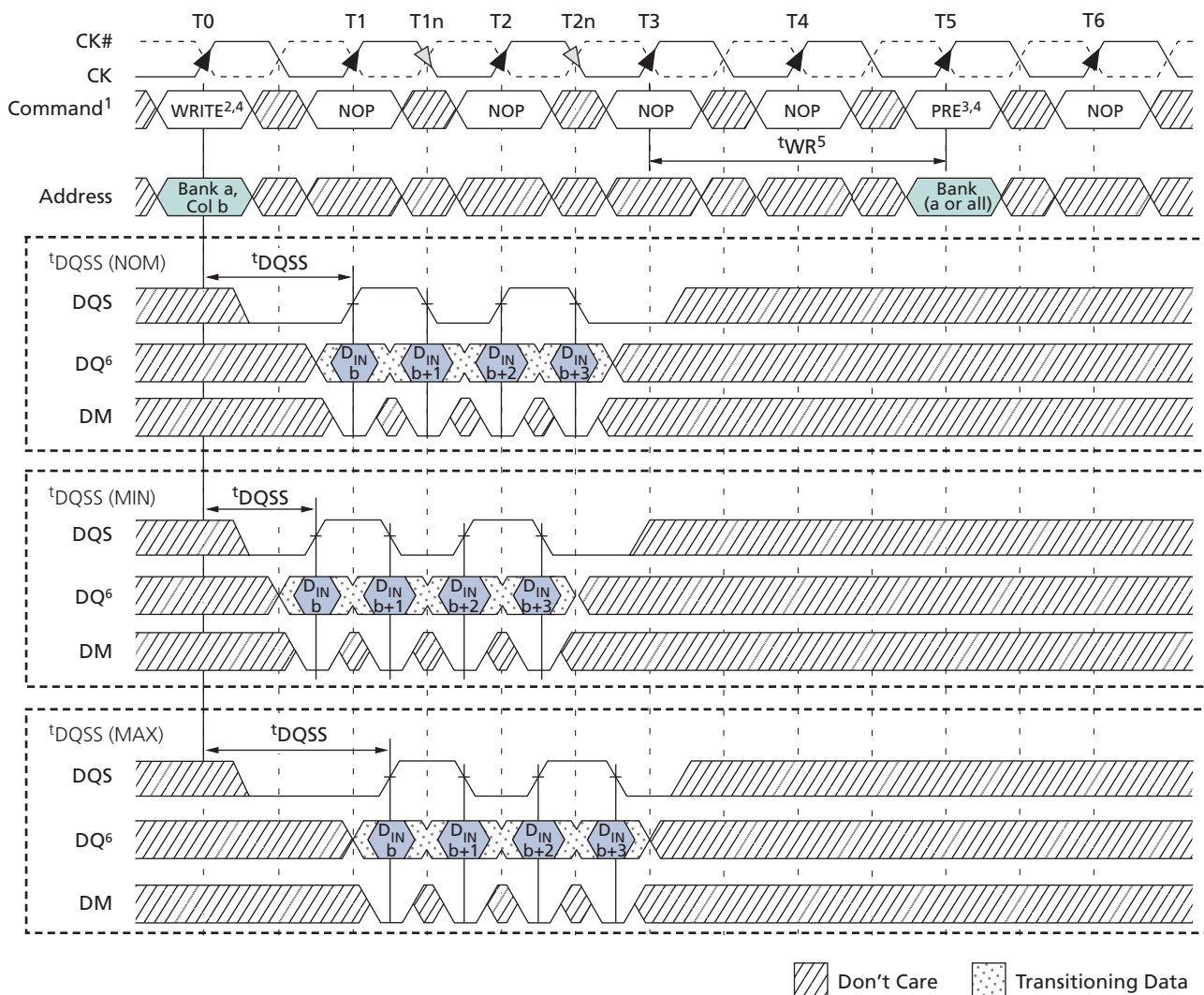
Figure 47: WRITE-to-PRECHARGE – Uninterrupting
