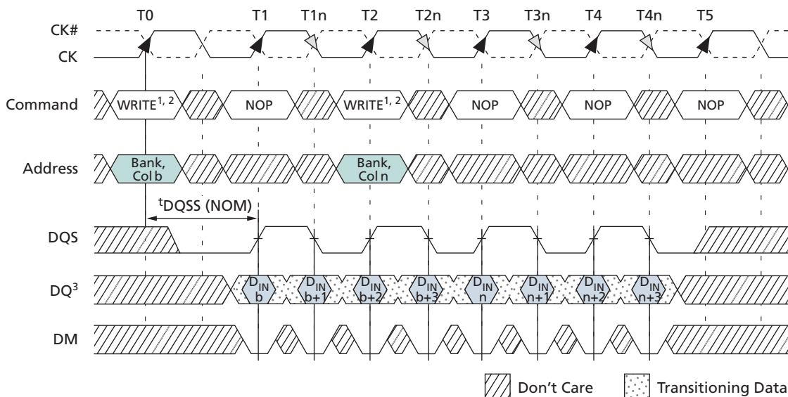
Figure 41: Consecutive WRITE-to-WRITE
