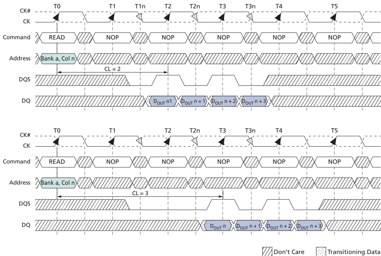
Figure 28: READ Burst
