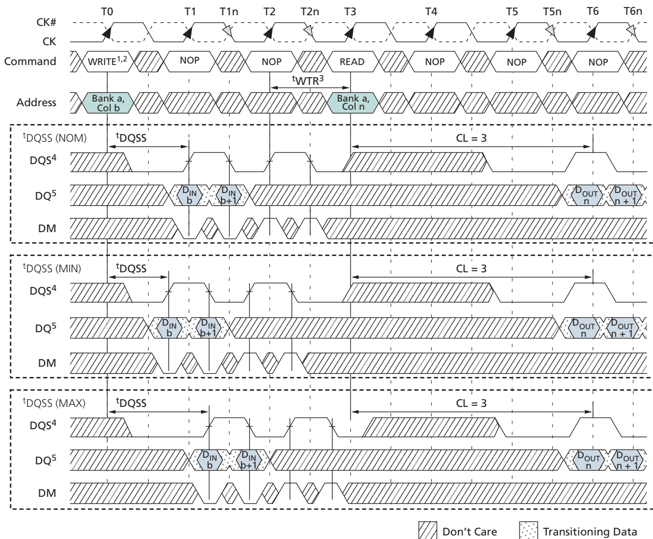
Figure 45: WRITE-to-READ – Interrupting
