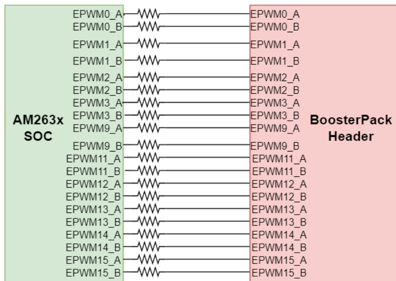
Figure 4-23. EPWM Signal Mapping to BoosterPack Header
