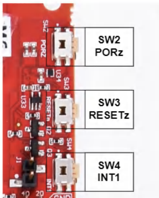
Figure 3-5. Push Buttons
