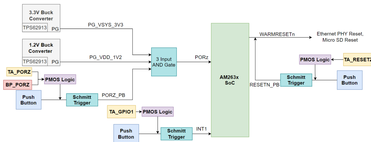
Figure 4-2. Reset Architecture
