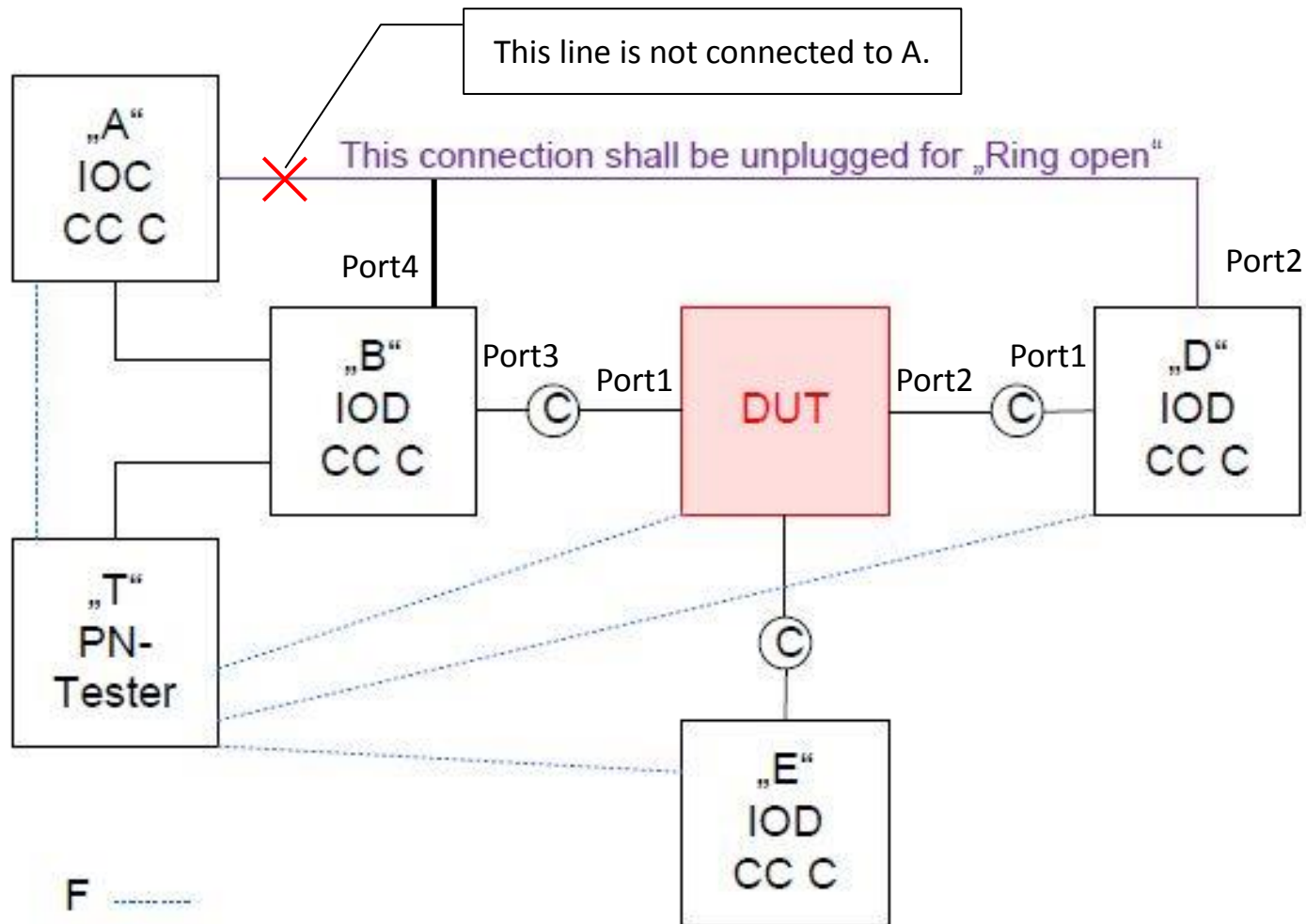
Figure 7-15 MRP test setup
