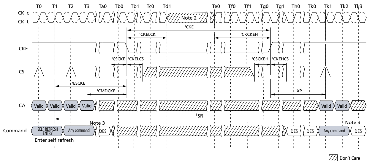
Figure 82: Command Input Timings after Power-Down Exit During Self Refresh
