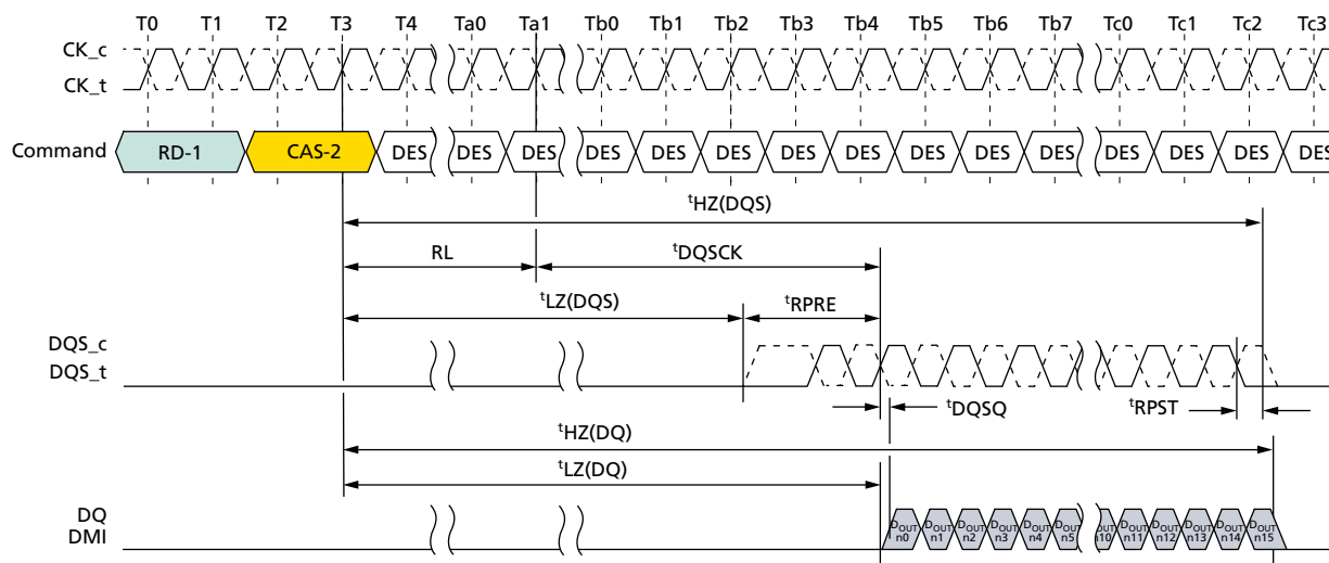
Figure 25: Read Timing
