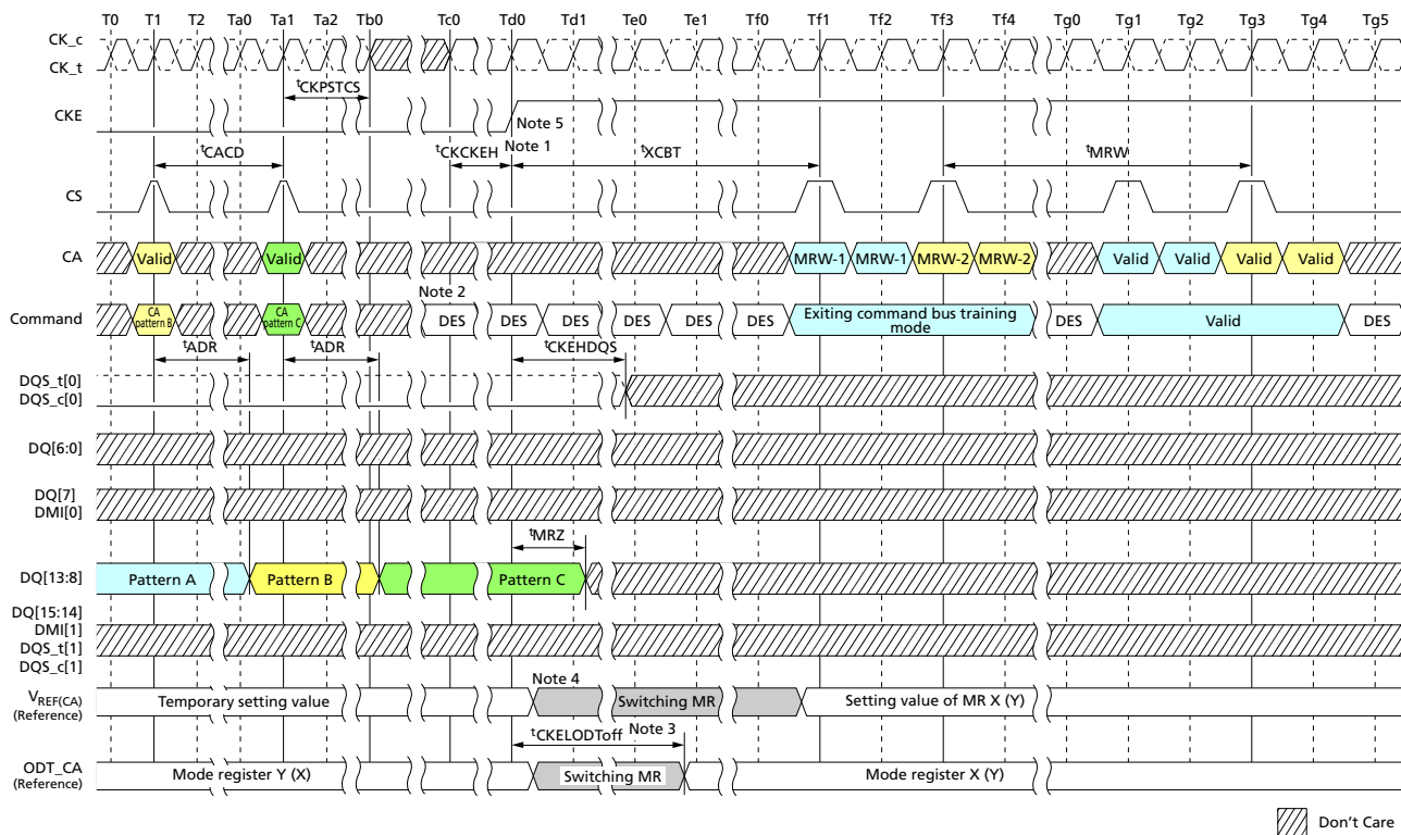
Figure 118: Command Bus Training Mode Exit with Valid Command
