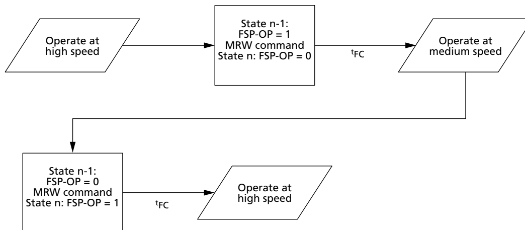
Figure 142: Example of Switching Between Two Trained Frequency Set Points
