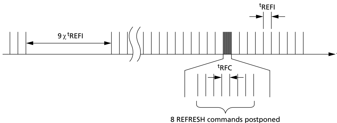
Figure 76: Postponing REFRESH Commands (Example)
