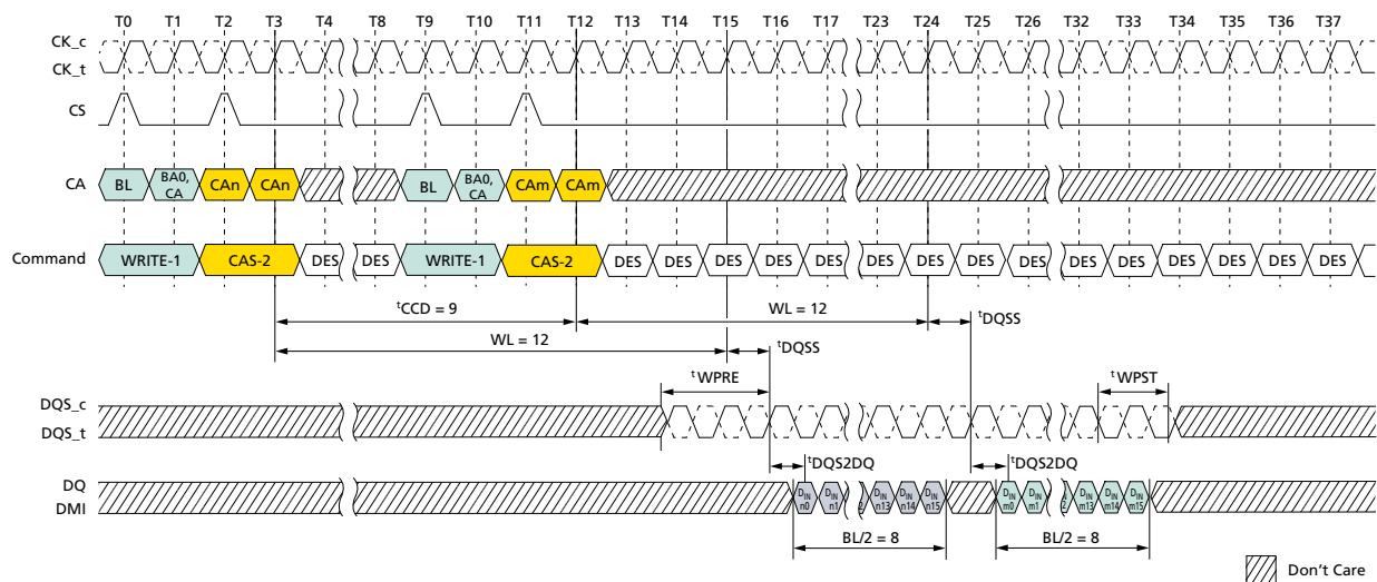
Figure 60: Consecutive WRITE: t_{CCD} = \text{MIN} + 1, 1.5nCK Postamble
