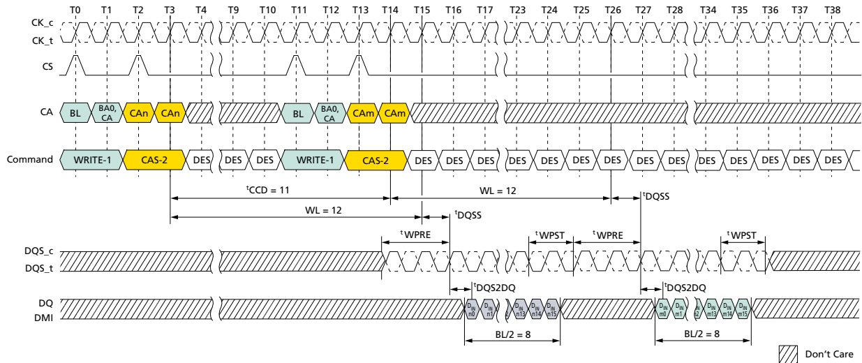
Figure 64: Consecutive WRITE: t_{CCD} = \text{MIN} + 3, 1.5nCK Postamble
