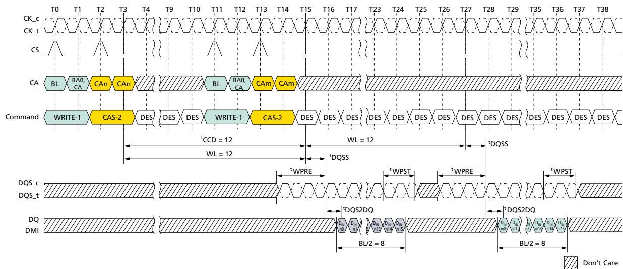
Figure 65: Consecutive WRITE: t_{CCD} = \text{MIN} + 4, 1.5n\text{CK} Postamble
