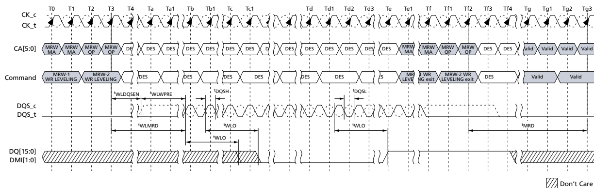
Figure 121: Write Leveling Timing – t_{DQSL}(\text{MIN})
