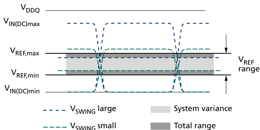
Figure 109: V_{REF} Operating Range ( V_{REF,max} , V_{REF,min} )
