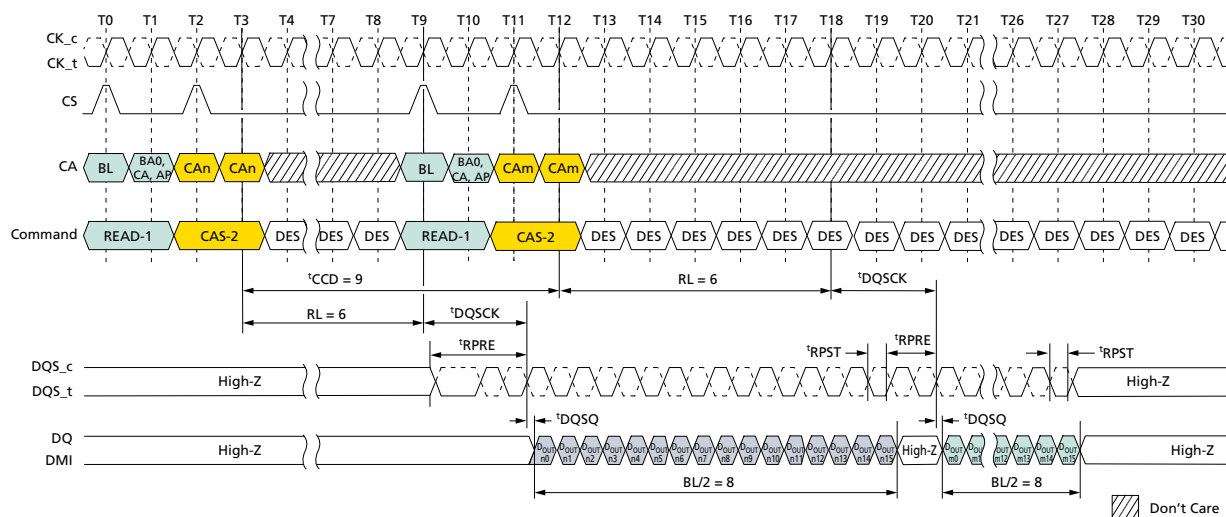
Figure 45: Consecutive READ: t_{CCD} = \text{MIN} + 1 , Preamble = Toggle, 0.5n\text{CK} Postamble
