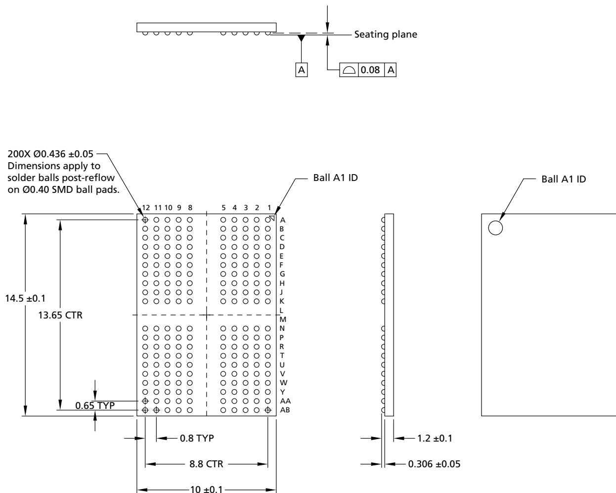
Figure 12: 200-Ball LFBGA – 10mm x 14.5mm x 1.3mm (Package Code: GS)
