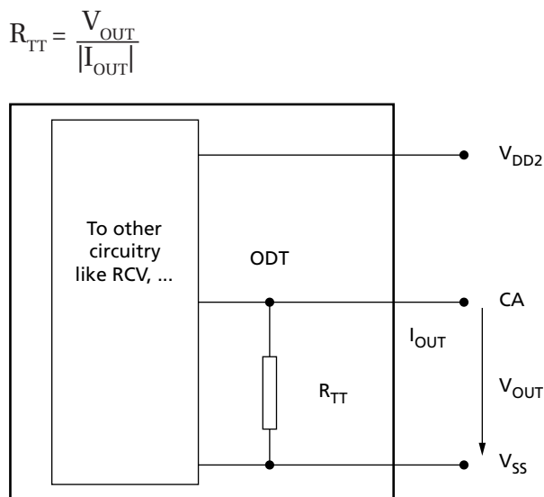
Figure 144: ODT for CA
