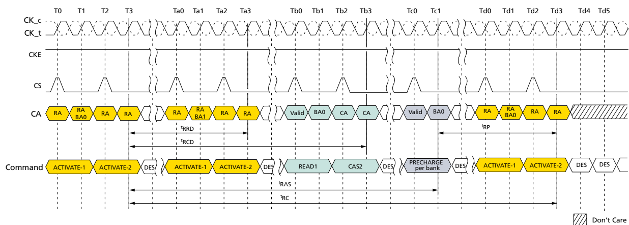
Figure 16: ACTIVATE Command
