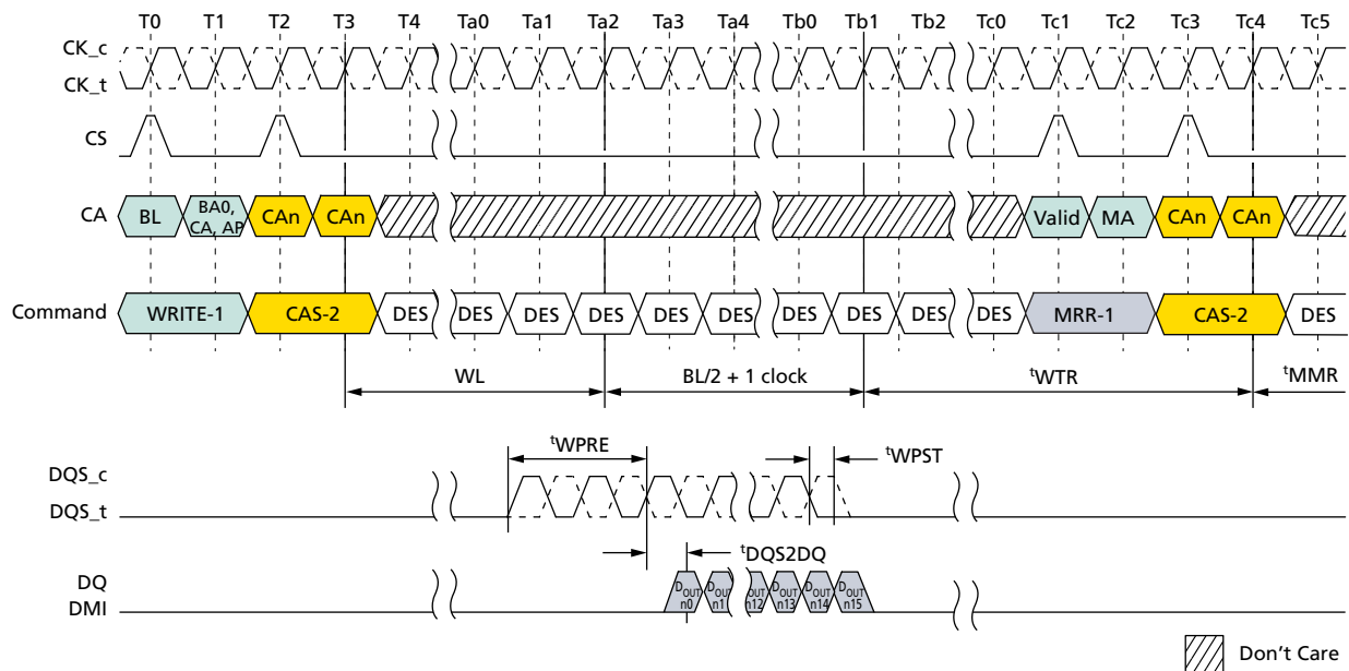
Figure 97: WRITE-to-MRR Timing
