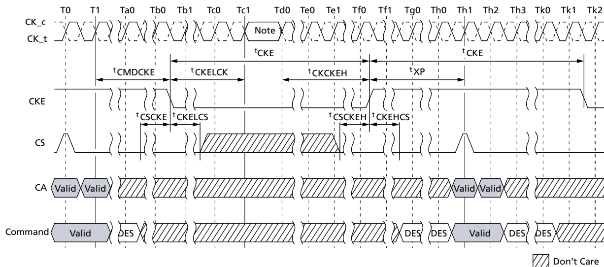
Figure 85: Basic Power-Down Entry and Exit Timing
