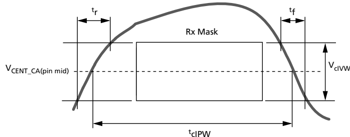
Figure 174: CA t_{cIPW} and SRIN_cIVW Definition (for Each Input Pulse)
