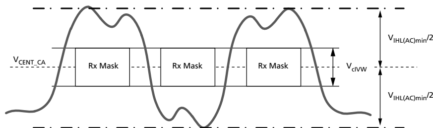
Figure 175: CA V_{IHL\_AC} Definition (for Each Input Pulse)
