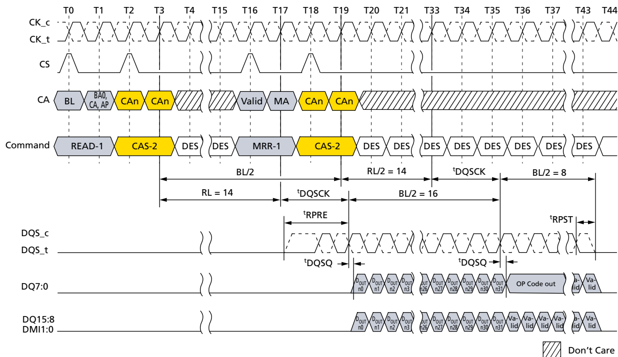
Figure 96: READ-to-MRR Timing
