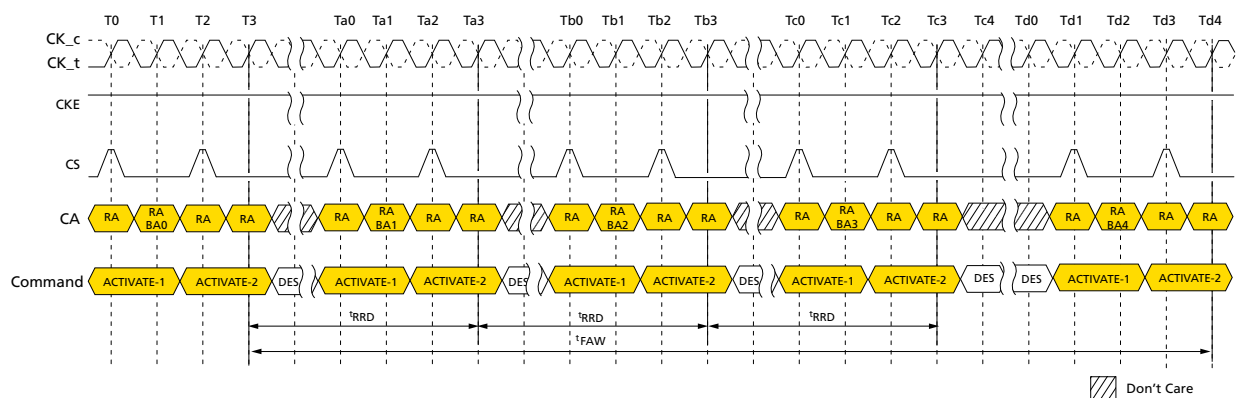
Figure 17: t_{FAW} Timing
