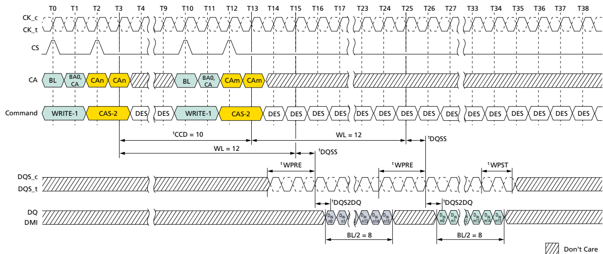
Figure 62: Consecutive WRITE: t_{CCD} = \text{MIN} + 2, 1.5n\text{CK} Postamble
