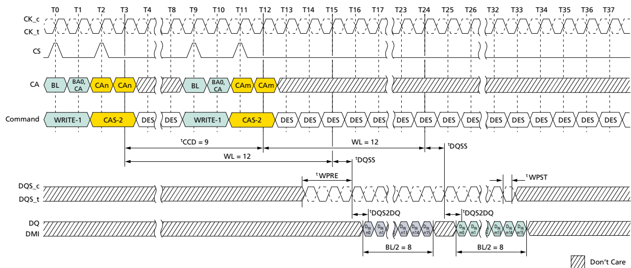
Figure 59: Consecutive WRITE: t_{CCD} = \text{MIN} + 1, 0.5nCK Postamble
