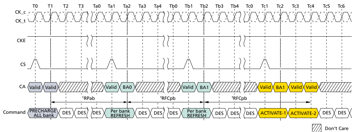
Figure 75: Per-Bank REFRESH Operation
