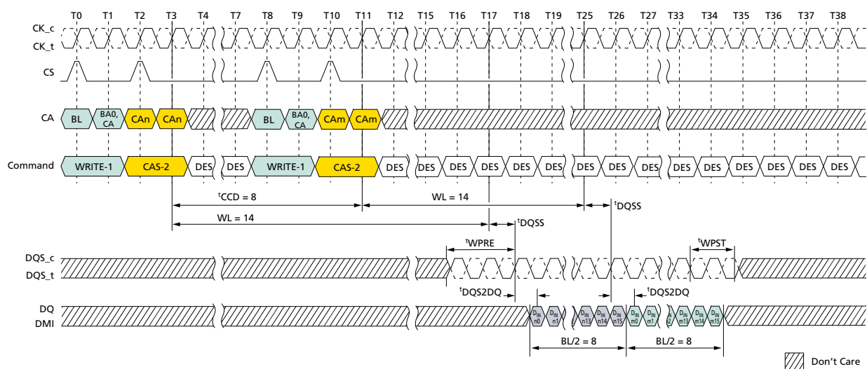
Figure 58: Seamless WRITE: t_{CCD} = \text{MIN} , 1.5nCK Postamble
