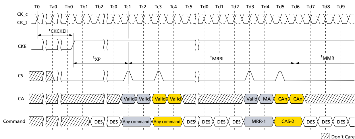
Figure 98: MRR Following Power-Down
