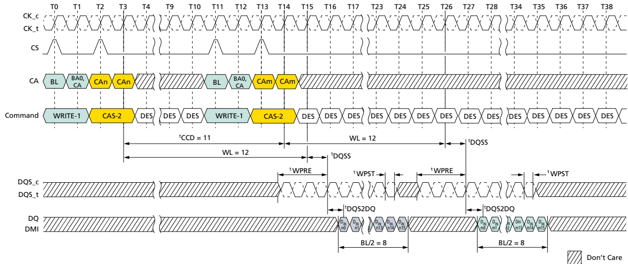
Figure 63: Consecutive WRITE: t_{CCD} = \text{MIN} + 3, 0.5nCK Postamble
