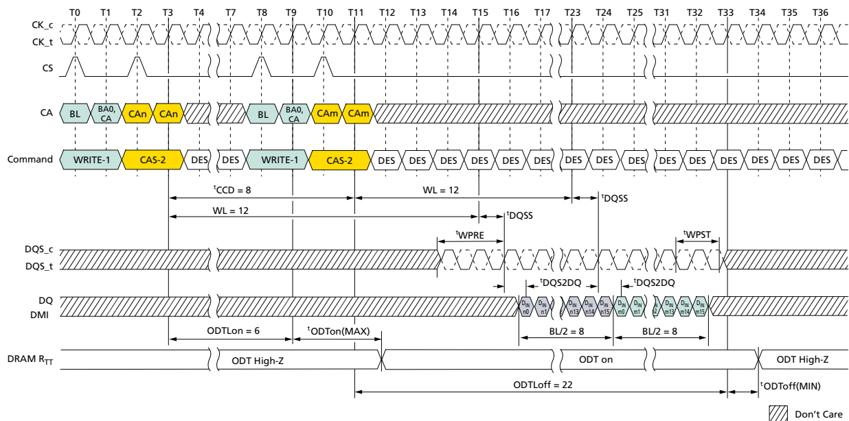
Figure 57: Seamless WRITE: t_{CCD} = \text{MIN} , 1.5nCK Postamble, 533 \text{ MHz} < \text{Clock Frequency} \leq 800 \text{ MHz} , ODT Worst Timing Case
