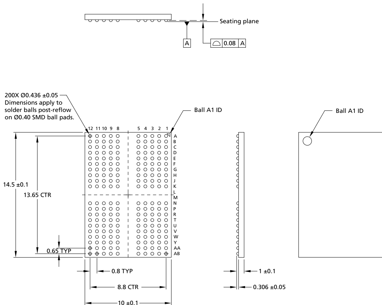
Figure 10: 200-Ball TFBGA – 10mm x 14.5mm x 1.1mm (Package Code: FW)
