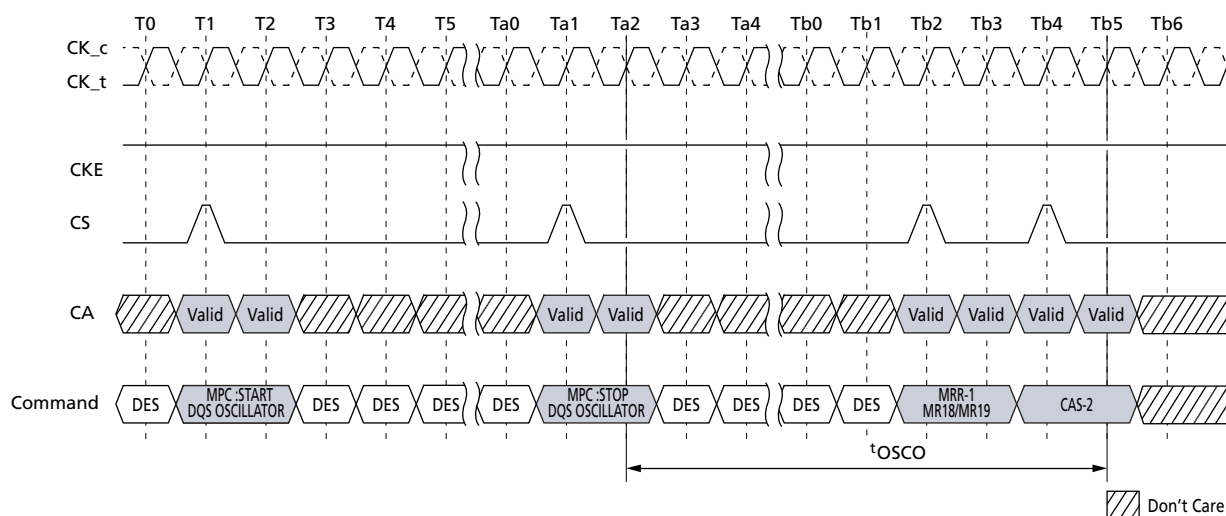
Figure 136: In Case of DQS Interval Oscillator is Stopped by MPC Command
