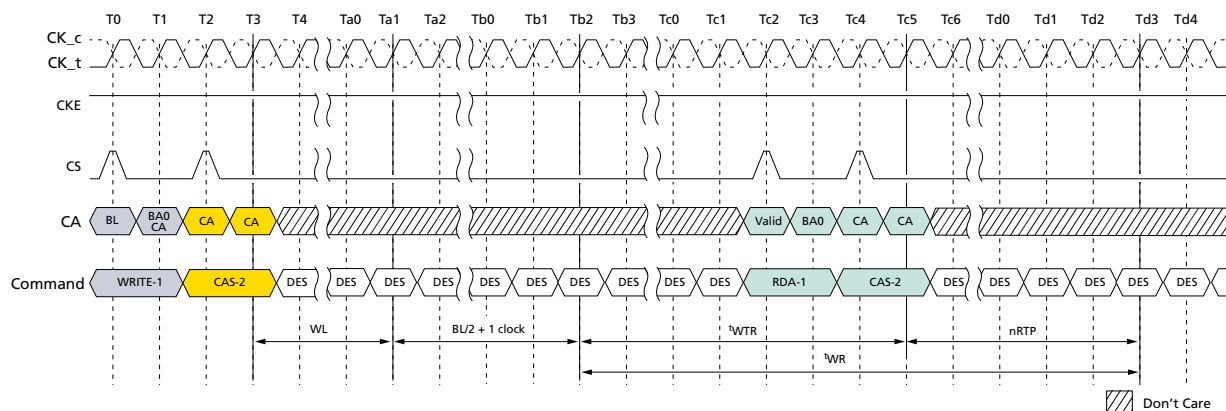
Figure 73: Delay Time From WRITE-to-READ with Auto Precharge
