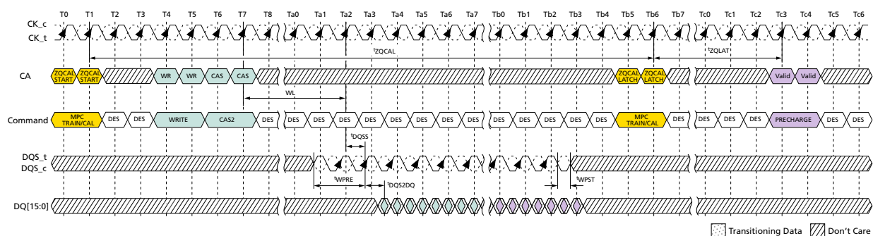
Figure 139: ZQCAL Timing
