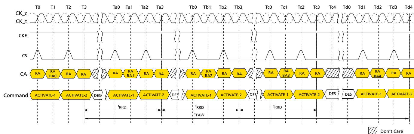
Figure 16: t_{FAW} Timing
