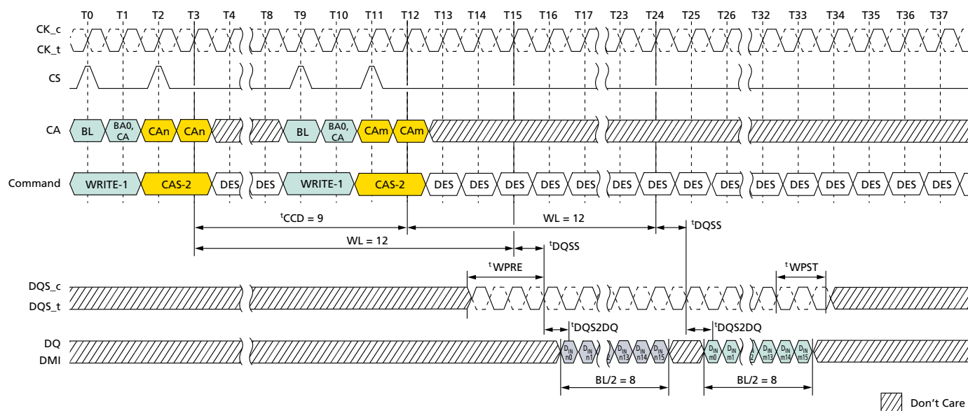
Figure 59: Consecutive WRITE: t_{CCD} = \text{MIN} + 1, 1.5n\text{CK} Postamble
