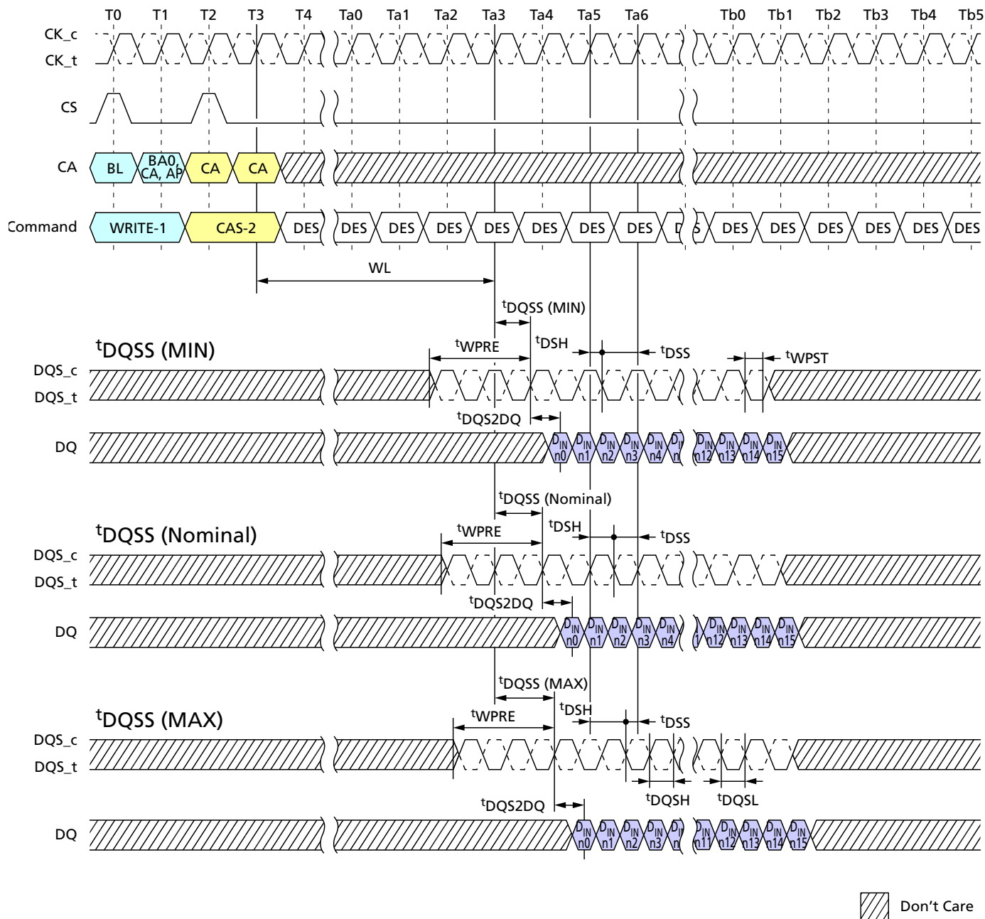
Figure 31: Write Timing
