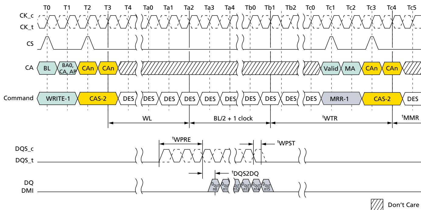
Figure 96: WRITE-to-MRR Timing
