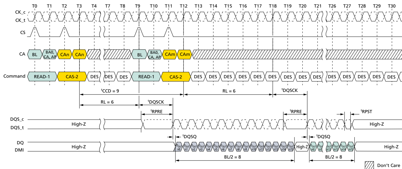
Figure 46: Consecutive READ: t_{CCD} = \text{MIN} + 1 , Preamble = Static, 0.5nCK Postamble
