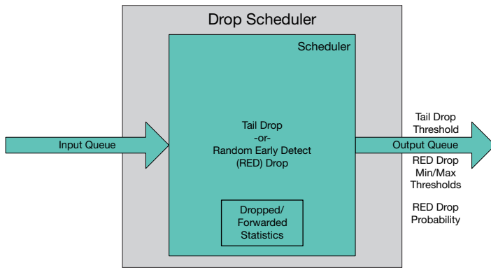
Figure 3: Drop scheduler block diagram
