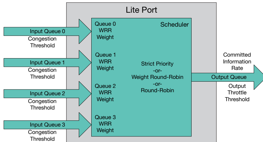
Figure 2: Lite port block diagram
