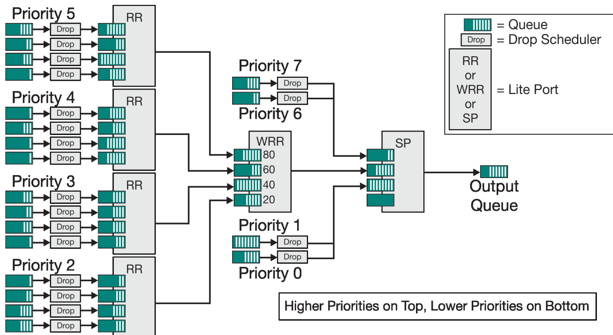
Figure 4: Example QoS hierarchy
