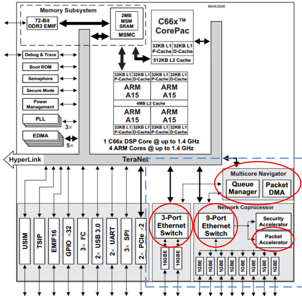
Figure 1: 66AK2E05 SoC block diagram
