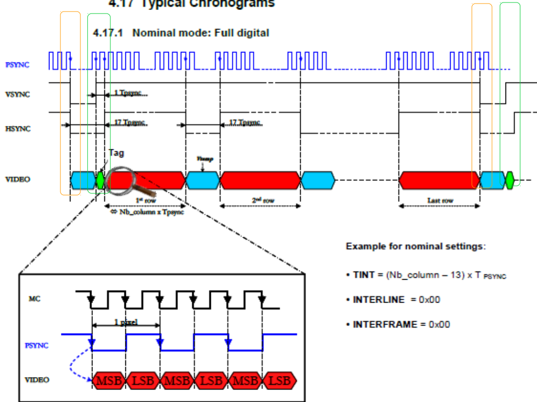
Figure 4.38 – Typical chronogram – Digital video
