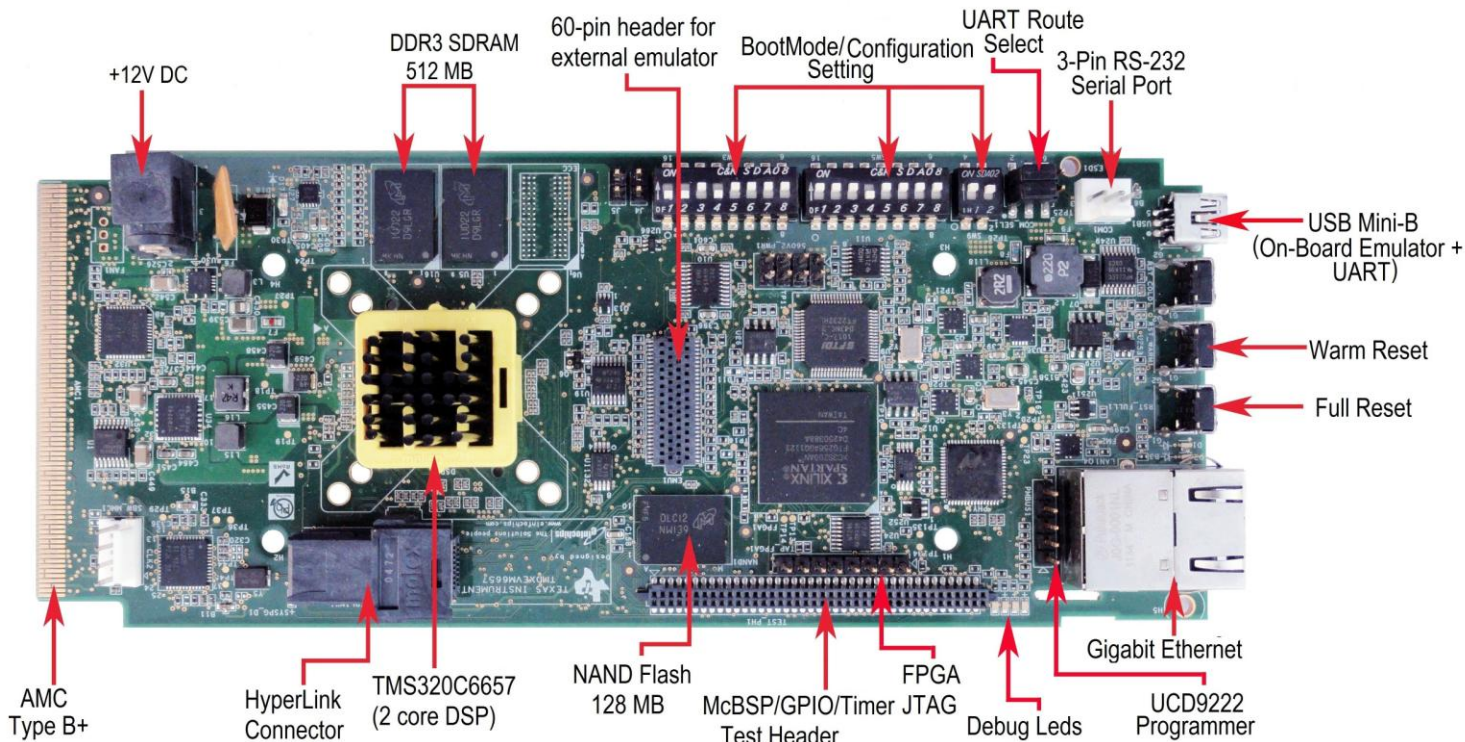
Figure 1.3: TMDXEVM6657L
