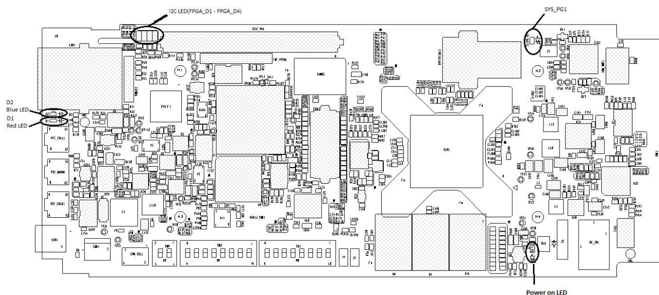
Figure 3.9: Board LEDs
