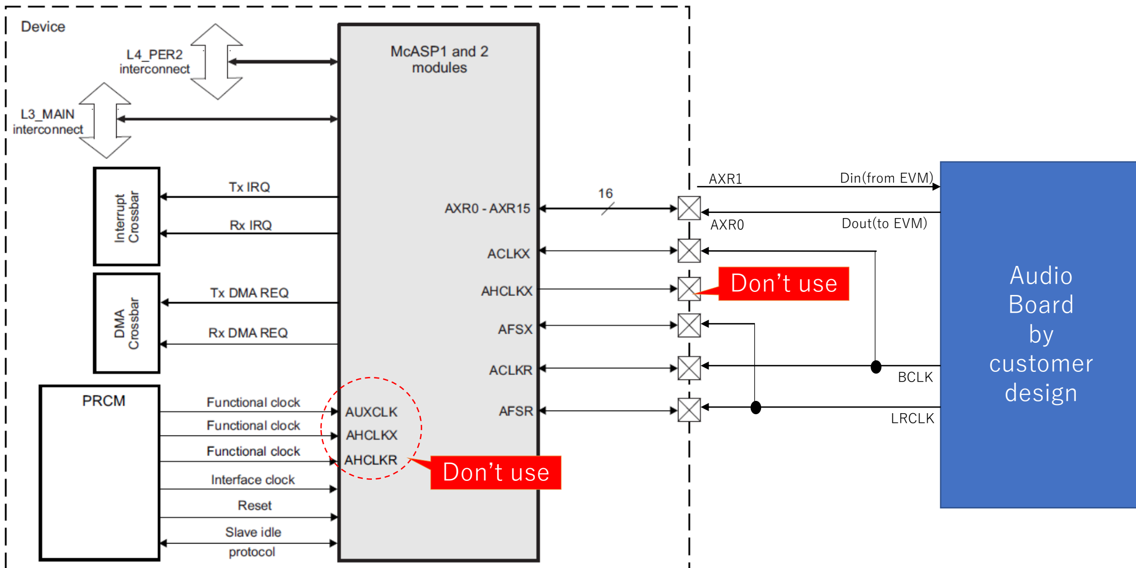
Figure 24-103. McASP Modules Overview
