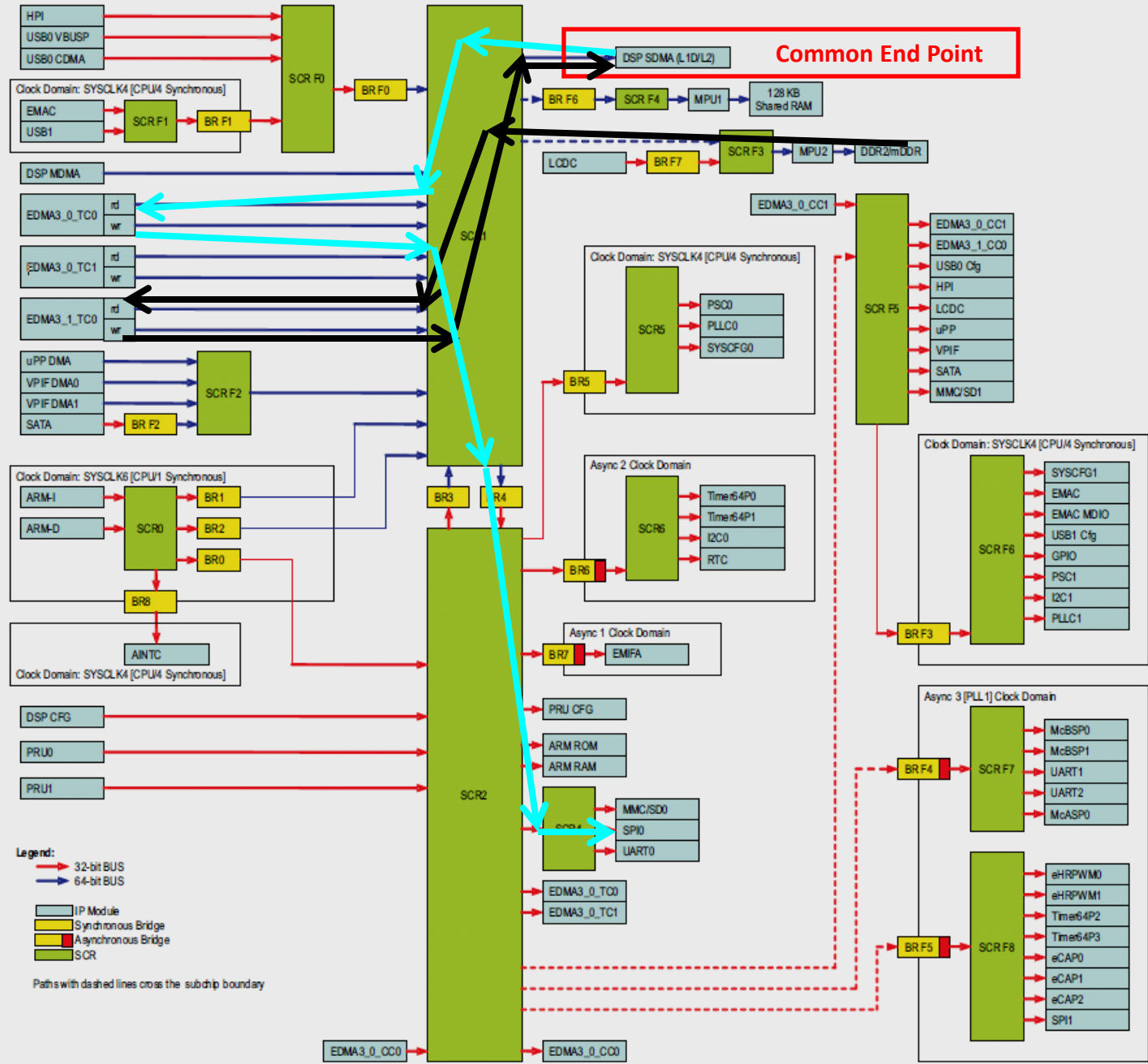
Figure 4-1. System Interconnect Block Diagram
