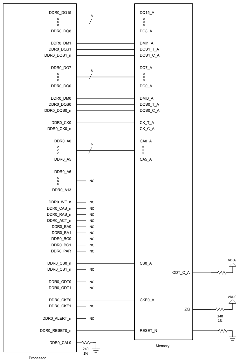
Figure 3-1. 16-Bit, Single-Rank, Single Channel LPDDR4 Implementation
