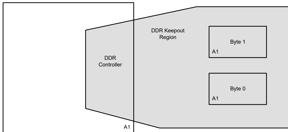
Figure 2-4. DDR4 Keepout Region
