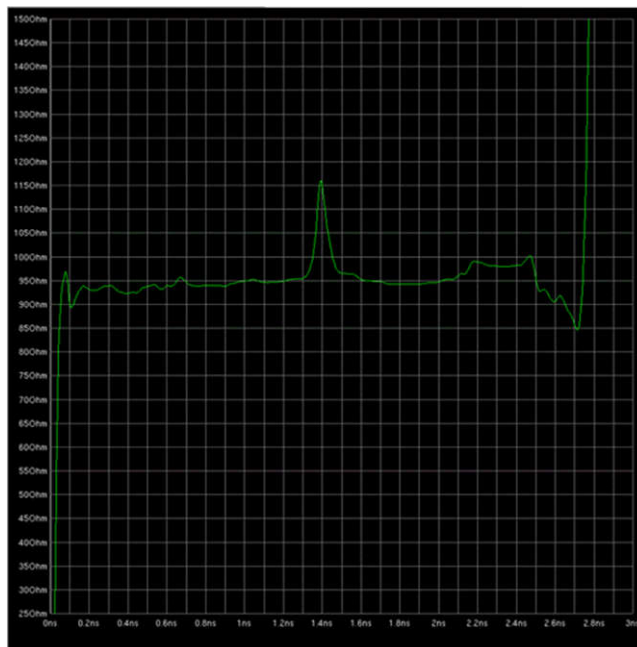
Figure 4-1. TDR Plot Example With Impedance Mismatch
