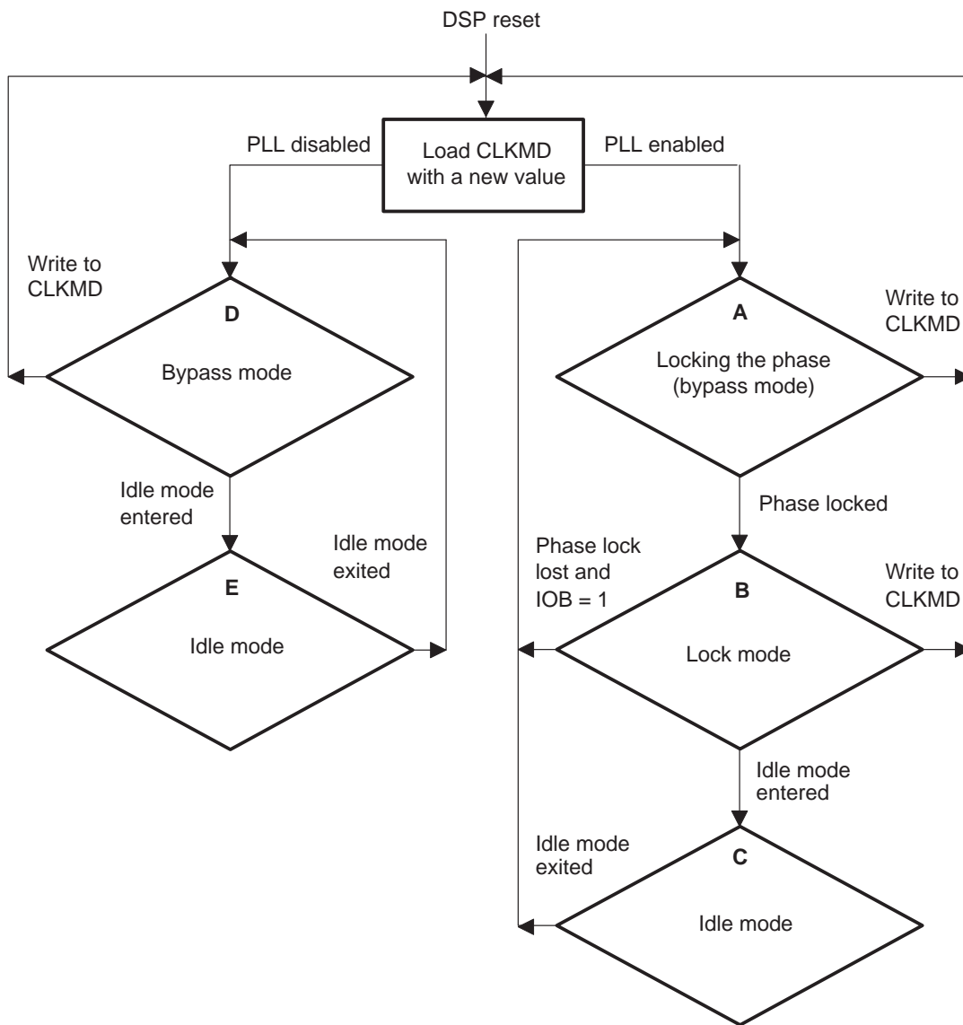
Figure 3–1. Operational Flow of the DSP Clock Generator
