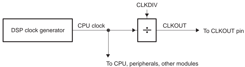
Figure 3–2. Dividing the CPU Clock for the CLKOUT Pin
