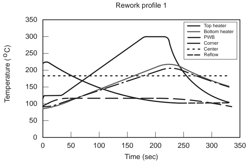
Figure 24. Thermal Reflow Profile
