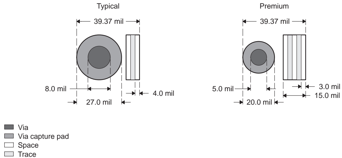
Figure 15. Typical and Premium Via Capture Pad Sizes (in mils)
