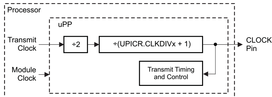
Figure 33-6. Clock Generation for a Channel Configured in Transmit Mode
