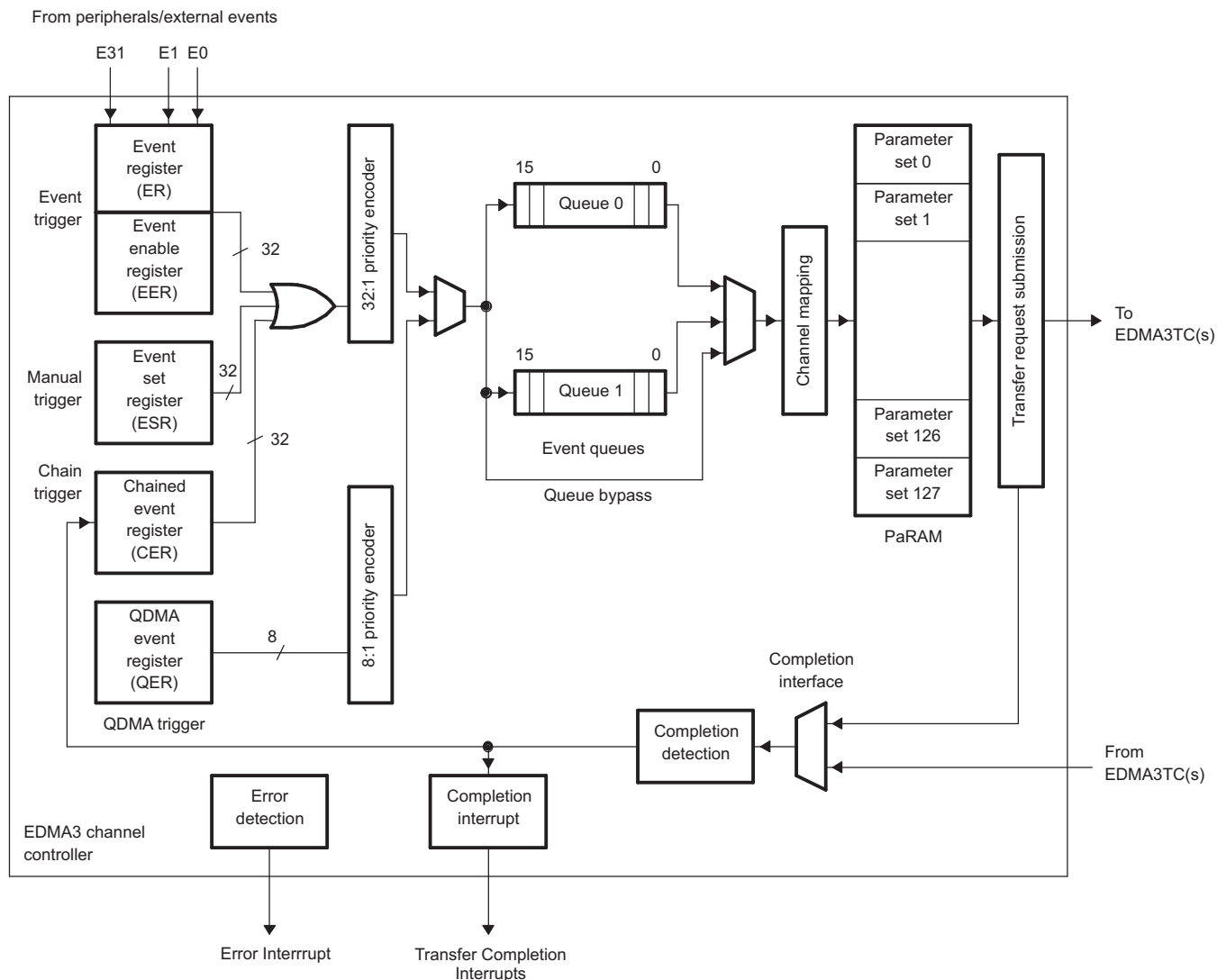
Figure 18-2. EDMA3 Channel Controller (EDMA3CC) Block Diagram
