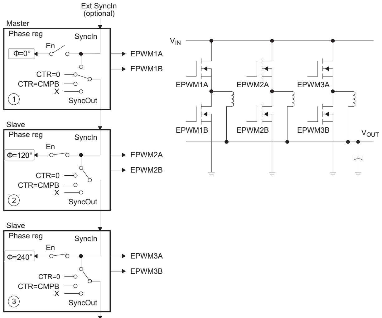
Figure 17-61. Control of a 3-Phase Interleaved DC/DC Converter
