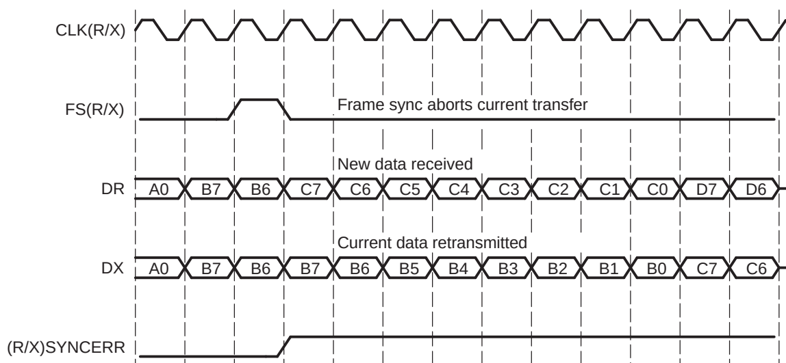
Figure 26-19. Unexpected Frame Synchronization With (R/X)FIG = 0
