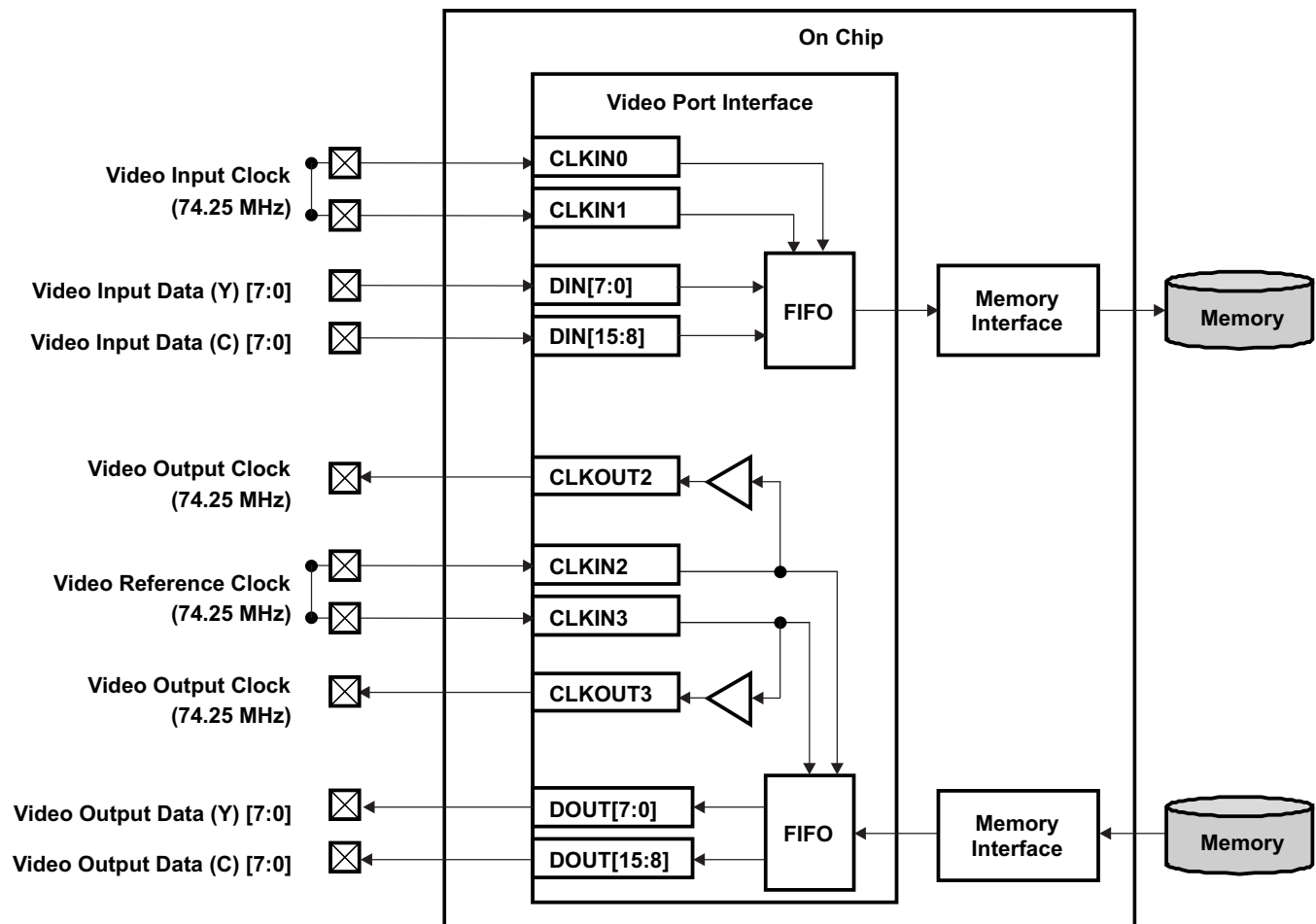
Figure 36-16. Clock Control on Video Input and Output with HDTV Encoding
