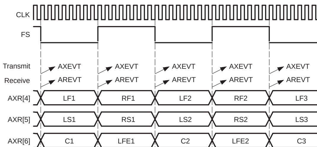
Figure 25-27. DMA Events in an Audio Example—Two Events
