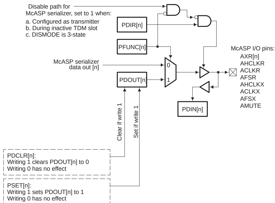
Figure 25-21. McASP I/O Pin Control Block Diagram
