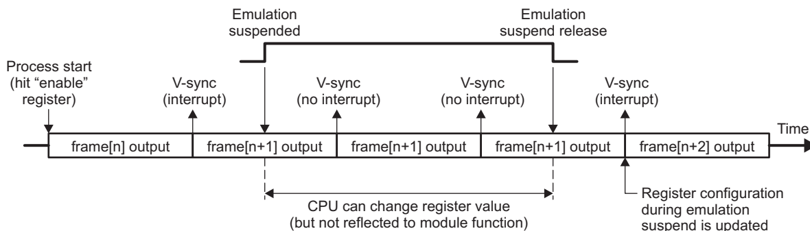
Figure 36-13. Emulation Suspend Function on Channels 2 and 3 (Transmit)
