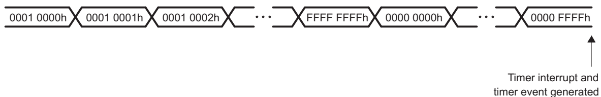
Figure 31-8. 32-Bit Timer Counter Overflow Example
