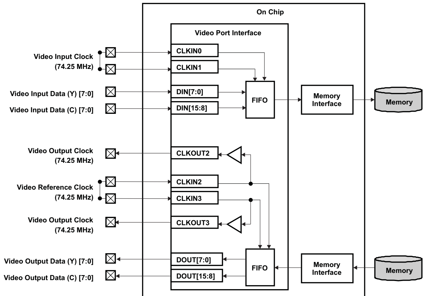
Figure 36-17. Clock Control on Video Input and Output with HDTV Encoding
