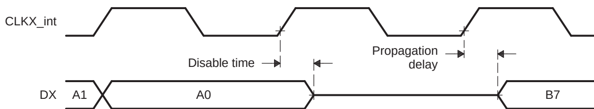
Figure 26-3. Transmit Data Clocking
