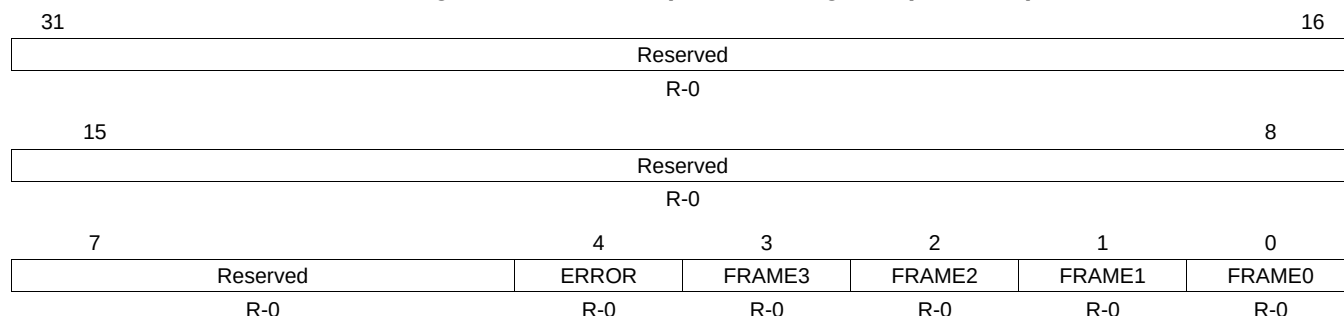
Figure 36-26. Interrupt Status Register (INTSTAT)
