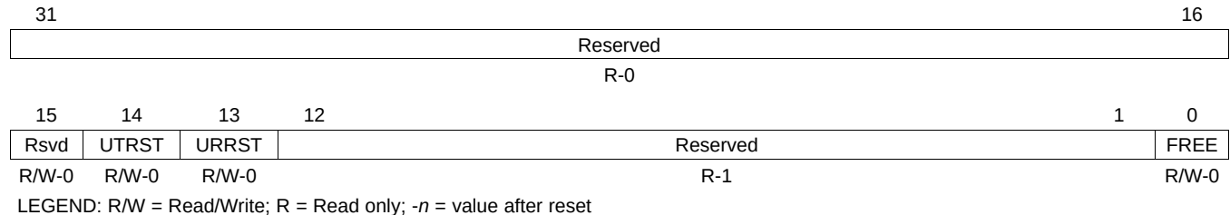
Figure 32-23. Power and Emulation Management Register (PWREMU_MGMT)
