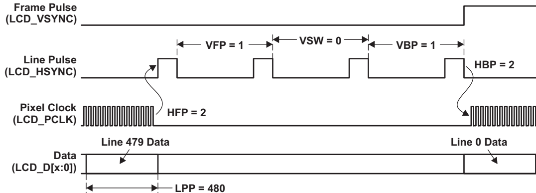
Figure 24-33. Vertical Front Porch (VFP)
