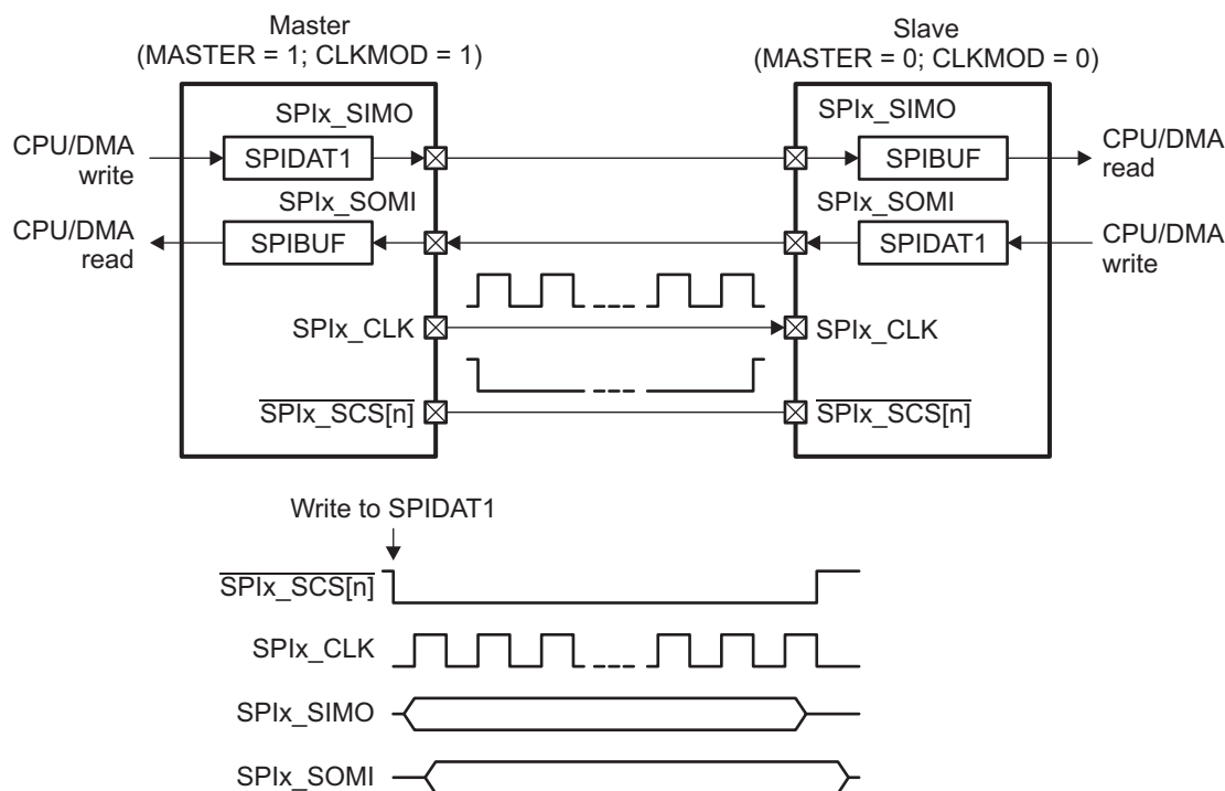
Figure 30-3. SPI 4-Pin Option with \overline{\text{SPIx\_SCS}}[n]
