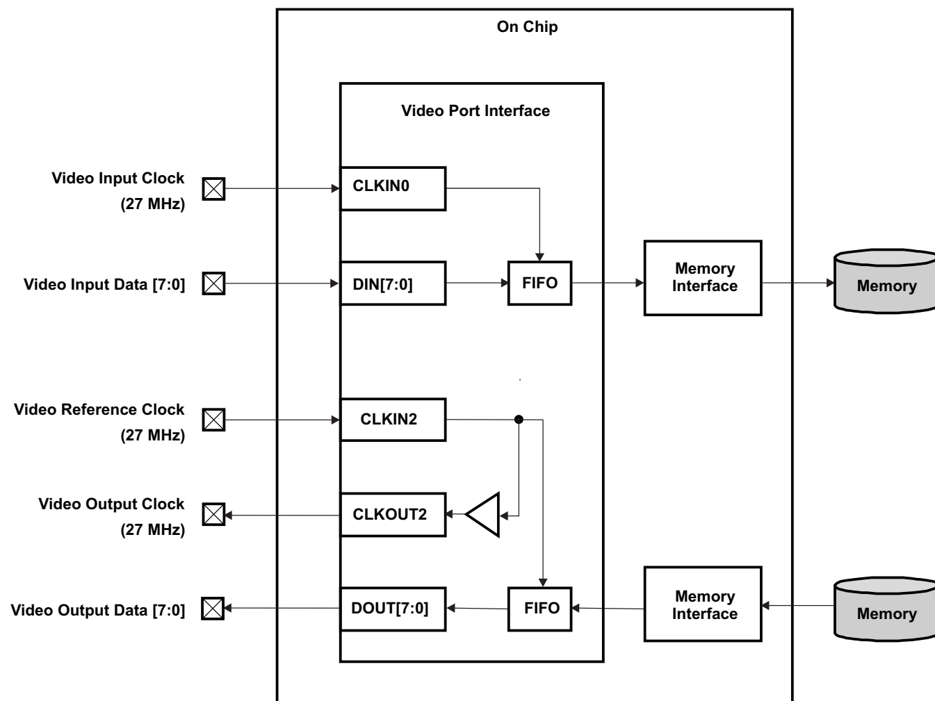
Figure 36-15. Clock Control on Video Input and Output with SDTV Encoding
