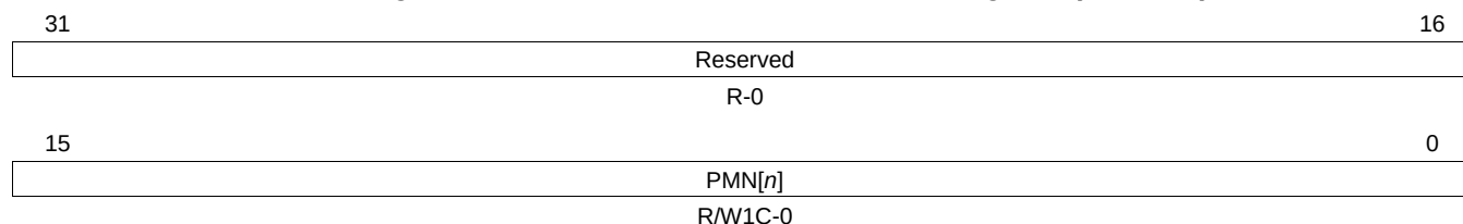
Figure 29-32. Port Serial ATA Notification Register (POSNTF)
