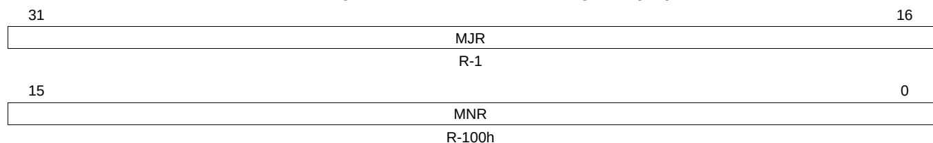
Figure 29-5. AHCI Version Register (VS)
