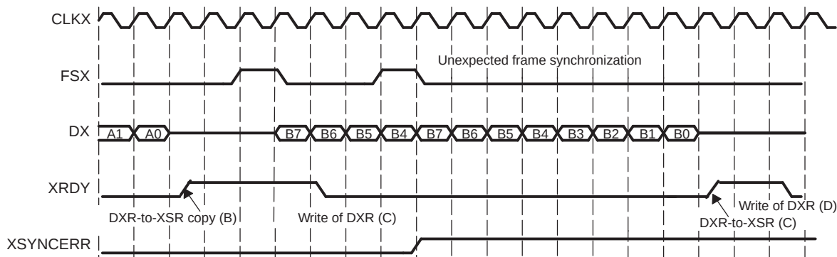
Figure 26-31. Unexpected Transmit Frame Synchronization Pulse
