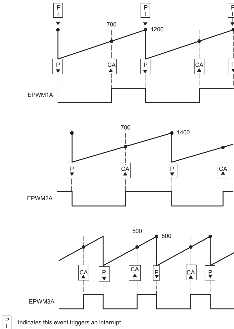
Figure 17-52. Buck Waveforms for Figure 17-51 (Note: Only three bucks shown here)
