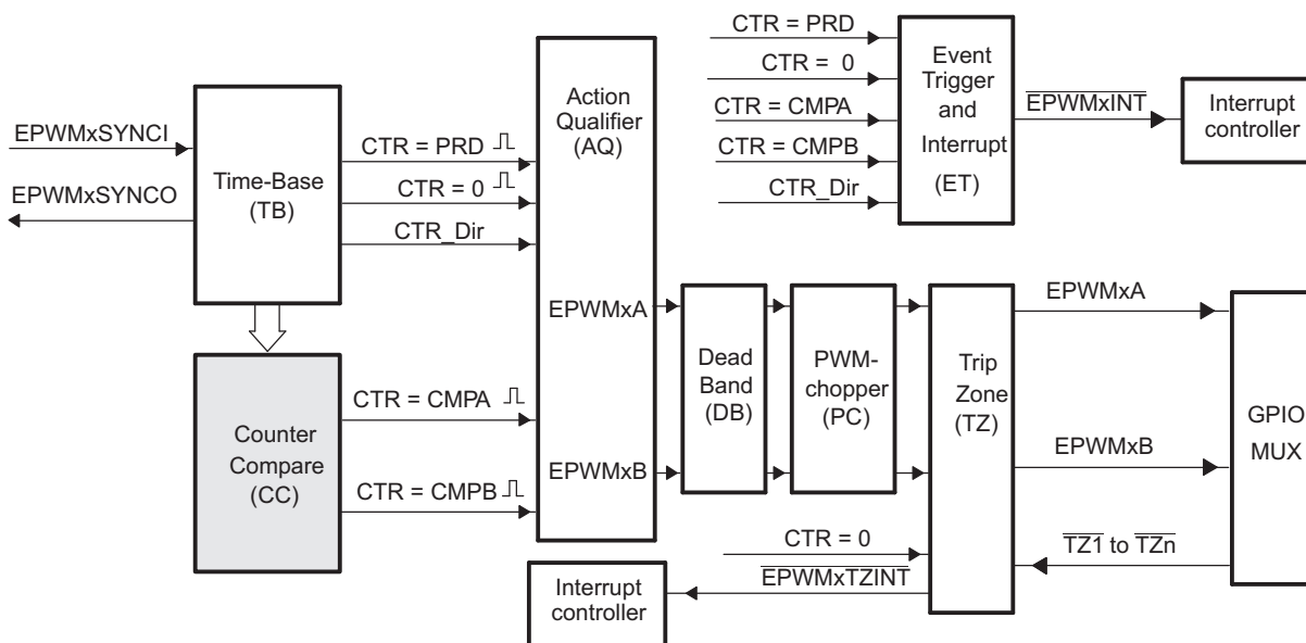
Figure 17-12. Counter-Compare Submodule
