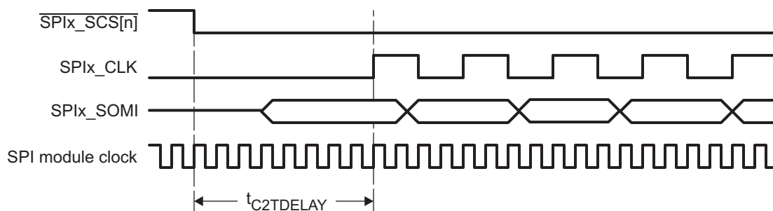
Figure 30-34. Example: t_{\text{C2DELAY}} = 8 SPI Module Clock Cycles
