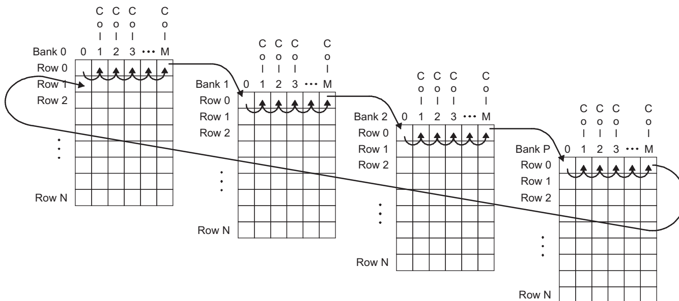
Figure 15-12. DDR2/mDDR SDRAM Column, Row, and Bank Access
