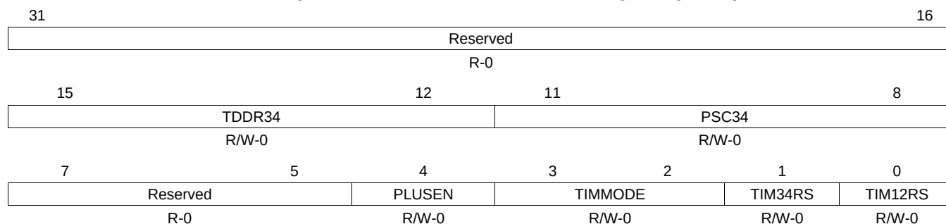
Figure 31-22. Timer Global Control Register (TGCR)
