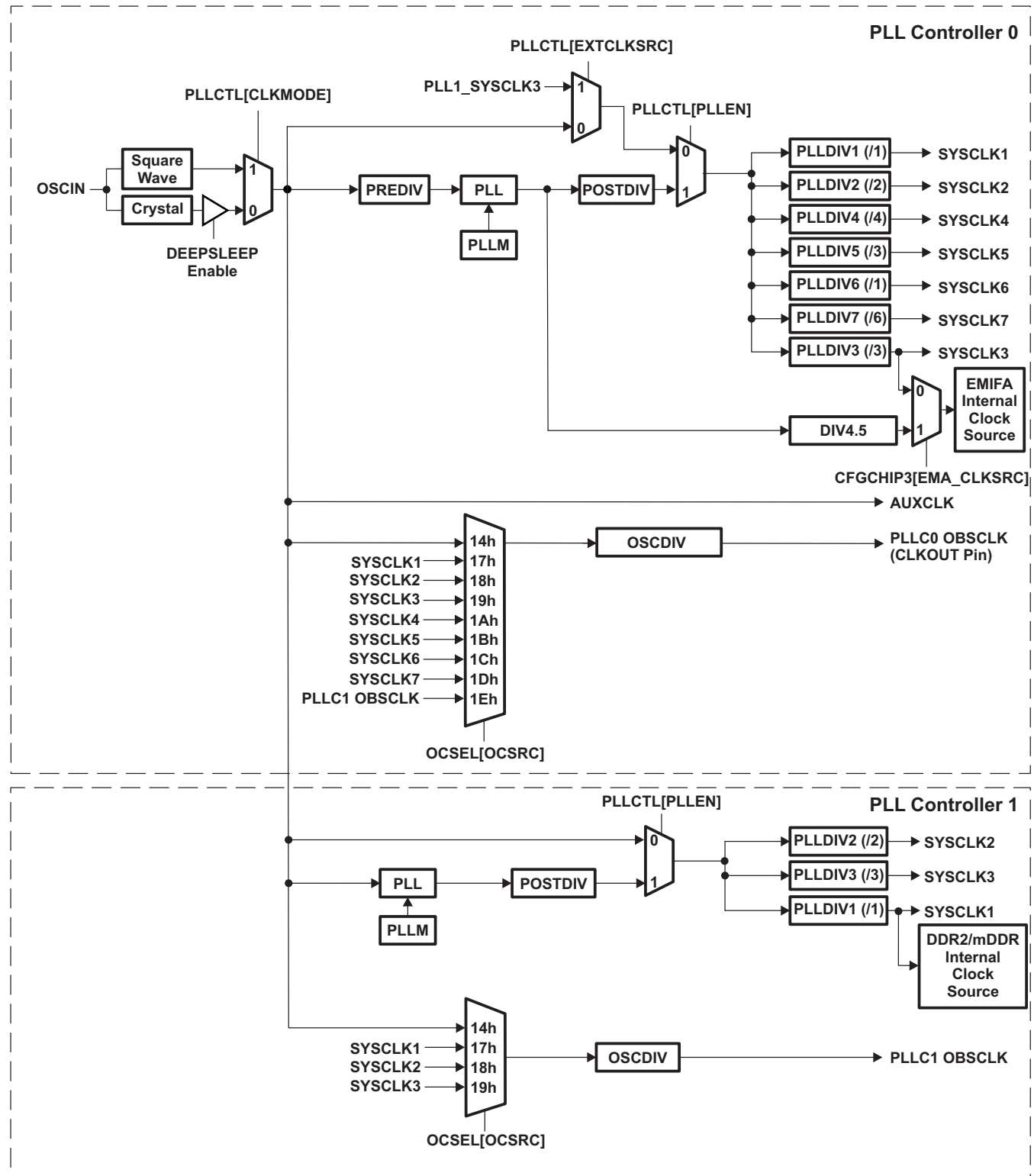
Figure 8-1. PLLC Structure
