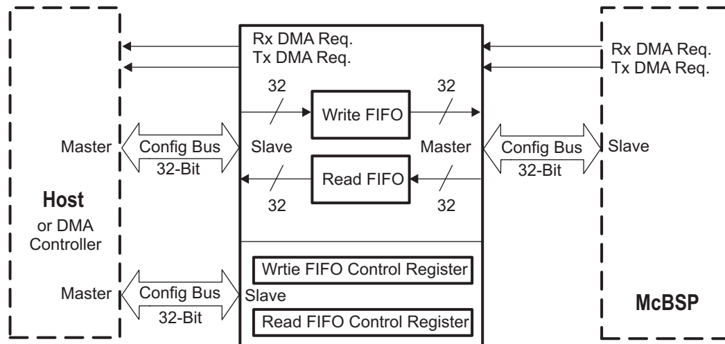
Figure 26-32. McBSP Buffer FIFO (BFIFO) Block Diagram
