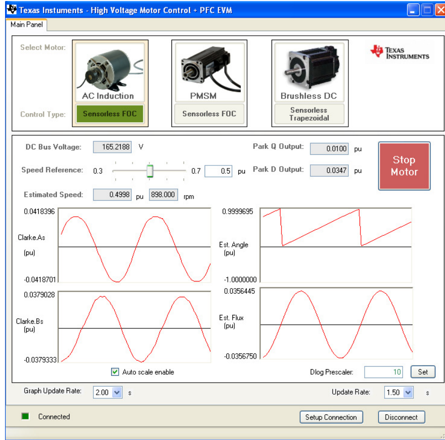
Fig 6: GUI Running ACI Motor
