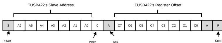
Figure 9. I2C Write Without Data
