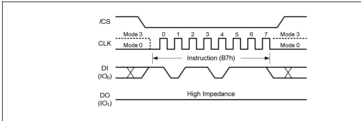
Figure 12. Enter 4-Byte Address Mode instruction
