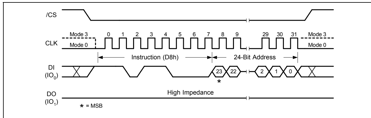
Figure 34. 64KB Block Erase Instruction 32-Bit Address is required when the device is operating in 4-Byte Address Mode
