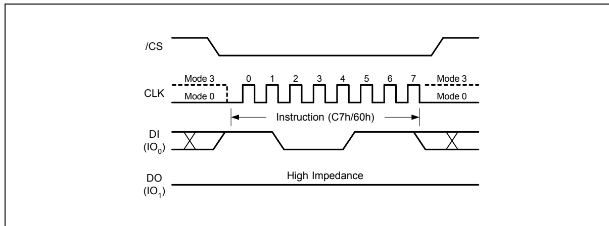
Figure 36. Chip Erase Instruction Sequence Diagram
