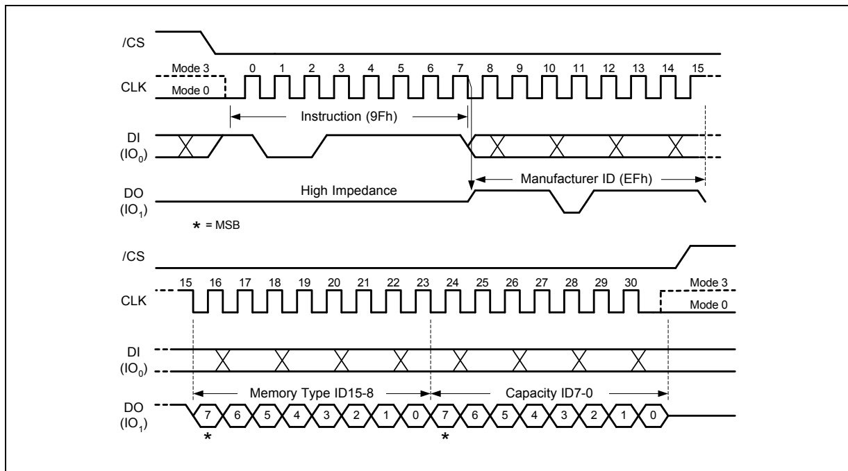
Figure 45. Read JEDEC ID Instruction
