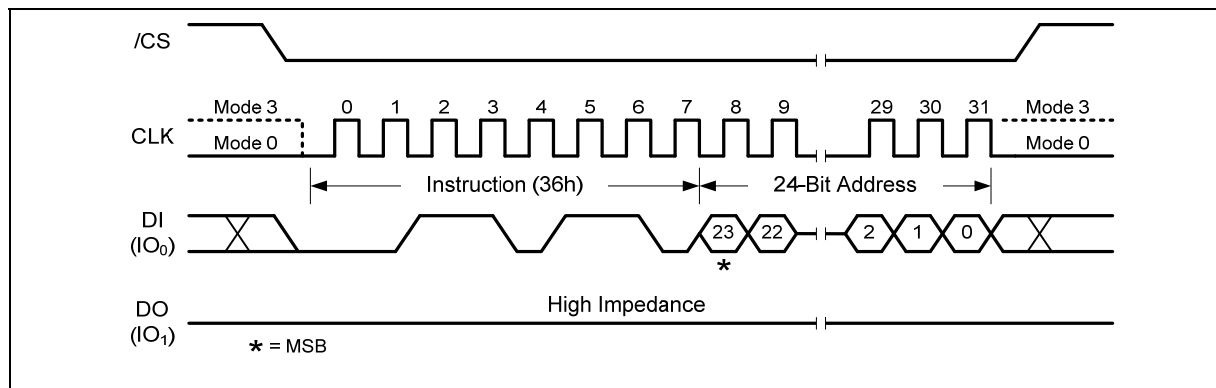
Figure 50. Individual Block/Sector Lock Instruction
