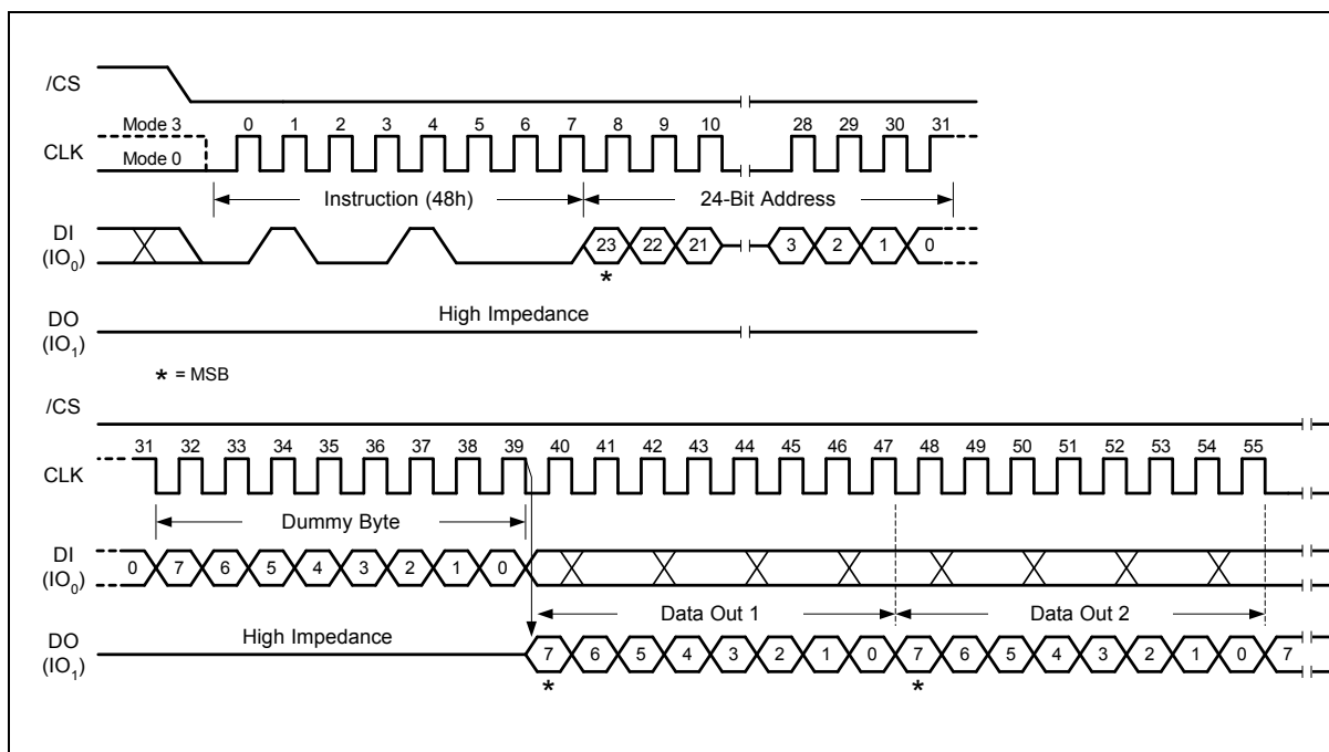
Figure 49. Read Security Registers Instruction 32-Bit Address is required when the device is operating in 4-Byte Address Mode
