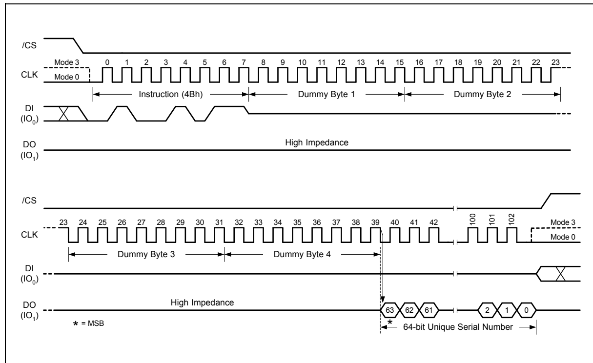
Figure 44. Read Unique ID Number Instruction
