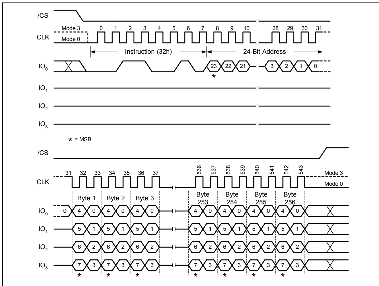
Figure 29. Quad Input Page Program Instruction 32-Bit Address is required when the device is operating in 4-Byte Address Mode
