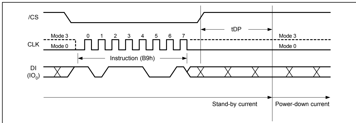
Figure 39. Deep Power-down Instruction
