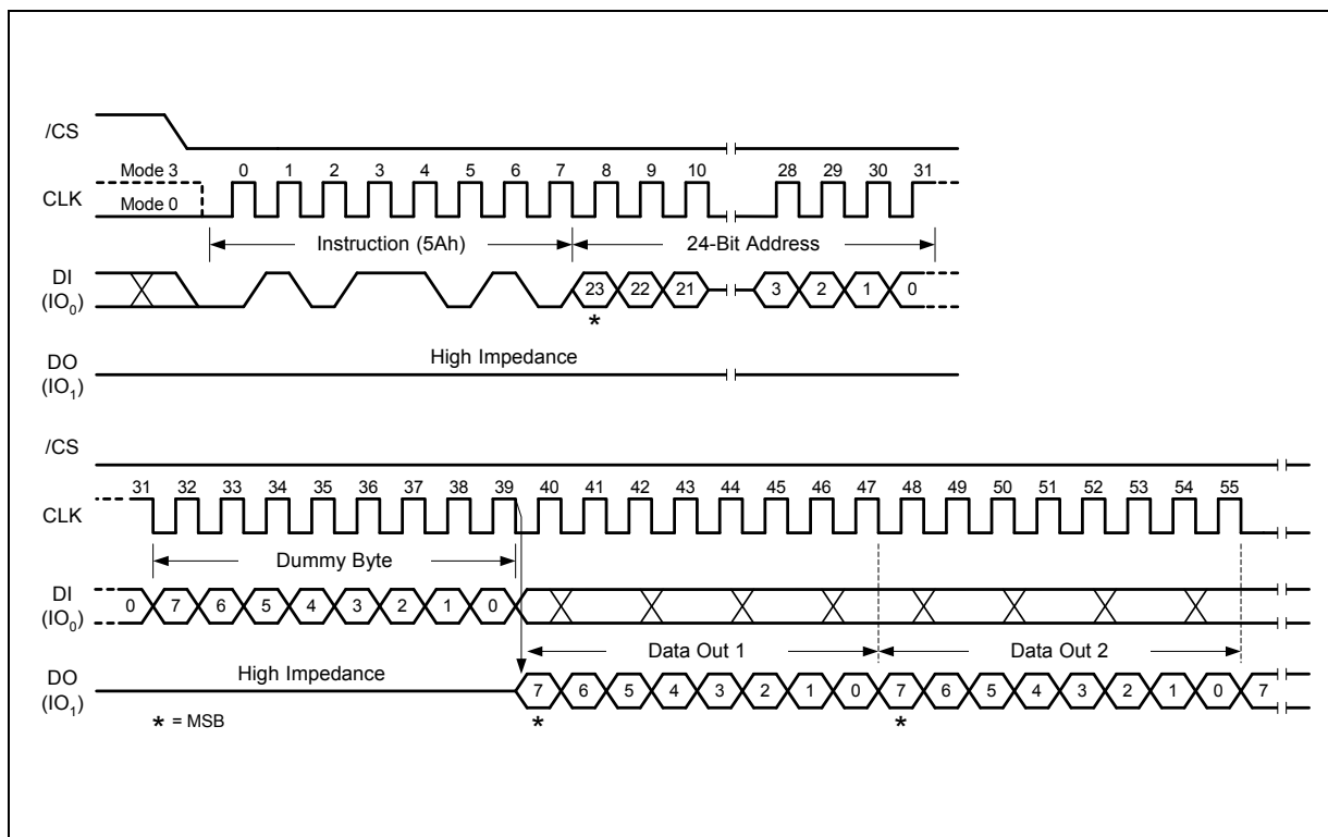
Figure 46. Read SFDP Register Instruction Sequence Diagram
