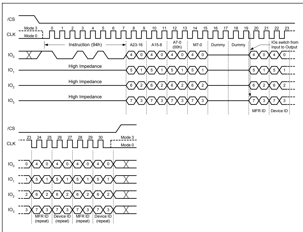
Figure 43. Read Manufacturer / Device ID Quad I/O Instruction
