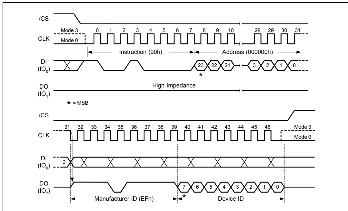
Figure 41. Read Manufacturer / Device ID Instruction
