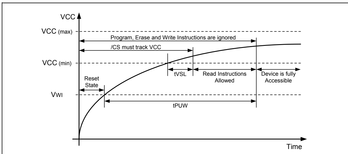
Figure 56a. Power-up Timing and Voltage Levels
