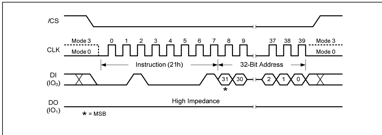
Figure 32. Sector Erase with 4-Byte Address Instruction
