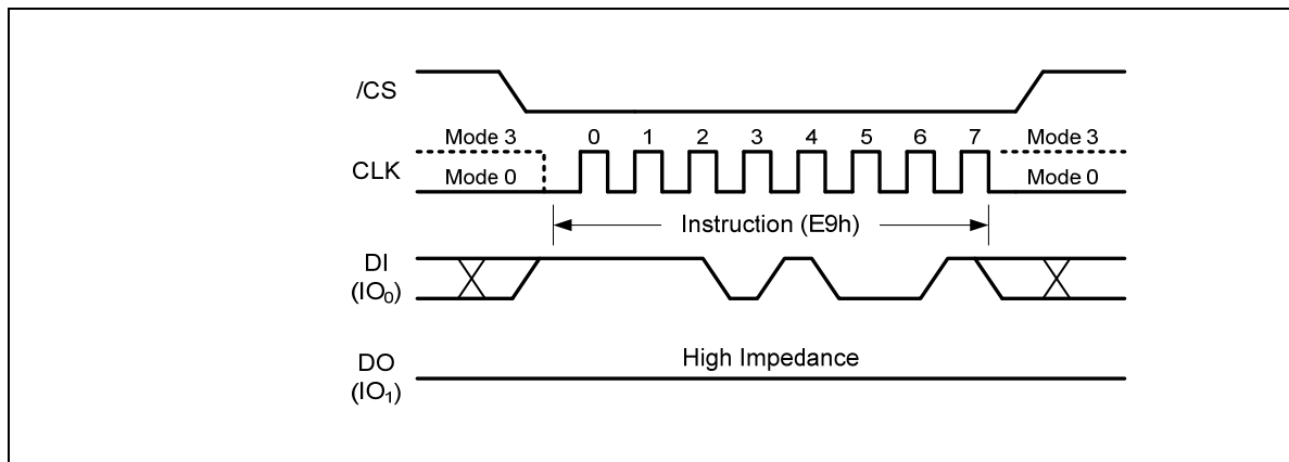
Figure 13. Exit 4-Byte Address Mode instruction
