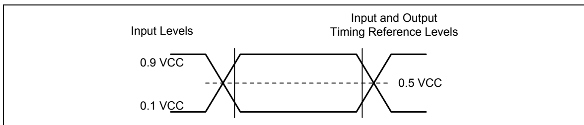
Figure 57. AC Measurement I/O Waveform
