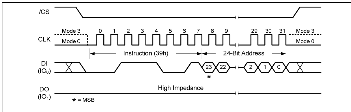
Figure 51. Individual Block Unlock Instruction
