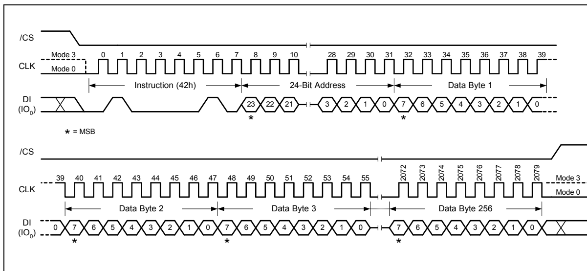
Figure 48. Program Security Registers Instruction 32-Bit Address is required when the device is operating in 4-Byte Address Mode
