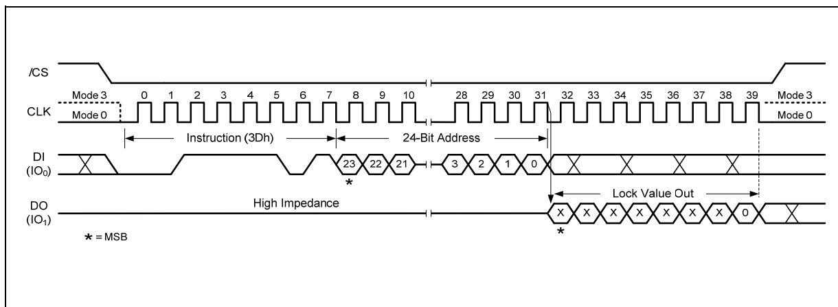
Figure 52. Read Block Lock Instruction 32-Bit Address is required when the device is operating in 4-Byte Address Mode
