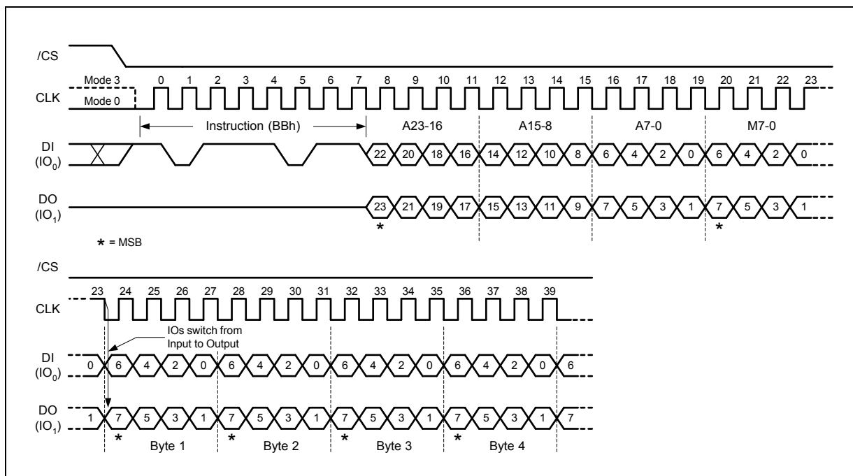
Figure 22. Fast Read Dual I/O (M7-M0 should be set to Fxh) 32-Bit Address is required when the device is operating in 4-Byte Address Mode
