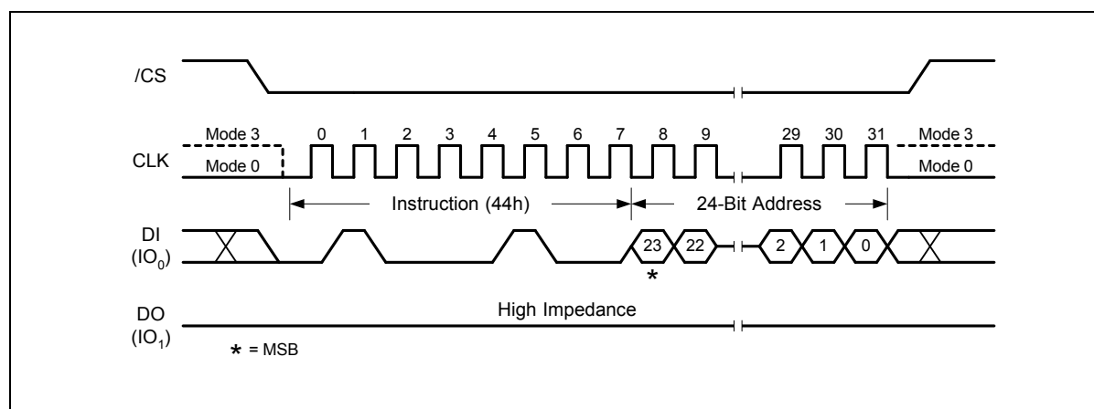
Figure 47. Erase Security Registers Instruction 32-Bit Address is required when the device is operating in 4-Byte Address Mode
