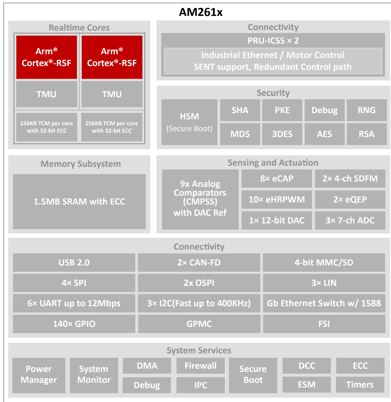
Figure 3-1. AM261x Functional Block Diagram
