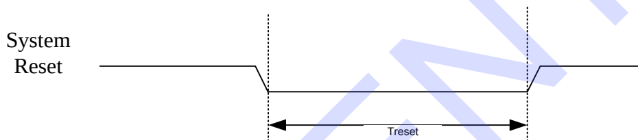
Figure 7-5. Power-Up Timing
