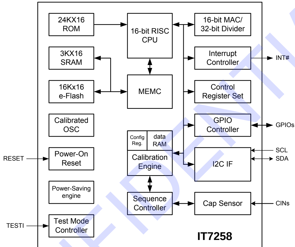
Figure 3-1. Block Diagram
