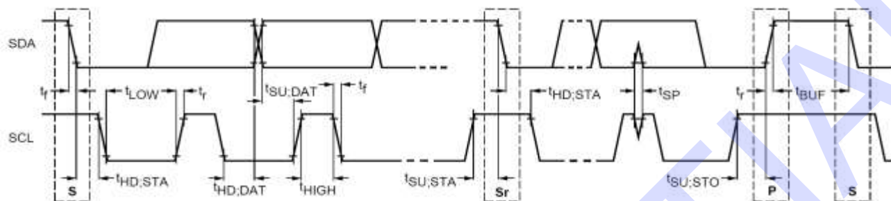
Figure 9-1. Definition of Timing for I 2 C Interface
