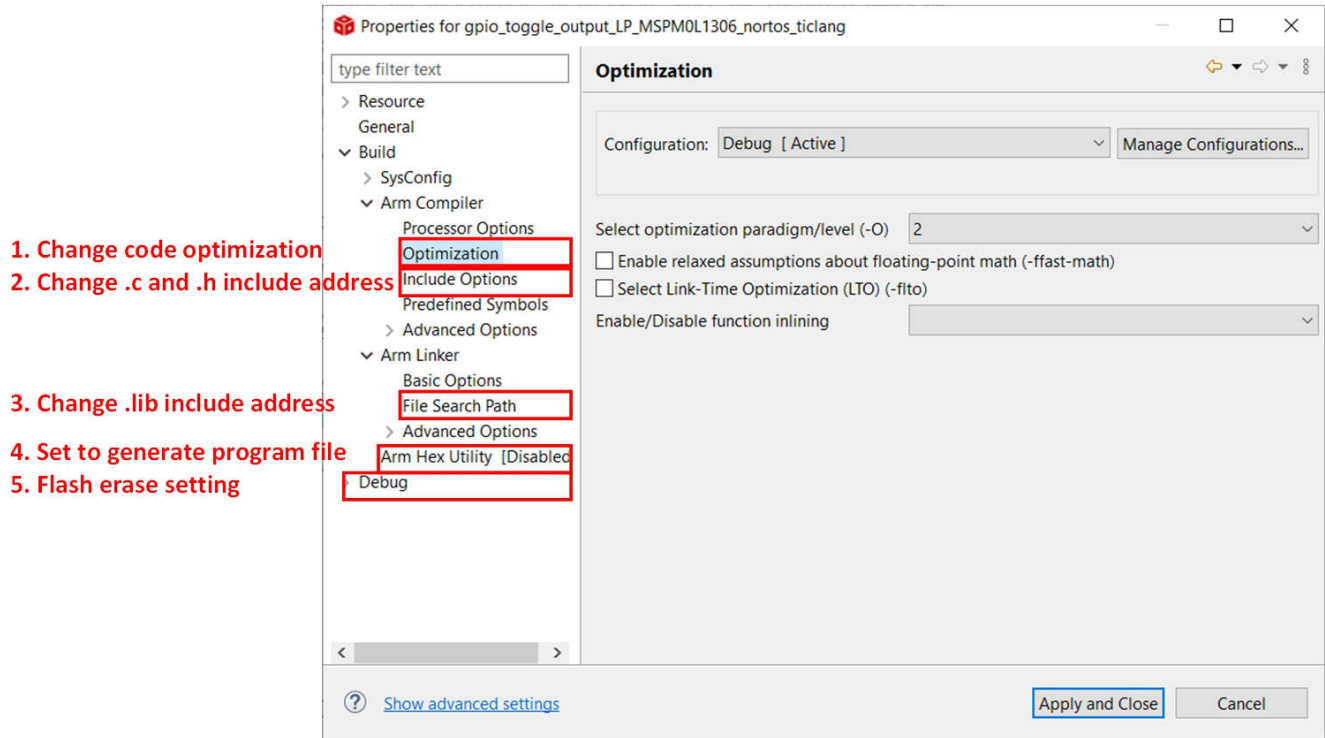
Figure A-9. Common Used Project Settings
