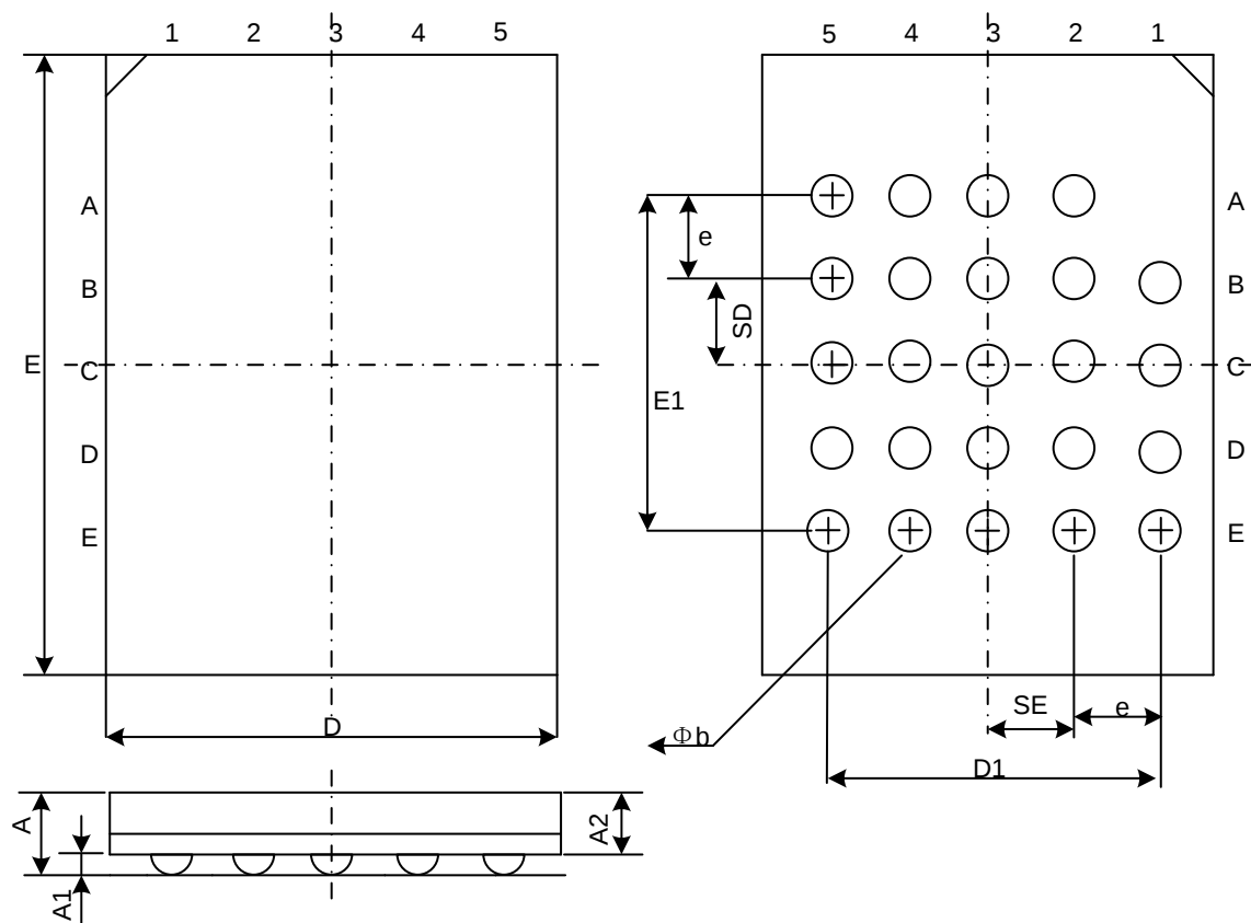
Figure 20-2. TFBGA-24 6x8 BALL (5*5-1 ball array)
